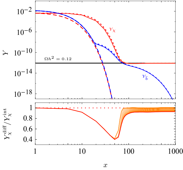
FIG. 7. Upper panel: Evolution for the resulting abundance of \tilde{b} (blue) and \chi (red) of the differential (solid) and integrated (dotted) Boltzmann equation. The dashed curves denote the equilibrium abundances. Lower panel: Ratio of the two abundances for \chi . The red solid line shows the converged result while the orange thick and thin curves denote the first and the following iterations, respectively. Only the decay term is considered.
