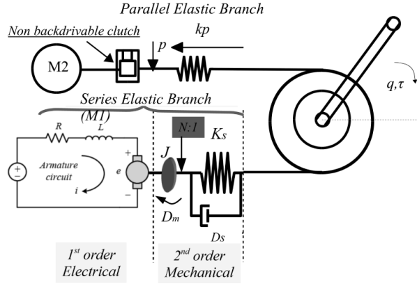
Figure 4. The series and parallel branch of a compliant actuator of the COMAN.
