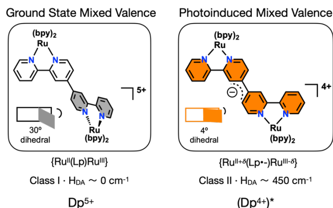
Figure 1. Structure of the ground state mixed valence and photoinduced mixed valence states of Dp^{n+} complexes studied herein, as well as their electronic configuration and their classification according to Robin and Day.
