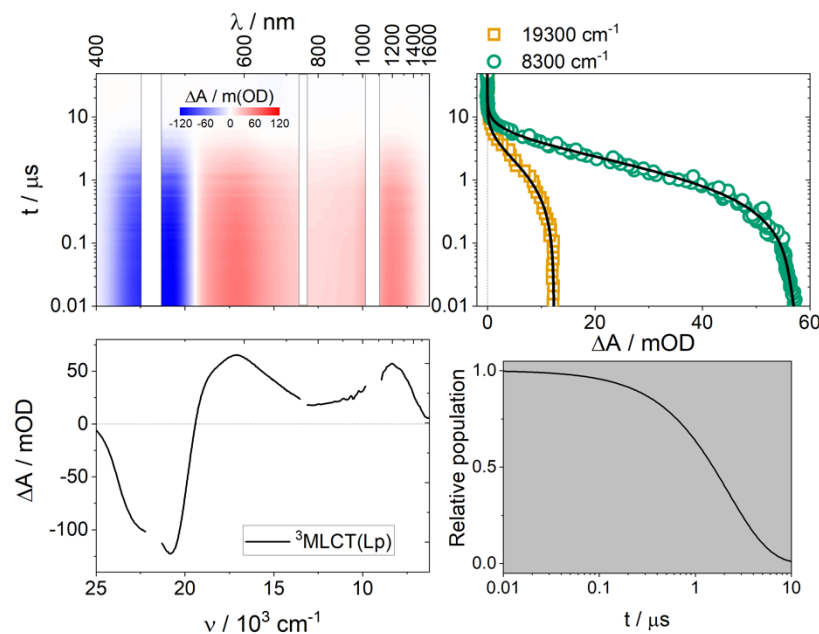
Figure 3. Top left: Differential absorption 3D map obtained from nsTAS for \text{Dp}^{4+} in ACN upon 460 nm ( 21700 \text{ cm}^{-1} ) excitation. Top right: Time absorption profile and corresponding fit at 8300 \text{ cm}^{-1} and 19300 \text{ cm}^{-1} . Bottom left: Species associated differential spectrum of the {}^3\text{MLCT(Lp)} excited state. Bottom right: Concentration evolution over time.
