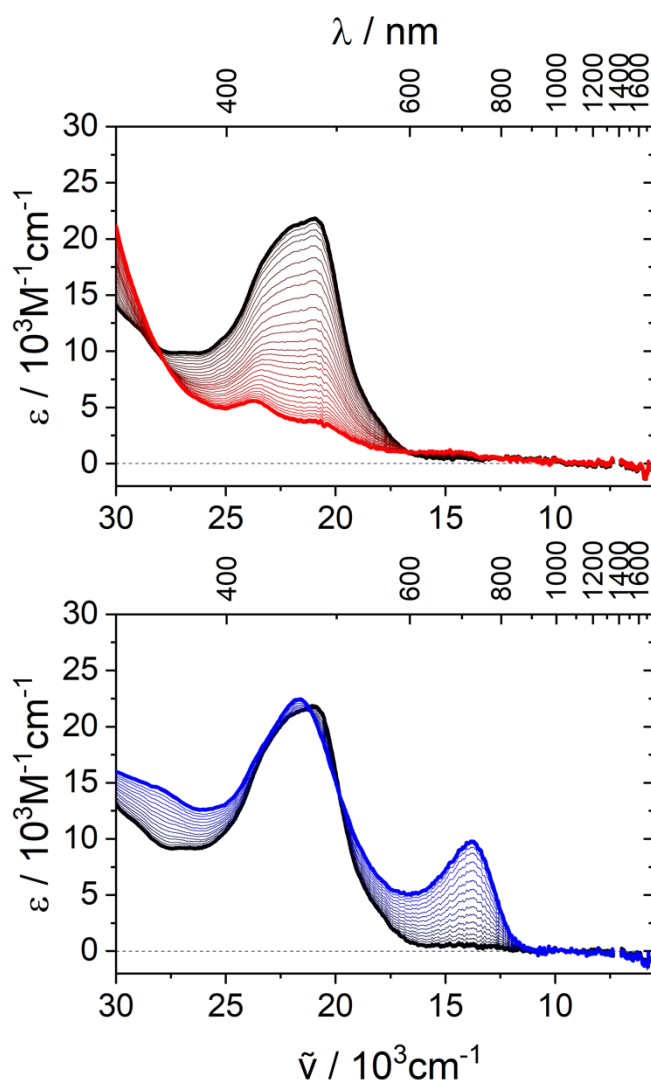
Figure 2. Spectroelectrochemical measurements recorded during the two-electron oxidation (top, potential scans from +1.2 to +1.5 V vs. Ag/AgCl) and one-electron reduction (bottom, potential scans from -0.8 to -1.15 V vs. Ag/AgCl) of Dp^{4+} in 0.1 M TBAPF 6 ACN electrolyte. Initial spectra (black) correspond to Dp^{4+} and the final spectra to Dp^{6+} (red) and Dp^{3+} (blue).
