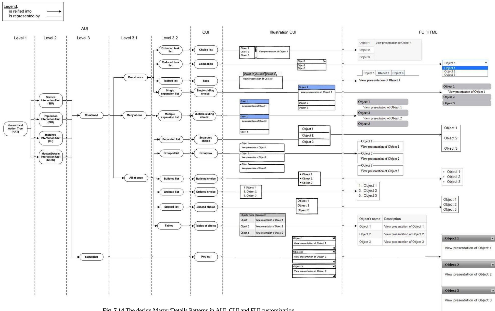
Fig. 7.14 The design Master/Details Patterns in AUI, CUI and FUI customization
