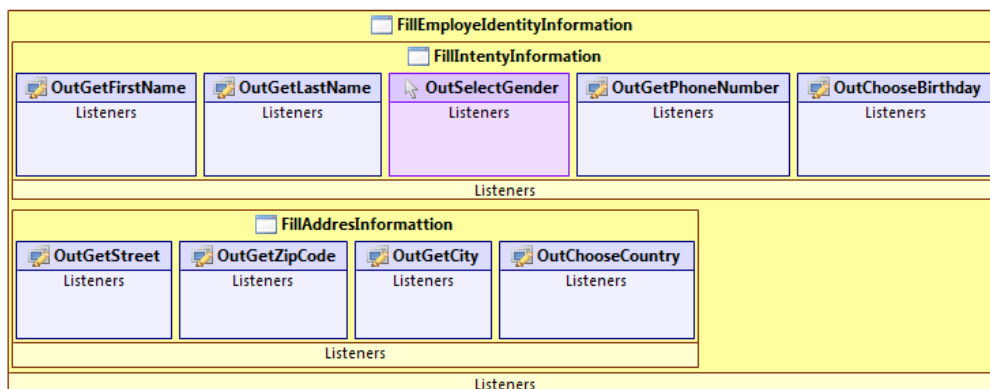
Fig. 7.12 The Master-Detail Pattern leading to a AUI model
