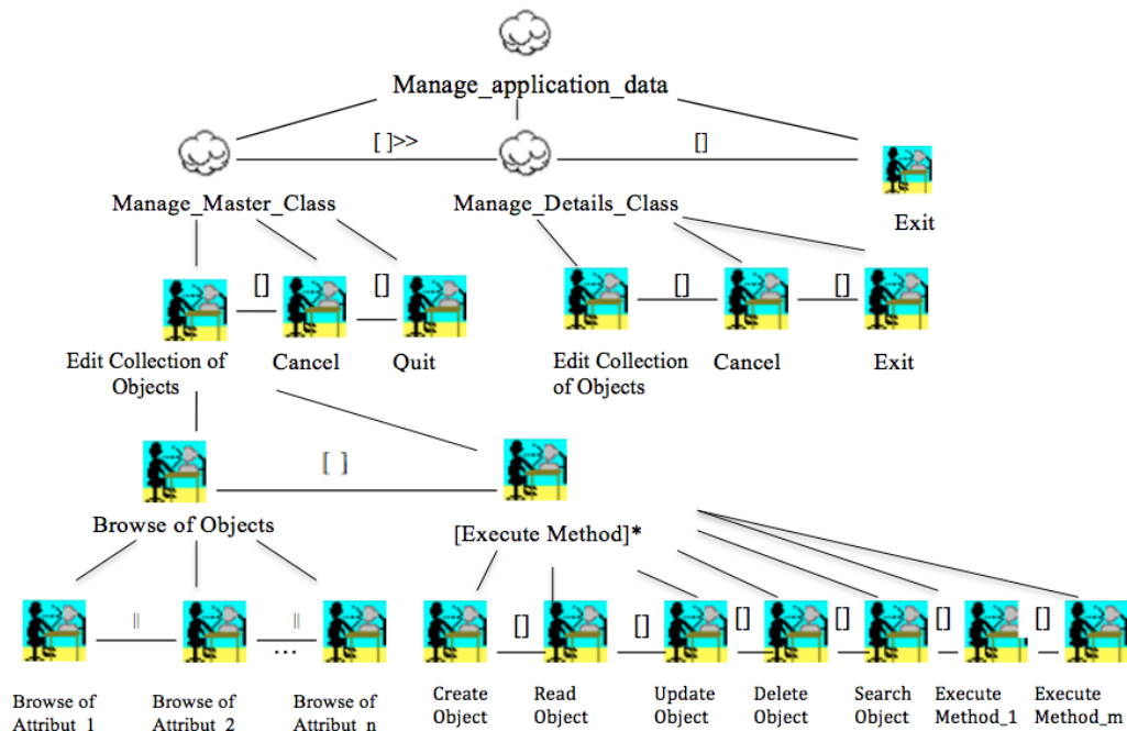
Fig. 7.9 Master-Detail pattern defined by an aggregation relationship
