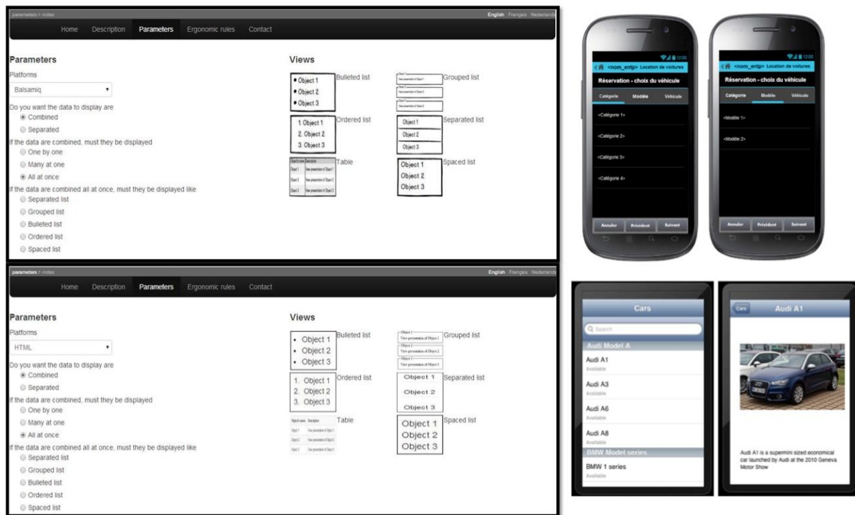
Fig. 7.19 A tool of guidance for M/D pattern implementation with Balsamiq FUI model (left above), with HTML FUI model (left below), final CUI model (right above), FUI model (right below)
