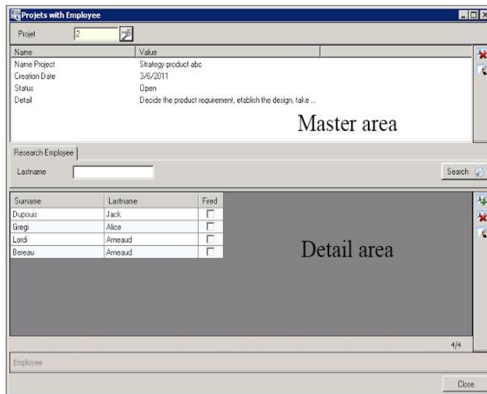
Fig. 7.4 Master-Detail pattern for desktop platforms: (a)Microsoft Windows and (b) MacOS (PJMolina 2013)
