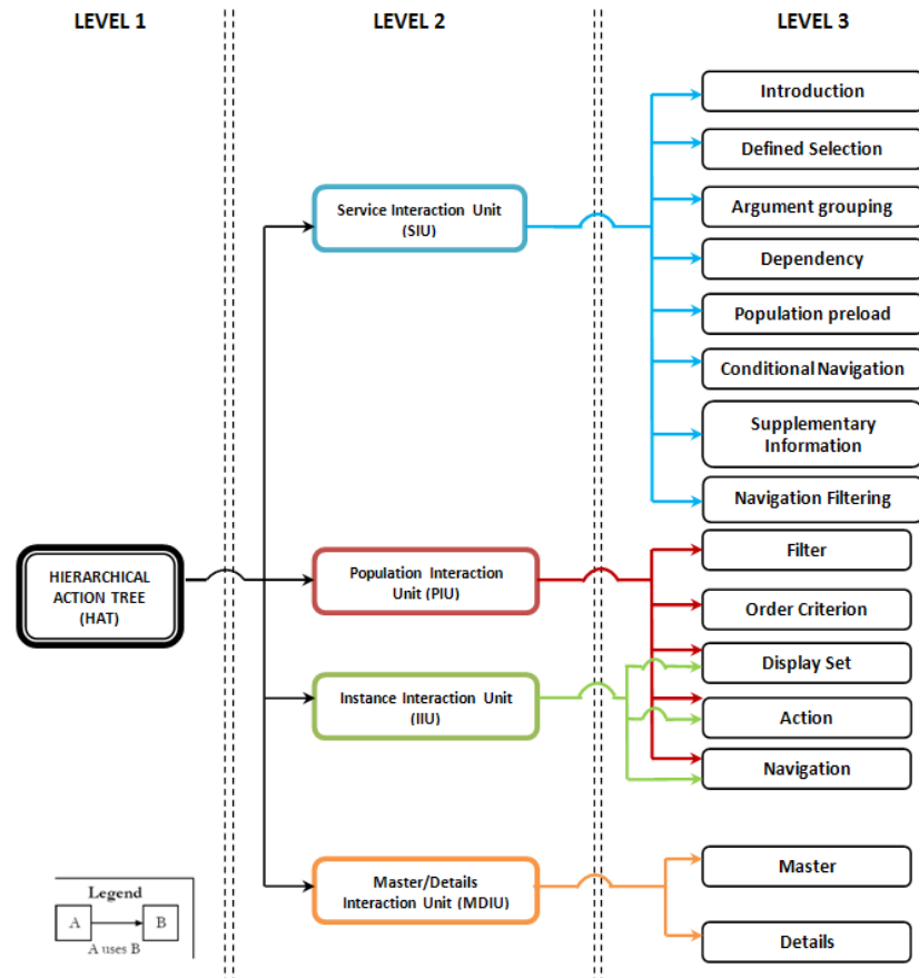
Fig. 7.2 The Presentation Model of OO-Method (Aquino and al. 2010)
