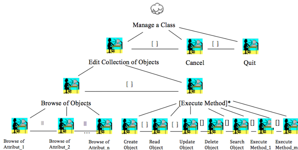
Fig. 7.8 Master-Detail pattern defined by a unity class
