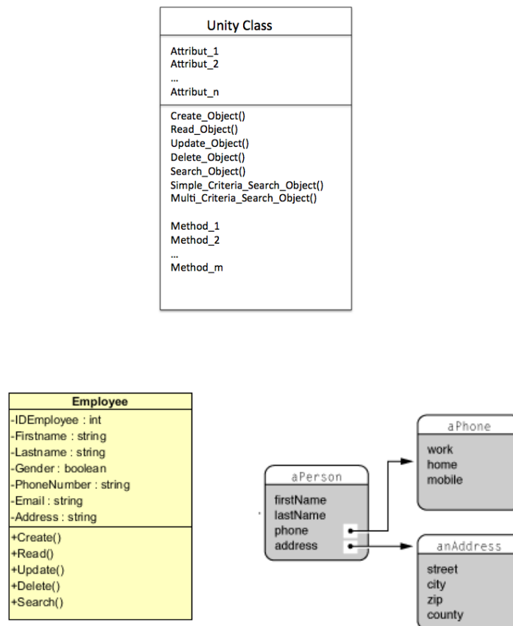
Fig. 7.10 A domain model associated to the Master-Detail pattern (a) and associated to the System Environment (Mac Developer Library 2012) (b)
