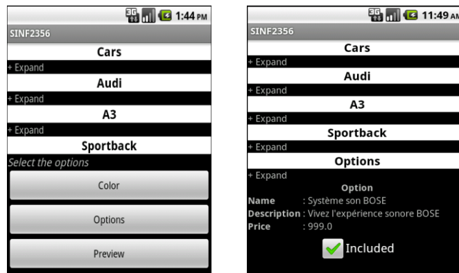
Fig. 7.21 Master/Details pattern in Android System
