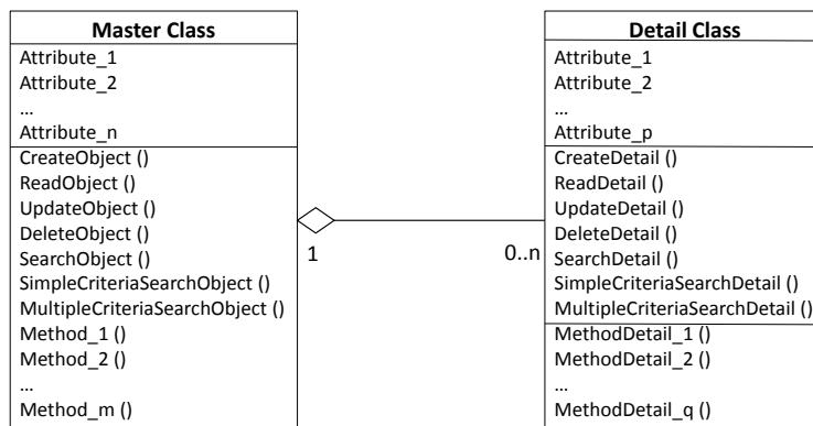
Fig. 7.11 The Master-Detail pattern in an aggregation relationship
