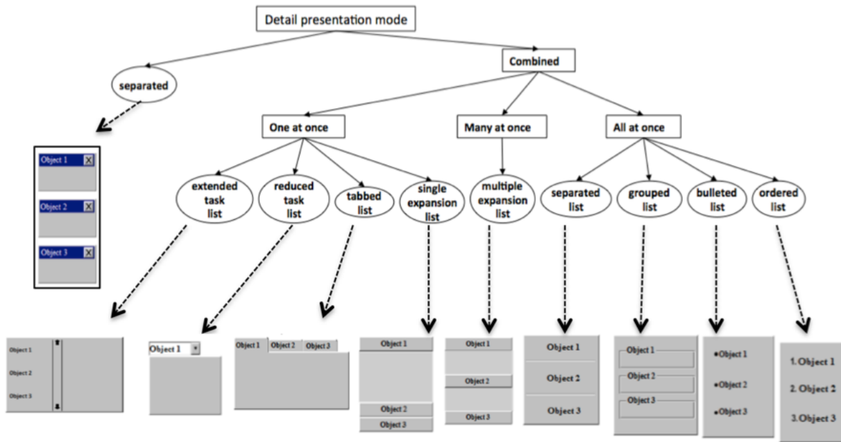
Fig. 7.16 Object Presentation in M/D pattern
