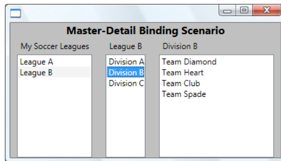
Fig. 7.1 An example of a UI implementation of the M-D pattern on desktop view.
