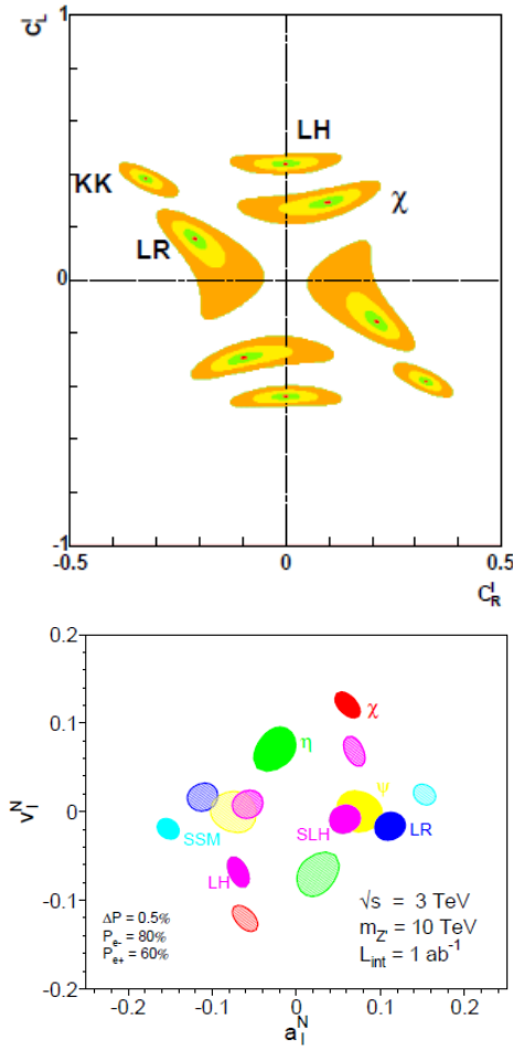
Fig. 121 Top: Resolving power (95% CL) for M_{Z'} = 1, 1.5 , and 2 TeV and \sqrt{s} = 500 GeV, \mathcal{L}_{\text{int}} = 1 \text{ ab}^{-1} , |P_{e-}| = 80\% , |P_{e+}| = 60\% , for leptonic couplings based on the leptonic observables \sigma , A_{\text{LR}} , A_{\text{FB}} . The couplings correspond to the E_6 \chi , LR, LH, and KK models. From Ref. [905]. Bottom: Expected resolution at CLIC with \sqrt{s} = 3 TeV and \mathcal{L} = 1 \text{ ab}^{-1} on the "normalised" leptonic couplings of a 10 TeV Z' in various models, assuming lepton universality. The mass of the Z' is assumed to be unknown. The couplings correspond to the E_6 \chi , \eta , and \psi , the SSM, LR, LH and SLH models. The couplings can only be determined up to a twofold ambiguity. The degeneracy between the \psi and SLH models might be lifted by including other channels in the analysis ( t\bar{t} , b\bar{b} , ...). From Refs. [9, 906].
