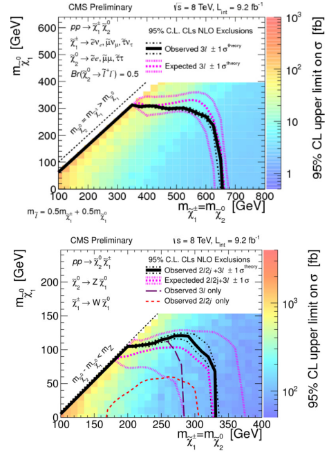
Fig. 126 95% CL exclusion limits on the chargino-neutralino production NLO cross section times branching fraction in the flavor-democratic scenario, for the three-lepton (upper panel), di-lepton WZ+MET and tri-lepton (lower panel) CMS searches with 9.2 \text{ fb}^{-1} of data at 8 TeV (from [1027]).
