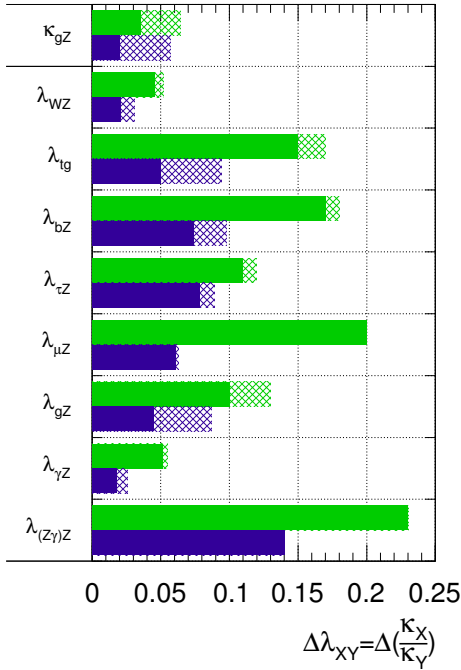
Fig. 34 Relative uncertainty expected for the ATLAS experiment on the determination of coupling scale factor ratios \lambda_{XY} = \kappa_X/\kappa_Y from a generic fit [129], assuming a SM Higgs boson with a mass of 125 GeV and 300 fb -1 and 3000 fb -1 of 14 TeV data. The hashed areas indicate the increase of the estimated error due to current theory uncertainties.
