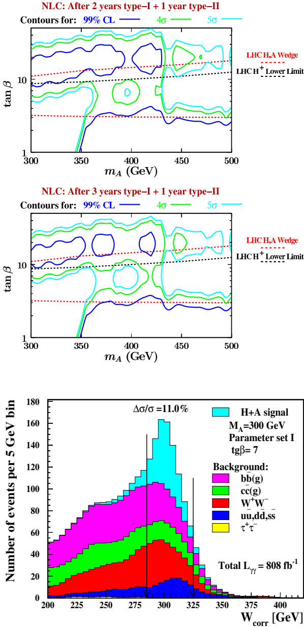
Fig. 99 Top: Production of A and H , with parameters corresponding to the LHC wedge, at the \gamma\gamma collider. Exclusion and discovery limits obtained for NLC collider for \sqrt{ee} = 630 GeV, after 2 or 3 years of operation [581], Bottom: The case M_H = M_A = 300 GeV at \chi_V^H \approx 0 in the MSSM. Distributions of the corrected invariant mass W_{\text{corr}} for selected b\bar{b} events at \tan\beta = 7 [582].
