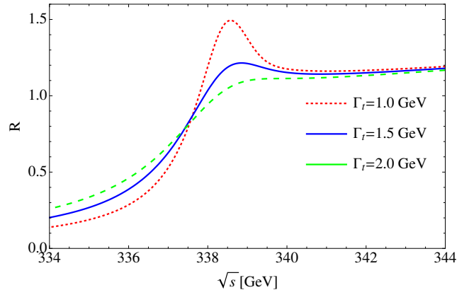
Fig. 101 The top quark production cross section R for m_t = 170\text{ GeV} and three values for top quark width. The LO formula for the cross section and \alpha_s(30\text{ GeV}) = 0.142 is used
