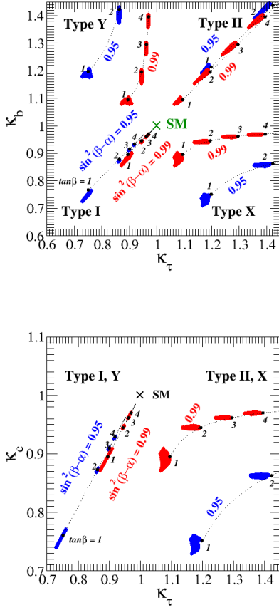
Fig. 70 Predictions of various scale factors on the \kappa_\tau vs \kappa_b (upper panel), and \kappa_\tau vs \kappa_c (bottom panel) in four types of Yukawa interactions in the cases with \cos(\beta - \alpha) < 0 [268]. Each black dot shows the tree level result with \tan\beta=1, 2, 3 and 4 . One-loop corrected results are indicated by red for \sin^2(\beta - \alpha) = 0.99 and blue for \sin^2(\beta - \alpha) = 0.95 regions where m_\Phi and M are scanned over from 100 GeV to 1 TeV and 0 to m_\Phi , respectively. All the plots are allowed by the unitarity and vacuum stability bounds.
