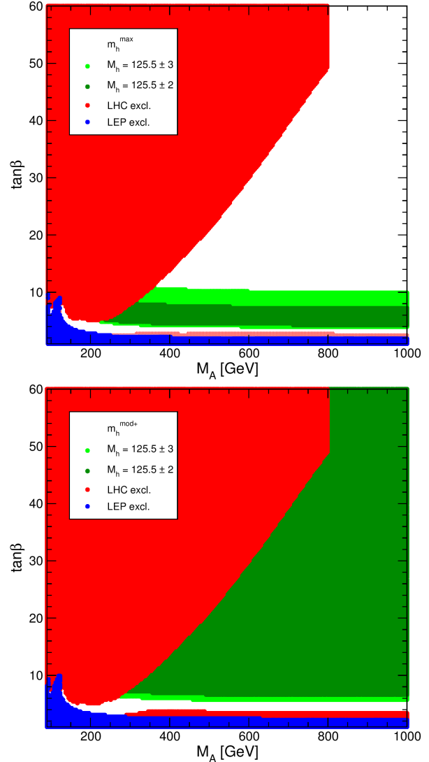
Fig. 61 M_A - \tan\beta plane in the m_h^{\max} scenario (upper) and in the m_h^{\text{mod}+} scenario (lower plot) [220]. The green shaded area yields M_h \sim 125 \pm 3 GeV, the red area at high \tan\beta is excluded by LHC heavy MSSM Higgs boson searches, the blue area is excluded by LEP Higgs searches, and the red strip at low \tan\beta is excluded by the LHC SM Higgs searches.
