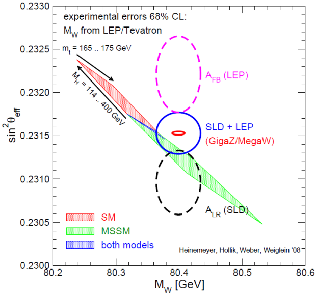
Fig. 114 MSSM parameter scan for M_W and \sin^2 \theta_{\text{eff}}^l over the ranges given in Eq. (115) with m_t = 165 \dots 175 GeV. Today's 68% C.L. ellipses (from A_{\text{FB}}^b(\text{LEP}) , A_{\text{LR}}^e(\text{SLD}) and the world average) are shown as well as the anticipated GigaZ/MegaW precisions, drawn around today's central value
