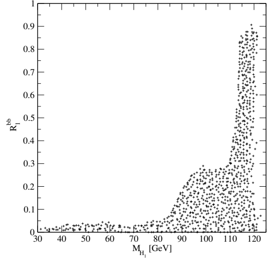
Fig. 87 The reduced signal cross section R_1^{bb} at a e^+e^- collider as defined in the text, as function of M_{H_1} in the semi-constrained NMSSM (from [424]).
