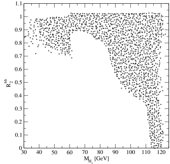
Fig. 88 The reduced signal cross section R_2^{bb} as function of M_{H_1} in the semi-constrained NMSSM (from [424]).
