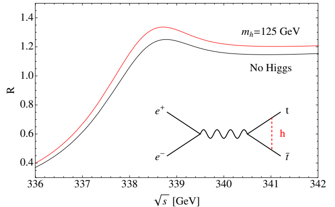
Fig. 105 Cross section for e^+e^- \rightarrow t\bar{t} for m_t = 170 \text{ GeV} with/without 1-loop Higgs boson corrections. A Higgs boson mass of m_h = 125 \text{ GeV} is used.
