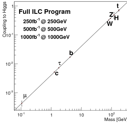
Fig. 12 Upper plot: Threshold rise of the Cross section for Higgs-strahlung e^+e^- \rightarrow ZH corresponding to Higgs spin = 0, 1, 2, complemented by the analysis of angular correlations; lower plot: Measurements of Higgs couplings as a function of particle masses.
