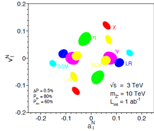
Fig. 10 New gauge bosons in the \mu^+\mu^- channel. The plot shows the expected resolution at CLIC with \sqrt{s} = 3 TeV and \mathcal{L} = 1 \text{ ab}^{-1} on the ‘normalized’ vector v_f^N = v_f^N / \sqrt{s / (m_{Z'}^2 - s)} and axial-vector a_f^N = a_f^N / \sqrt{s / (m_{Z'}^2 - s)} couplings to a 10 TeV Z' in terms of the SM couplings v_f^N, a_f^N . The mass of Z' is assumed to be unknown, nevertheless the couplings can be determined up to a two-fold ambiguity. The colours denote different Z' models [9].
