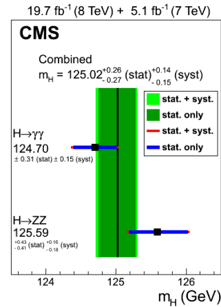
Fig. 25 CMS mass measurements [106] in the \gamma\gamma and ZZ \rightarrow 4\ell final states and their combinations. The vertical band shows the combined uncertainty. The horizontal bars indicate the \pm 1 standard deviation uncertainties for the individual channels.
