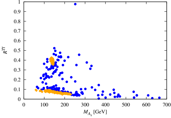
Fig. 91 The reduced coupling R^{\gamma\gamma} as function of M_{A_S} , for points in the semi-constrained NMSSM where H_S with M_{H_S} \sim 100 GeV explains the excess in bb at LEP II (from [434]; orange diamonds satisfy the WMAP constraint on the dark matter relic density).
