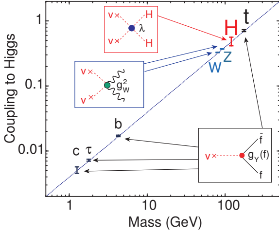
Fig. 39 Mass-coupling relation [136].
