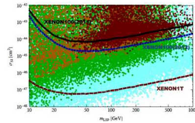
Fig. 157 Spin-independent direct detection cross section \sigma_{\text{SI}} on protons vs. dark matter mass m_{\text{LSP}} , from [1237]. The black (blue) line are the 90% CL limits from the XENON100(2011) [1238] and (2012) results [1010]. The dashed brown line is the projected sensitivity of the XENON1T experiment [1239]. The color code shows the with P > 0.2 (red), 0.1 < P < 0.2 (orange), 0.01 < P < 0.1 (green) and 0.001 < P < 0.01 (blue). Note however that the relic density constraint is not imposed here.
