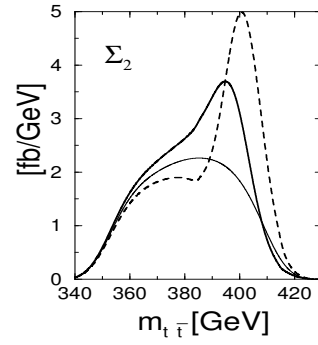
Fig. 100 The specific decay angular distributions \Sigma_i in the \gamma\gamma \rightarrow h^{(i)} \rightarrow t\bar{t} process in dependence on the t\bar{t} invariant mass for the scalar (dashed) and pseudoscalar (thick solid) h^{(i)} with M_H = 400 GeV [588].
