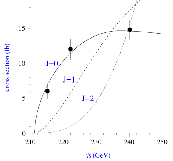
Fig. 44 Threshold scan of the e^+e^- \rightarrow Zh process for m_h = 120 GeV, compared with theoretical predictions for J^P = 0^+, 1^-, and 2^+ [146].
