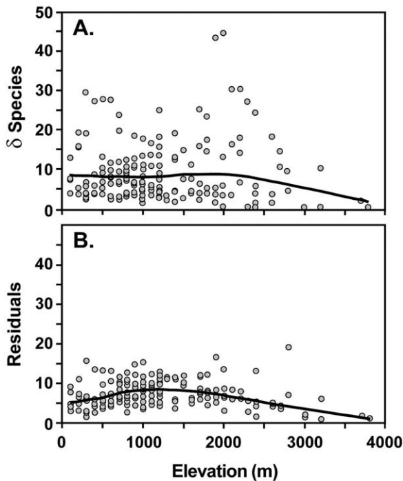
Figure 3 (a) Elevational pattern of species richness ( S_{int} , all analysis-grade gradients pooled and adjusted to the same average richness; \delta Species). Note that both y-axes have linear scaling, while log-transformed and standardized data were used for modelling. (b) Elevational pattern of residuals from the 'best' model (lowest AICc, pseudo- R^2 = 0.40 ). LOESS fits (black lines) are shown to visualize overall patterns in the data. See main text for linear and quadratic fits. Similar patterns were recovered when using the 'best subset' data alone (not shown).
