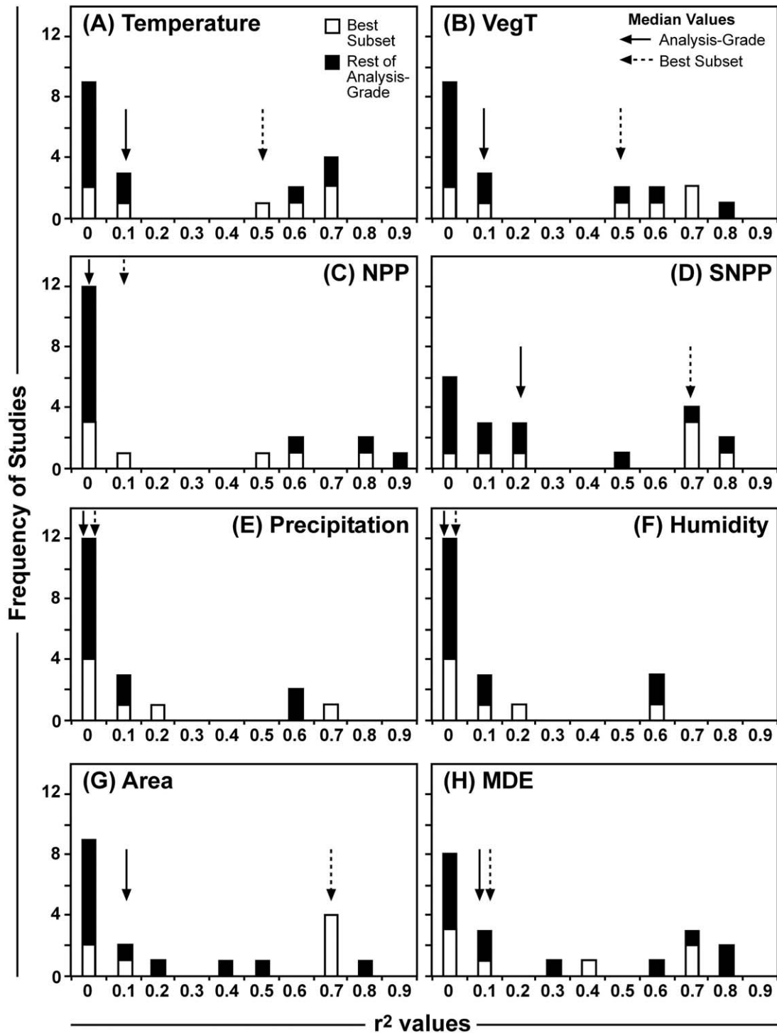
Figure 2 Frequency distributions of Pearson's r^2 values for univariate correlations of environmental and spatial predictors with richness ( S_{int} ) within gradients. Data for 19 analysis-grade gradients are shown as bars. Arrows indicate the median r^2 . Note that r^2 for negative correlations was set to zero, because only positive correlations were expected by our hypotheses. Definitions: VegT, mean annual temperature in non-freezing months; NPP, average net primary productivity; SNPP, summed NPP across the elevational band; MDE, mid-domain effect.
