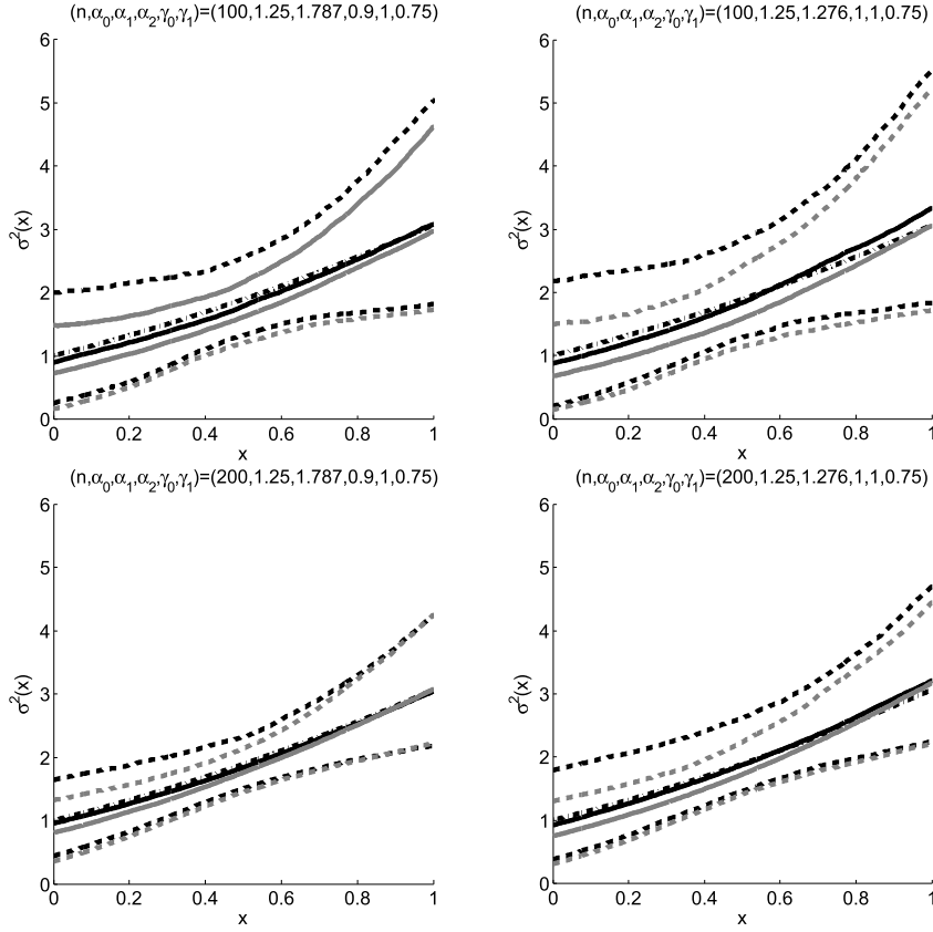
FIG 1. Comparison of the estimated conditional variances obtained with \tilde{\theta}_n (grey curves) and \hat{\theta}_n^T (black curves) for model (4.3). Dashed curves: 5% and 95% quantiles of the empirical distribution based on the estimated conditional variances; solid curve: median of this empirical distribution; dash-dotted curve: true conditional variance curve.
