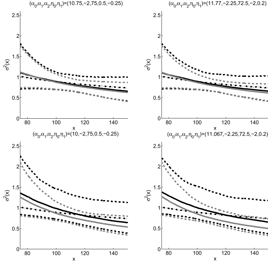
FIG 2. Comparison of the estimated conditional variances obtained with \tilde{\theta}_n (grey curves) and \hat{\theta}_n^T (black curves) for model (4.4). Dashed curves: 5% and 95% quantiles of the empirical distribution based on the estimated conditional variances; solid curve: median of this empirical distribution; dash-dotted curve: true conditional variance curve.
