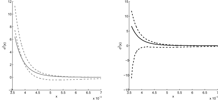
FIG 5. Fatigue life data. Confidence intervals for \sigma_{\theta_0^T}^2(x) based on the basic bootstrap where strain domain is restricted to values below 0.007; on the left, constructed with the estimated distribution of \sigma_{\theta_n}^2(x) and, on the right, with the estimated distribution of \sigma_{\theta_n^T}^2(x) (for each value of x ).
