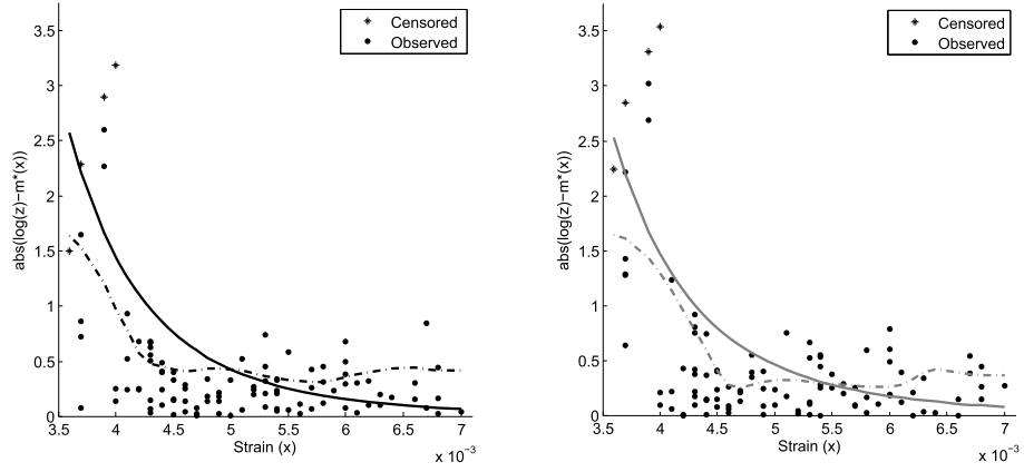
FIG 7. Fatigue life data. Scatter plot of the residuals of a nonparametric fit versus the strain with m^*(x) = \hat{m}^T(x) for the left panel and m^*(x) = \hat{m}(x) for the right panel. Solid black and grey curves correspond to \hat{\sigma}_{\hat{\delta}_n^T}(x) and \hat{\sigma}_{\hat{\delta}_n}(x) respectively; dash-dotted black and grey curves represent the nonparametric \hat{\sigma}^T(x) and \hat{\sigma}(x) respectively for x \in [0.0036; 0.0070] .
