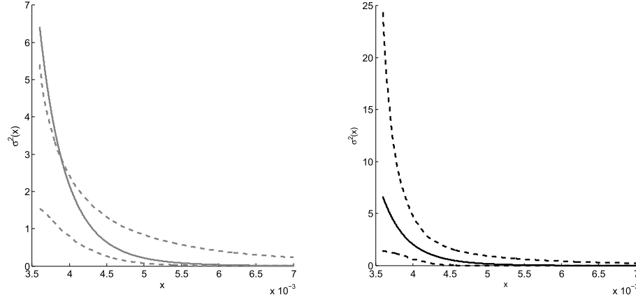
FIG 6. Fatigue life data. Confidence intervals for \sigma_{\theta_0^T}^2(x) based on the percentile bootstrap where strain domain is restricted to values below 0.007; on the left, constructed with the estimated distribution of \sigma_{\theta_n}^2(x) and, on the right, with the estimated distribution of \sigma_{\theta_n^T}^2(x) (for each value of x ).
