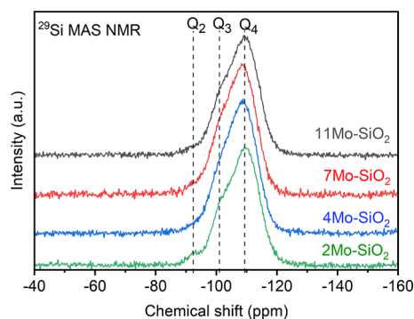
Figure 1. 29 Si MAS NMR spectra of molybdenum-silicate catalysts.
