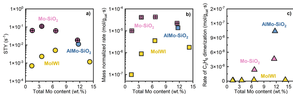
Figure 6. Reactivity of Mo–SiO 2 , Al1Mo–SiO 2 , and MoIWI catalysts, (a) STY of propylene metathesis, (b) rate of propylene metathesis, and (c) rate of propylene dimerization. Conditions: 10–50 mg of catalyst, 50% propylene in a helium balance, and 50 mL min −1 total flow rate under atmospheric pressure at 200 °C.
