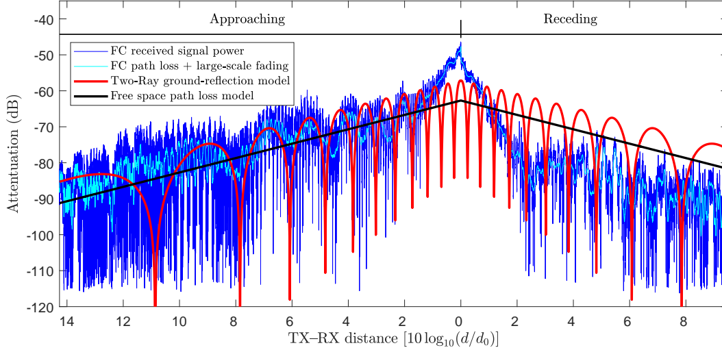
Fig. 6. Attenuation, extracted path loss and large-scale fading along side the free space path and Two-Ray ground-reflection path loss models ( P_t = 0 dBm, G_t = G_r = 1 , h_t = h_C = 1.2 m, h_r = h_{FC} = 1.5 m, \epsilon_g = 0.34 ) for the FC channel in Scenario A.
