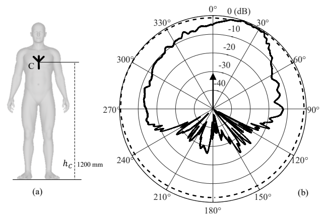
Fig. 1. (a) Illustration of the TX node position on the central chest (C) region of the pedestrian and (b) its measured azimuthal directivity pattern (black continuous line) with the same sleeve dipole antenna in free space (black dashed line). The upward arrow in (b) denotes the forward direction from the pedestrian's chest.
