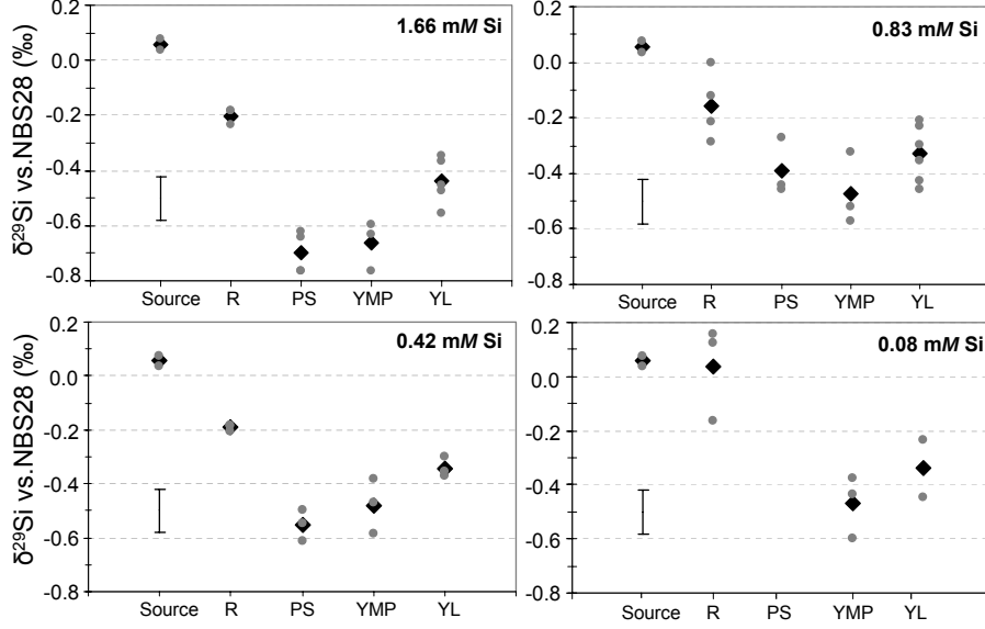
Figure 7.3: Si-isotopic compositions ( \delta^{29}\text{Si} vs. NBS28) in banana plantlets at four different Si supplies (0.08, 0.42, 0.83, 1.66 mM Si): single measurements (grey circles) and their average (black diamonds). Brackets show the average standard deviation of full replicates ( \pm 2\sigma_{SD} ). Source = solution, R = roots, PS = pseudostems, YMP = young midribs and petioles, YL = young lamina.
