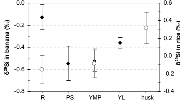
Figure 7.4: Comparison between Si-isotopic compositions ( \delta^{29}\text{Si} (‰)) in banana (this study) and rice (Ding et al., 2005b). Brackets show the standard deviation. R = roots, PS = pseudostems, YMP = young midribs and petioles, YL = young lamina, husk = in rice (PS-YMP-YL are represented by one point Stem-Leaf in rice). Banana = diamond; Rice = circle rice.
