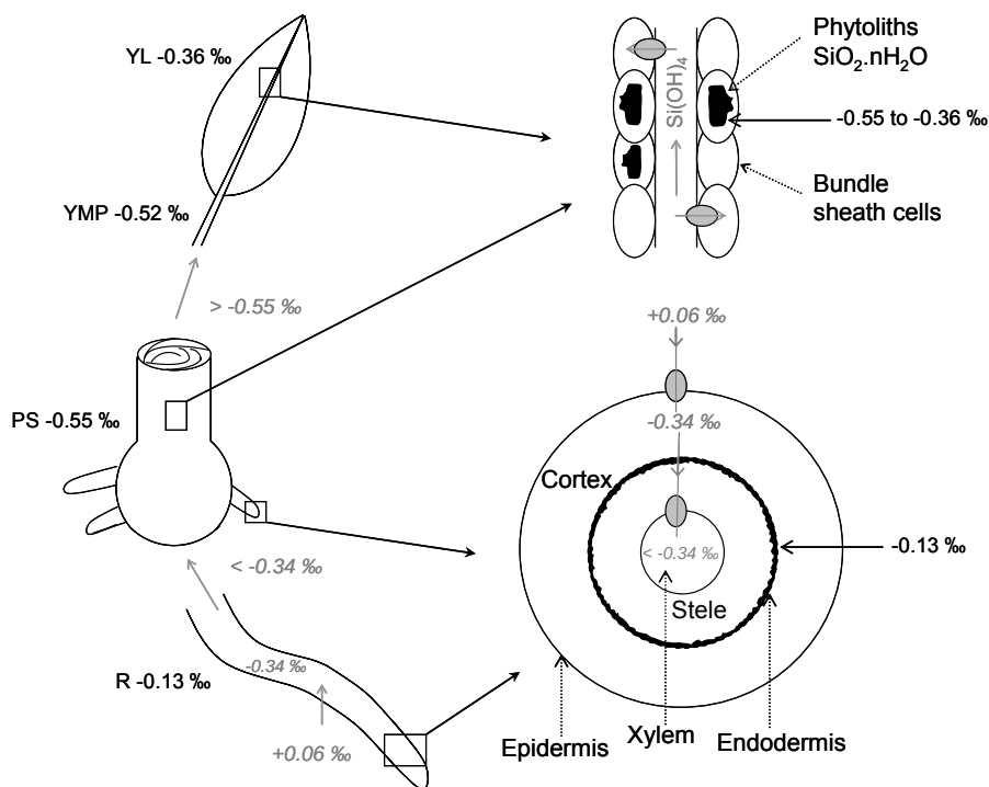
Figure 7.5: Proposed schematic model of global Si-isotopic fractionation in banana. Black = Si-isotopic composition of biogenic silica; grey and italic = Si-isotopic composition of \text{H}_4\text{SiO}_4 ( \delta^{29}\text{Si} vs. NBS28 (‰)). R = roots, PS = pseudostems, YMP = young midribs and petioles, YL = young lamina.
