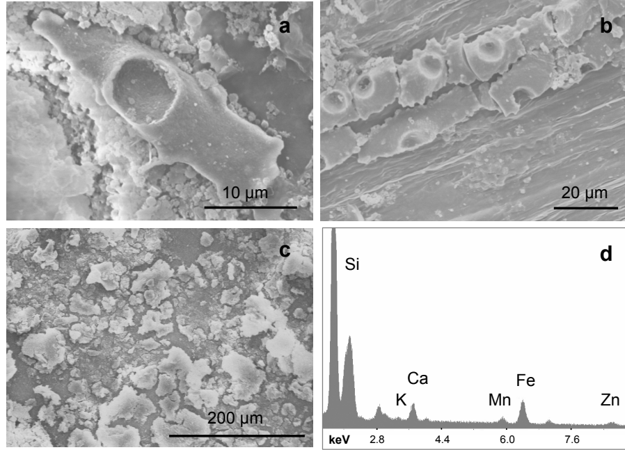
Figure 7.2: Morphological studies in banana: (a) Shoots: SEM image of a typical cone shaped phytolith truncated saddle-like - (b) Shoots: SEM image of long phytoliths chain in pseudostems - (c) Roots: SEM image of the roots residual matter after organic digestion - (d) Roots: EDX analysis of the roots residue. Unlabelled peaks represent Au-Pd from the coating or secondary peaks.
