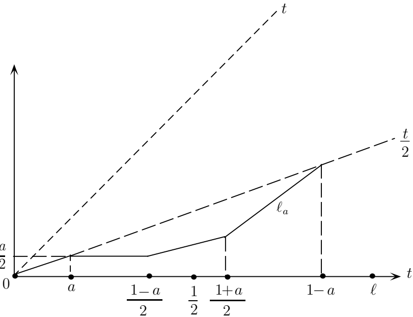
Figure 1: Graph of the median \ell_a
