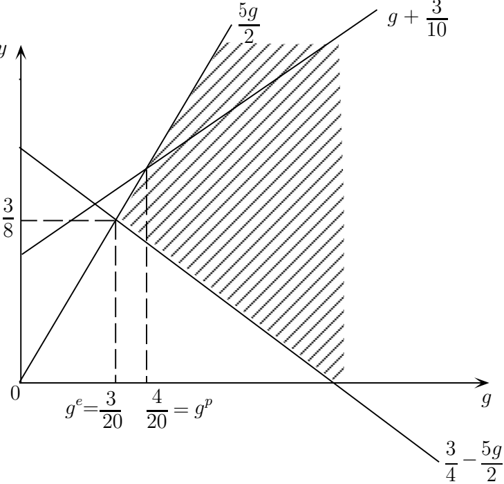
Figure 2: Secession proof transfers in example 6.7
