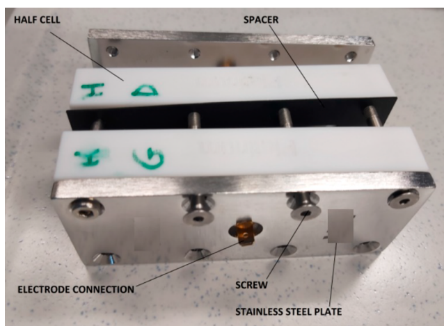
Figure 3. Electrochemical cell.
