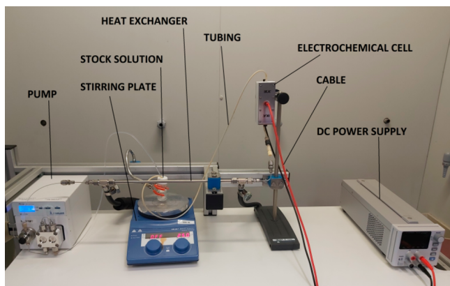
Figure 2. ElectraSyn Flow setup.
