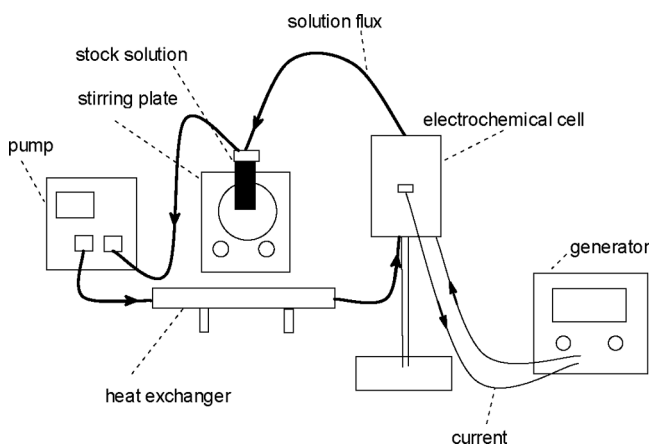
Figure 1. Diagram of the ElectraSyn Flow setup.
