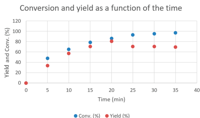
Figure 5. Kinetic study of the electrocyclization of 1-allyl-4-propylpyrrolidin-2-one 2 using a flow rate of 6 mL/min.
