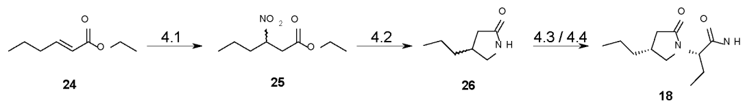
Scheme 7. Synthesis of Brivaracetam (Ates et al. 18 )
