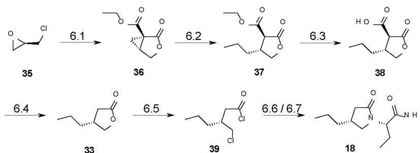
Scheme 10. Synthesis of Brivaracetam (Defrance et al. 21 )
