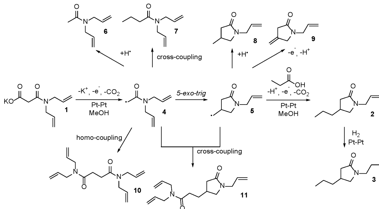
Scheme 4. Synthesis of Brivaracetam (Ates et al. 15 )
