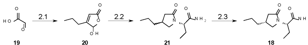
Scheme 6. Synthesis of Brivaracetam (Surtees et al. 17 )
