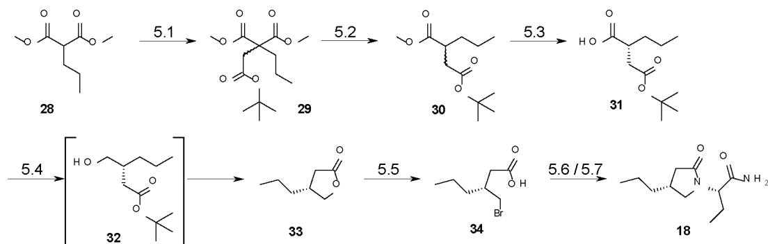
Scheme 9. Synthesis of Brivaracetam (Wang et al. 20 )
