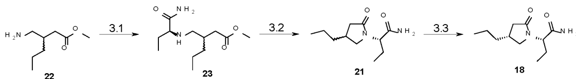
Scheme 7. Synthesis of Brivaracetam (Ates et al. 18 )
