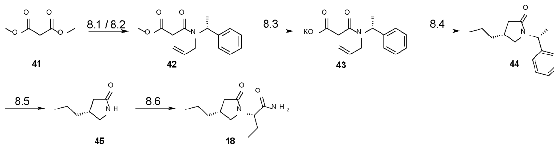
Scheme 11. Proposal for the Synthesis of Brivaracetam Based on Electrocyclization
