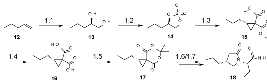
Scheme 5. Synthesis of Brivaracetam (Surtees et al. 16 )
