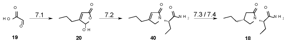
Scheme 11. Proposal for the Synthesis of Brivaracetam Based on Electrocyclization
