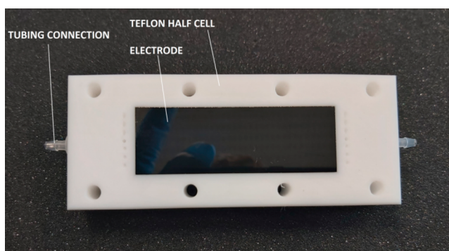
Figure 4. Half-cell.
