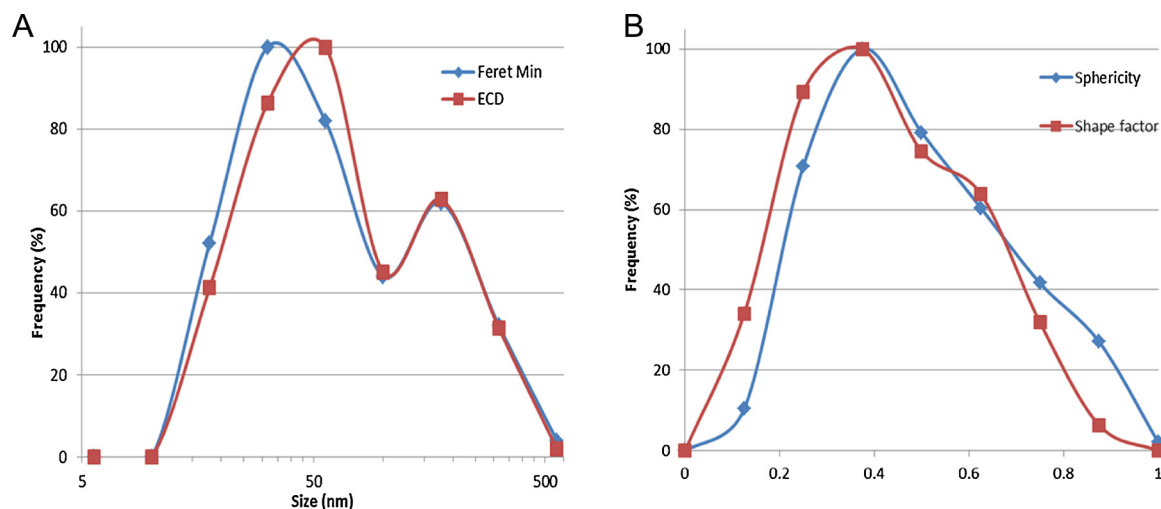
Fig. 2. Summary of the quantitative TEM characterization of silica NM-200 dispersed for in vivo use: (A) Feret-Min and ECD (equivalent circle diameter), and (B) sphericity and shape factor.
