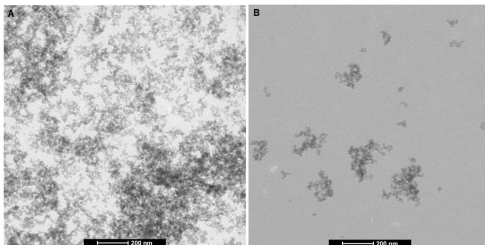
Fig. 1. Representative TEM images of the NM-200 dispersion (A) undiluted, prepared for in vivo use as such, and (B) diluted 100 times in PBS for quantitative TEM characterization.
