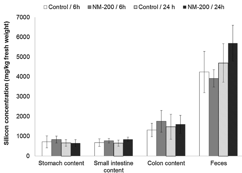
Fig. 4. Silicon concentration in the gastro-intestinal tract (mg/kg fresh weight), 6 h or 24 h after intravenous administration of NM-200 (20 mg/kg bodyweight) or PBS (Control). Data are expressed as the mean \pm standard deviation (n = 5).
