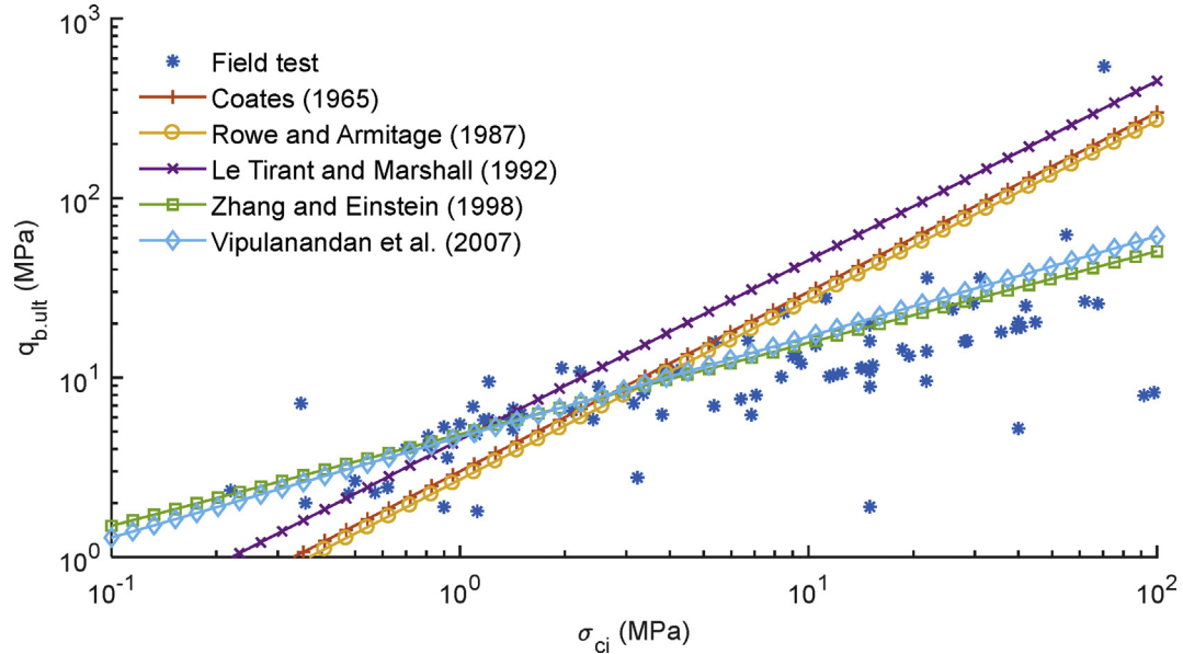
Fig. 5. Ultimate end bearing capacity as a function of the unconfined compressive strength \sigma_{ci} : Field test vs. empirical relations from Coates (1965), Rowe and Armitage (1987), Le Tirant and Marshall (1992), Zhang and Einstein (1998), and Vipulanandan et al. (2007).
