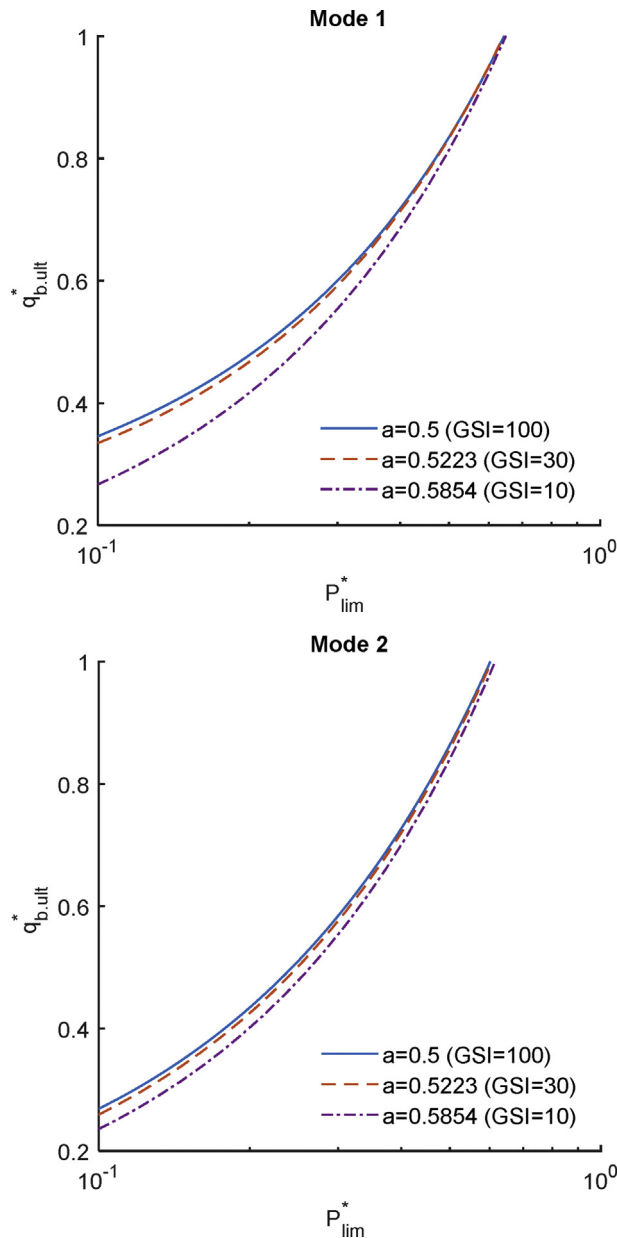
Fig. 4. 'True' ultimate bearing capacity for failure mechanisms of modes 1 and 2.
