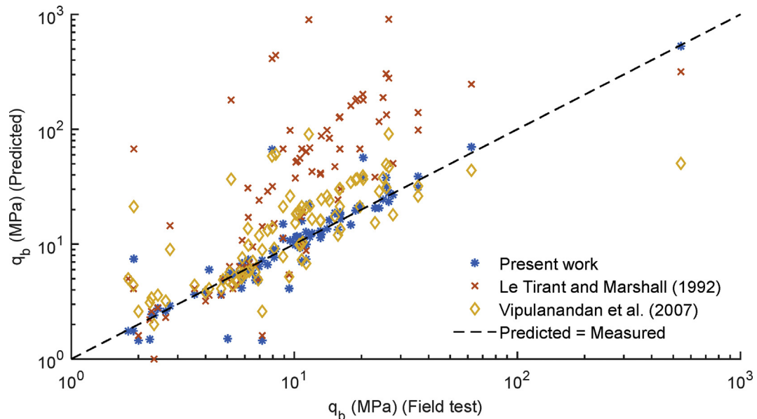
Fig. 6. End bearing resistance: Present work solution vs. empirical approaches from Le Tirant and Marshall (1992) and Vipulanandan et al. (2007).
