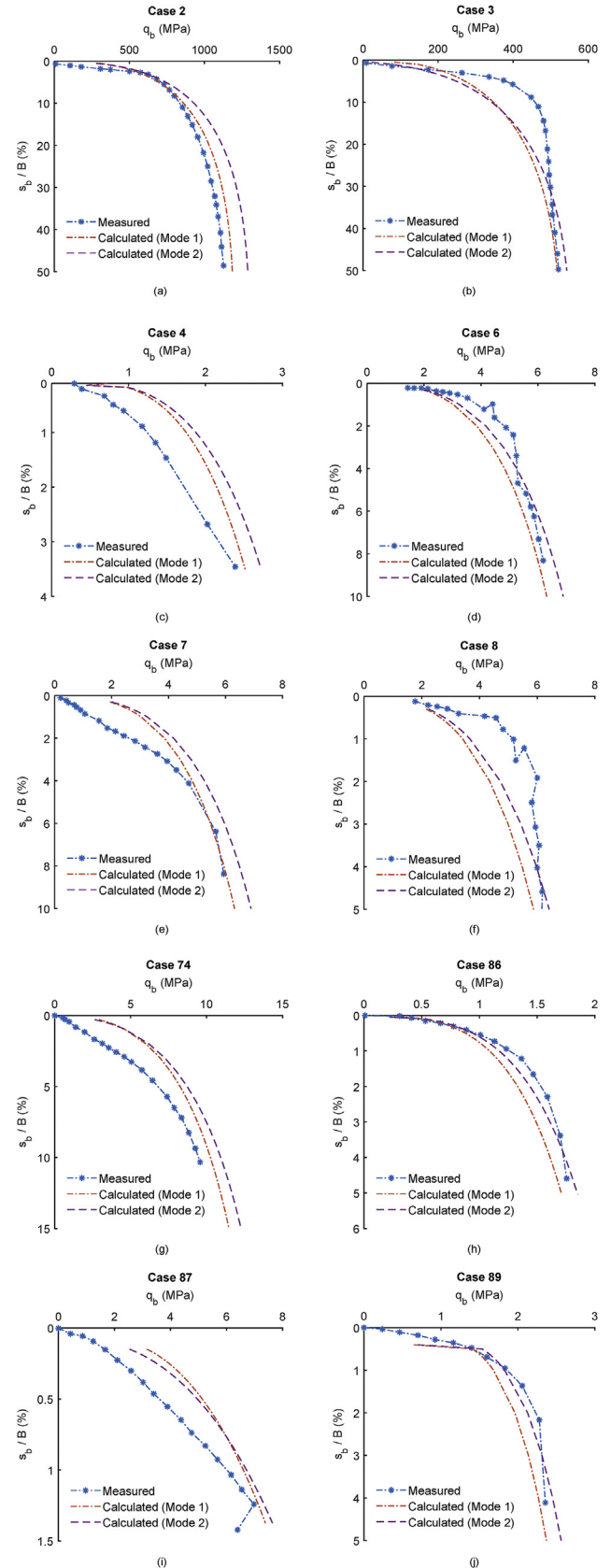
Fig. 7. Load-displacement curves: Present work vs. field test.
