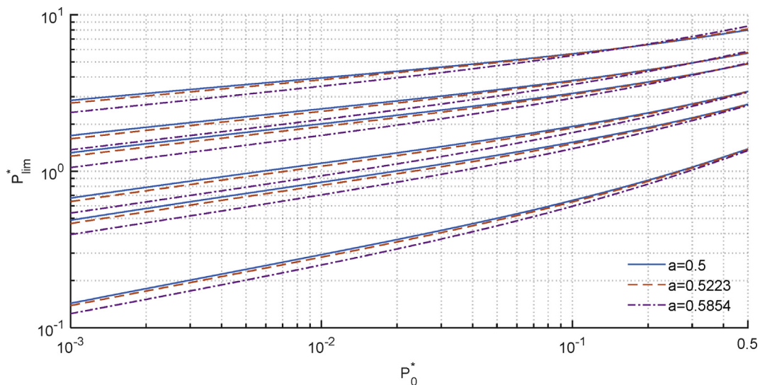
Fig. 3. Limit pressure chart by setting \psi = 0^\circ and \nu = 0.25 (after Gharsallaoui et al., 2020). Values of I_r^{-1} = 10^{-3}, 5 \times 10^{-3}, 10^{-2}, 5 \times 10^{-2}, 10^{-1} , and 1 correspond to the groups of curves from top to bottom.
