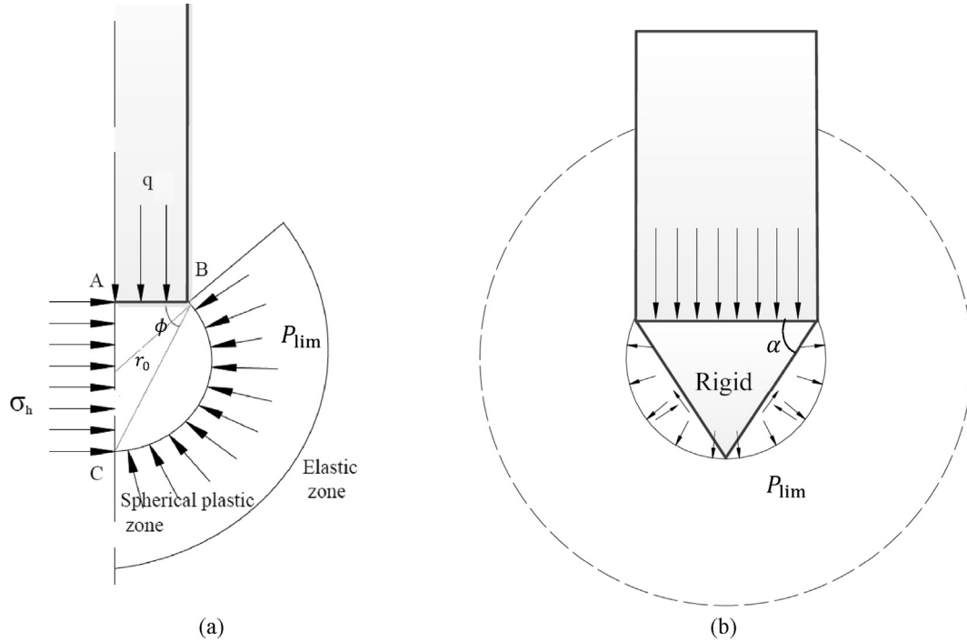
Fig. 1. Sketches of failure mechanisms around the pile tip: (a) Yasufuku and Hyde (1995), and (b) Vesic (1973).
