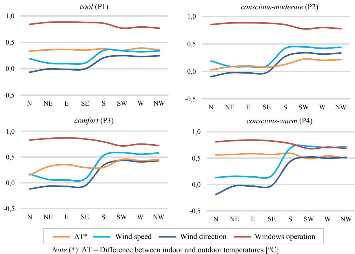
Figure 7. Rank correlation coefficients for different parameters in all profiles with respect to ventilation rate [ \text{h}^{-1} ] in the main bedroom per orientation
