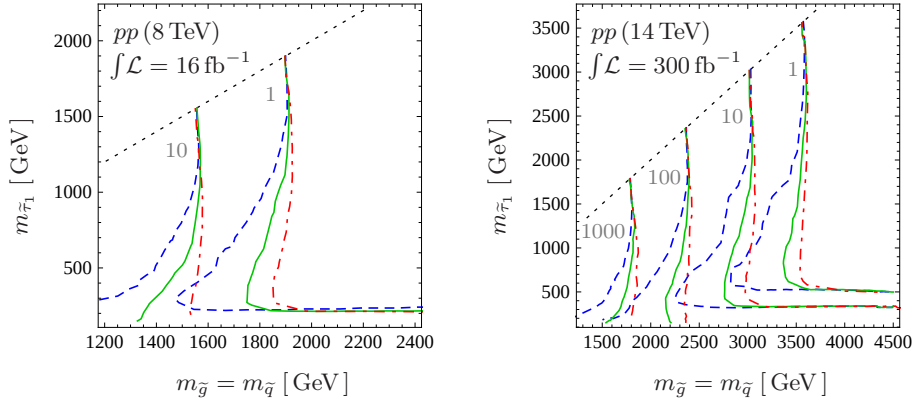
Figure 9: Number of events that contain at least one stau which is stopped inside the detector for the simplified models \mathcal{A} (blue dashed), \mathcal{B} (green solid) and \mathcal{C} (red dot-dashed). The iso-event-number curves are displayed in the m_{\tilde{g}}-m_{\tilde{\tau}_1} plane where we have chosen the common squark mass scenario and m_{\tilde{q}} = m_{\tilde{g}} .
