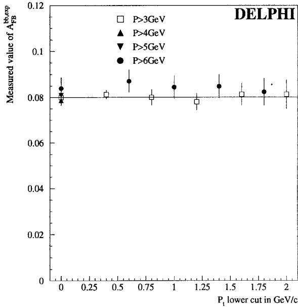
Fig. 8. Measured values of A_{\text{FB}}^{bb,\text{exp}} for various values of the p_t cut as a function of the p_t cut. The reference line is drawn from the point p > 3 GeV/c, no p_t cut
