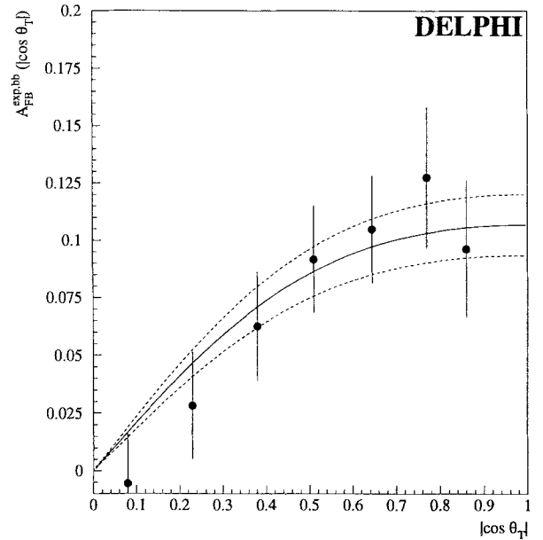
Fig. 7. Observed values of A_{FB}^{bb,exp}(x) = A_{FB}^{bb,exp} \frac{8}{3} \frac{x}{1+x^2} for different x = |\cos \theta_T| . Full curve: \chi^2 fit; dashed curves: one standard deviation from the central value; data points: observed asymmetries at the center of the \cos \theta_T bin
