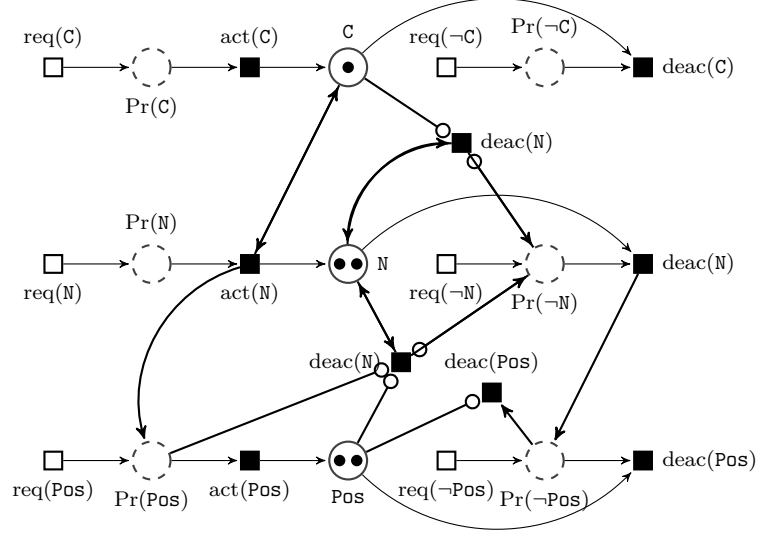
Figure 6.9: Composition of two CoPNs \mathcal{P}_1 = o(\{\mathcal{C}_N, \mathcal{C}_{Pos}\}, \{\langle I, \mathcal{C}_N, \mathcal{C}_{Pos} \rangle\}) and \mathcal{P}_2 = o(\{\mathcal{C}_N, \mathcal{C}_C\}, \{\langle Q, \mathcal{C}_N, \mathcal{C}_C \rangle\}) with an implication (N \blacktriangleright Pos) and a requirement (N \blacktriangleleft C) .
