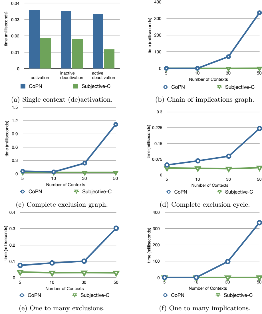
Figure 9.8: Benchmark results for the activation and deactivation of contexts with context dependency relations in CoPNs and Subjective-C.
