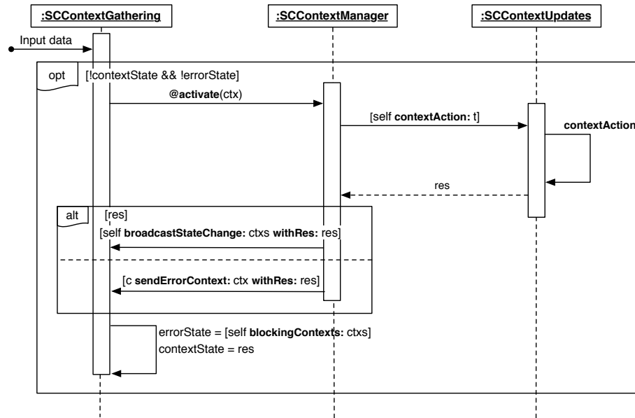
Figure 8.6: Process for context activation.
