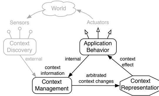
Figure 4.5: General context-awareness architecture [27] of Subjective-C.
