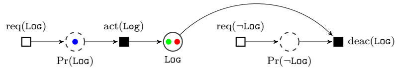
Figure 9.4: Three local activations for the LOG context.
