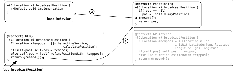
(b) Method call with multiple active contexts and timestamps
