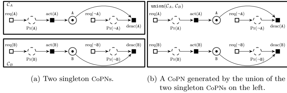
Figure 6.2: Application of the union function to two singleton CoPNs.
