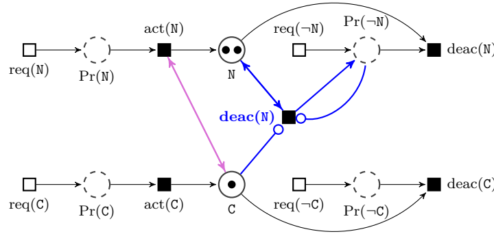
Figure 6.6: Requirement dependency relation ( \mathbf{N} \leftarrow \mathbf{C} ).
