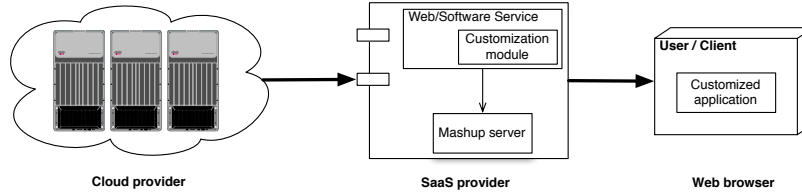
Figure 3.3: SaaS component architecture overview [8, 24].
