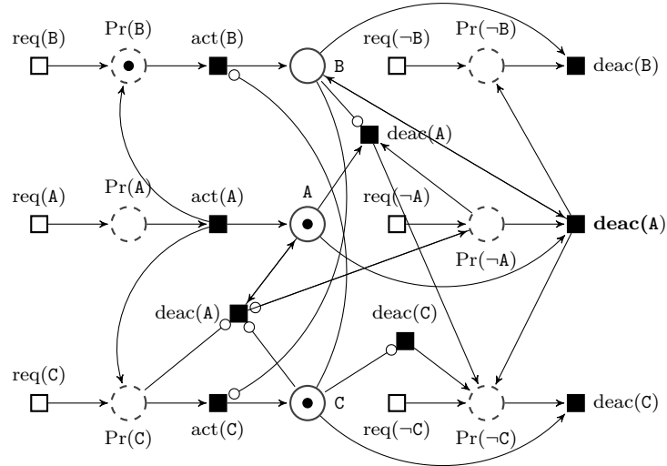
Figure 7.2: A CoPN with non-reachable context \mathbf{A} .
