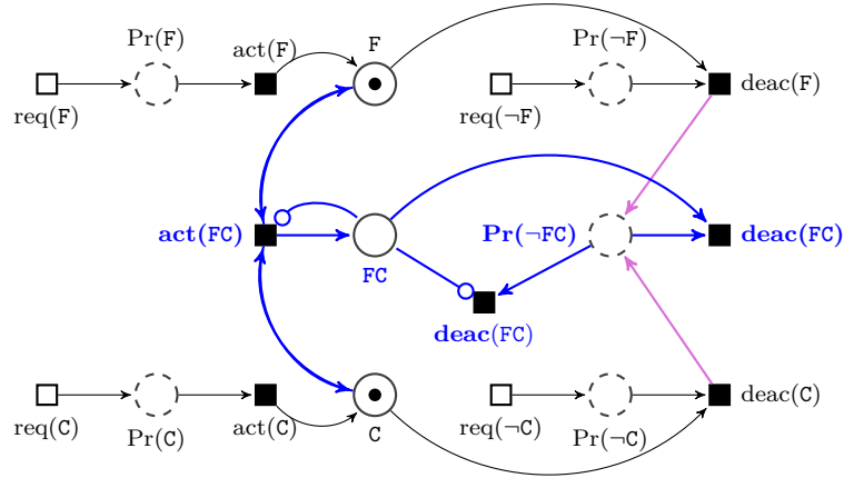
Figure 6.7: Conjunction dependency relation ( \rightarrow(F C) ).
