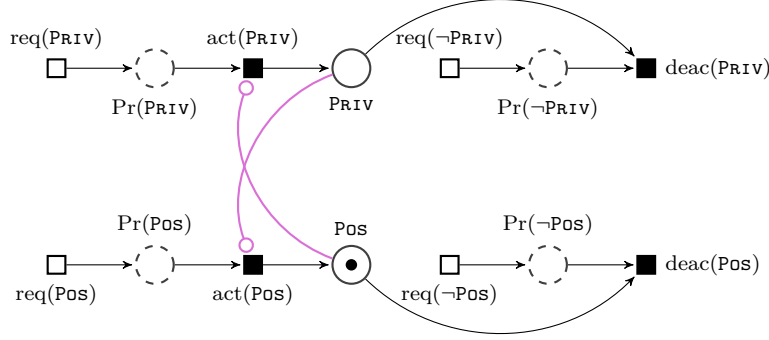
Figure 6.3: Exclusion dependency relation ( \text{PRIV} \perp \text{POS} ).
