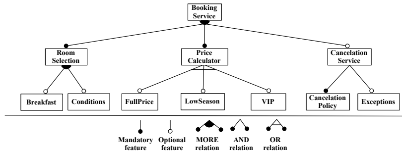
Figure 3.5: Feature model aggregation for the web booking application.
