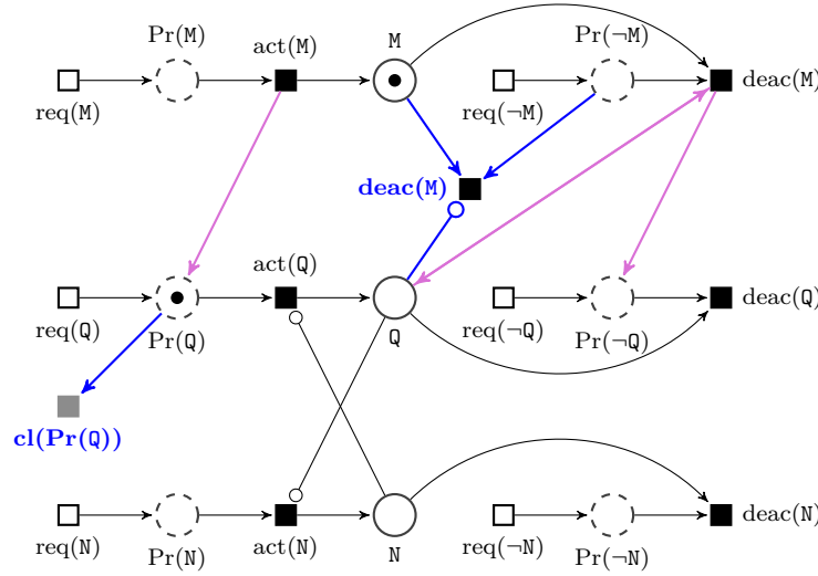
Figure 9.7: Suggestion dependency relation ( M \dashrightarrow Q ) and exclusion dependency relation ( Q \boxminus N ).
