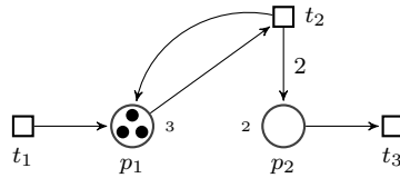
Figure 5.2: A Petri net with place capacities.
