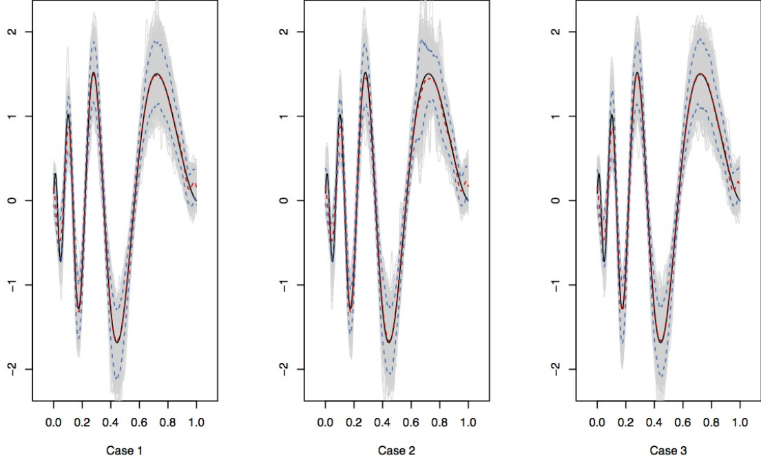
Figure 3: The grey graphs depict the Monte-Carlo realisations of the data-driven estimator \hat{f}_{\hat{m}} for the regression f_1 in the three cases of weak-dependence. The solid line corresponds to the true function, the red dashed line and the blue dashed lines represent, respectively, the point-wise median and the 5% and 95% point-wise percentile of the 501 replications.
