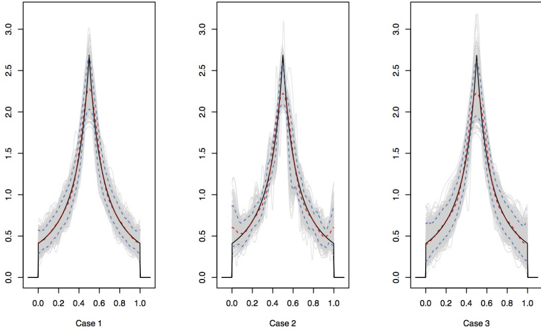
Figure 2: The grey graphs depict the Monte-Carlo realisations of the data-driven estimator \hat{f}_{\hat{m}} for the density f_2 in the three cases of weak-dependence. The solid line corresponds to the true function, the red dashed line and the blue dashed lines represent, respectively, the point-wise median and the 5% and 95% point-wise percentile of the 501 replications.
