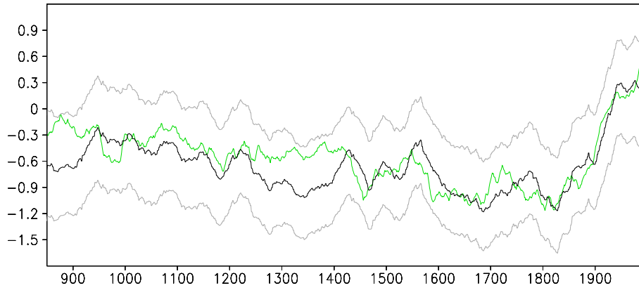
Figure 5.5: Anomaly in annual mean surface temperature (°C) averaged over the Arctic for the IND simulation (green) and the PAGES2k reconstruction (black) with error bars (grey). The reference period is 1901-1970. A 41-year running mean has been applied to the time series. The correlation between the time series is given in Table 5.6.
