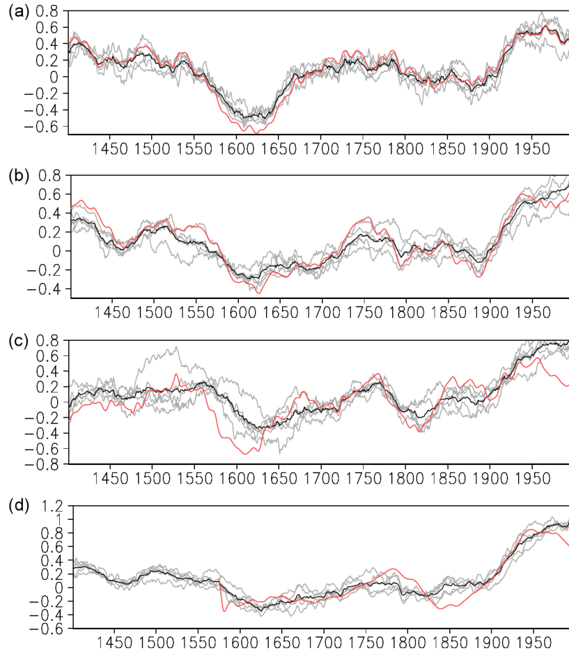
Figure 2.4: (a) Time series of the anomaly in annual mean surface temperature (°C) over the last 600 years for the region in the box A in Fig. 2.3. The black line is the mean over the 5 model simulations, the red line is the average over the 6 proxy data contained in box A in Fig. 2.3, and the grey lines are the results of the 5 different model simulations. (b) Same as a) for the mean over box B in Fig. 2.3 (5 proxies). (c) Same as a) for the mean over box C in Fig. 2.3 (2 proxies). (d) Anomaly of annual mean surface temperature in the Arctic for the last 600 years. The Arctic area corresponds to the mean over all longitudes between 64°N and 80°N. The red curve is the reconstruction of Overpeck et al. (1997). A 51-year running mean has been applied to all time series. The reference period is 1600-1950.
