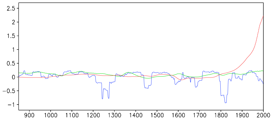
Figure 1.3: Estimates of past changes in annual mean radiative forcing ( Wm^{-2} ), as used in Crespín et al. (2012): solar forcing in green, volcanic forcing in blue, and greenhouse gas forcing in red. See Section 3.2 for references. A 25-year running mean has been applied to the time series.
