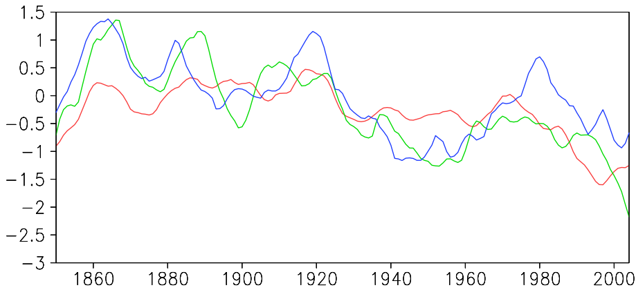
Figure 4.6: Time series of the annual mean of the MOC maximum anomaly in the North Atlantic ( \text{Sv} ). The ALL experiment is in blue, the ATL experiment in green, and the mean of an ensemble of 10 simulations made without data assimilation in red. An 11-year running mean has been applied to the time series. The reference period is 1880-1950.
