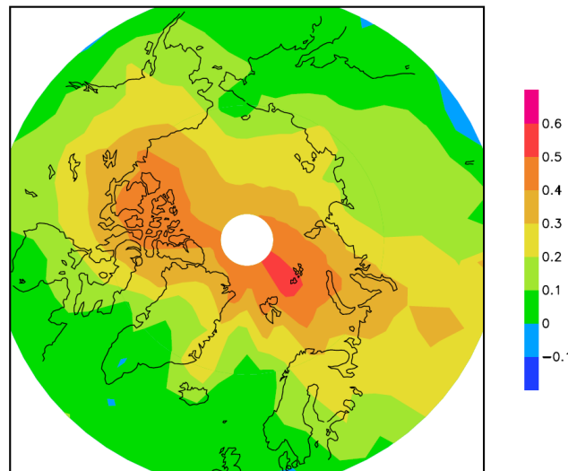
Figure 2.6: Anomaly in annual mean surface temperature ( ^{\circ}\text{C} ) over the 1470-1520 warm period for the model results averaged over the 5 simulations with data assimilation. The reference period is 1600-1950.
