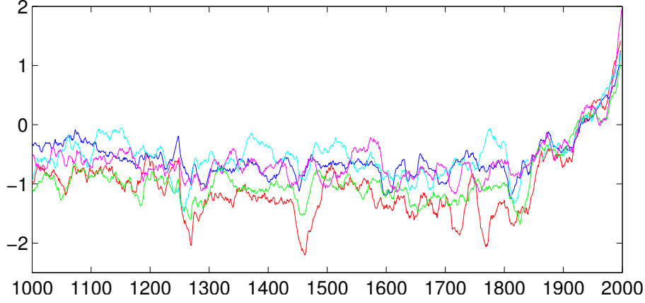
Figure 1.4: Anomaly in Arctic annual mean surface temperature (°C) simulated by 5 different GCMs: CCSM4 (USA) in red, GISS-E2-R (USA) in blue, IPSL-CM5A-LR (France) in green, MPI-ESM-P (Germany) in cyan, and Bcc-csm1-1 (China) in magenta. A 21-year running mean has been applied to the time series. The reference period is 1900-1970. (Data collected and processed by F. Klein).
