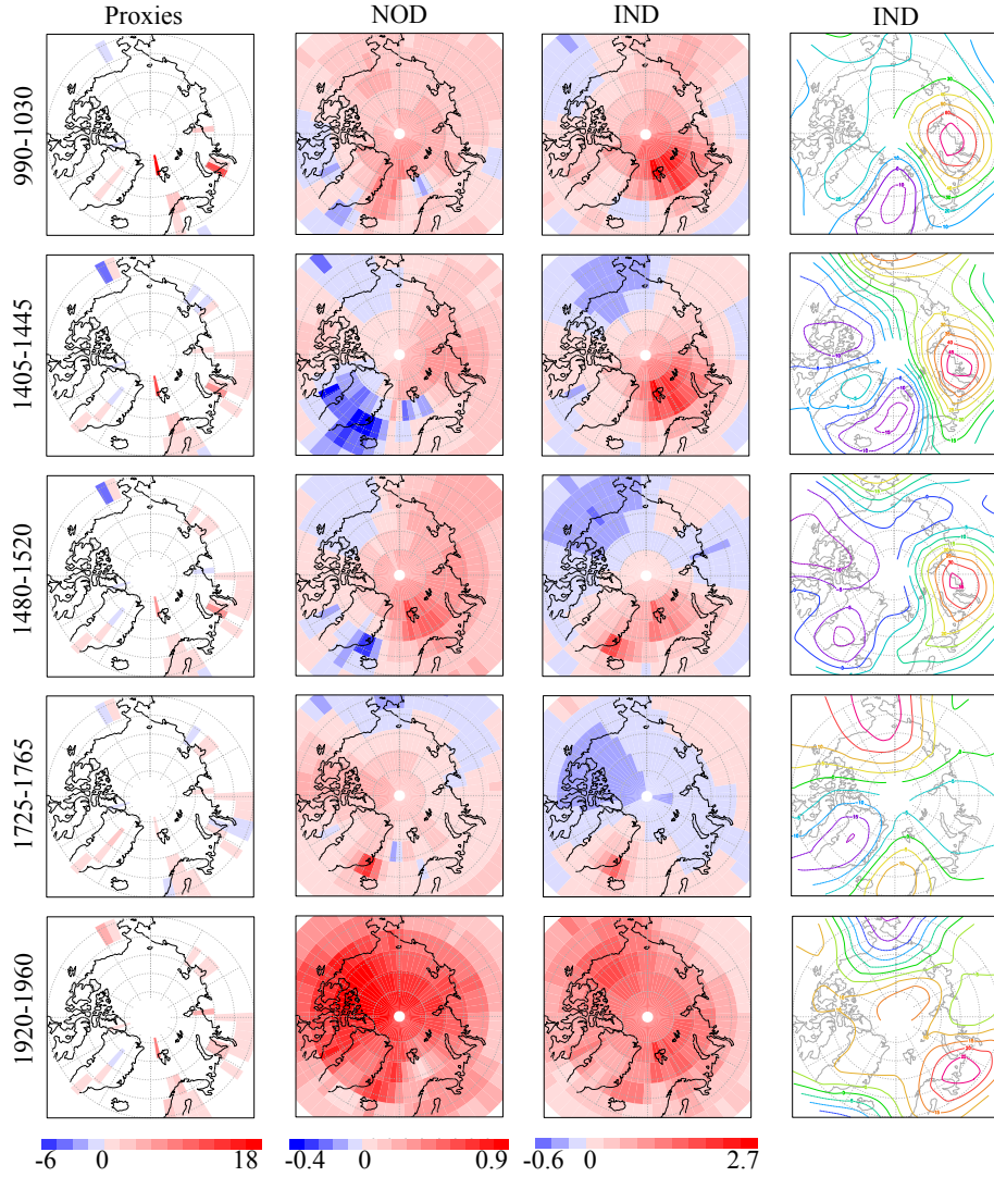
Figure 5.6: Anomaly in annual mean surface temperature (°C) over 5 different warm periods for the proxy-based reconstructions calibrated by indirect regression and the NOD and IND simulations (3 first columns) (note that the scale is different in the different columns). Anomaly in annual mean geopotential height at 800 hPa ( m^2s^{-2} ) over the 5 warm periods for the IND simulation (last column). The reference period is 1600-1950.
