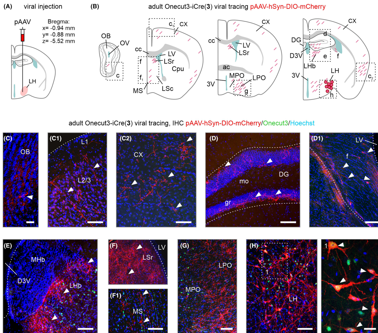
FIGURE 4 Indiscriminate viral transduction of Onecut3 + neurons in the adult lateral hypothalamus. (A) Coordinates relative to bregma to target the lateral hypothalamic area. Cre -dependent mCherry-expressing virus particles (pAAV-hSyn-DIO-mCherry) were injected to reveal efferent projections of Onecut3 + neurons. (B–H) Brain-wide mapping of mCherry + axons originating in Onecut3 + neurons of the lateral hypothalamus. Graphical rendering (B) and representative immunohistochemically images for the olfactory bulb (C), layer 2/3 of the somatosensory cortex (C 1 ), ecto/perirhinal cortex (C 2 ), the dentate gyrus (D), fimbria hippocampi (D 1 ), the lateral habenula (E), lateral and medial septal nuclei (F, F 1 ), the medial and lateral preoptic area (G) and the injection site with cell bodies (H). Arrowheads point to mCherry + fibers. 3V, 3rd ventricle; ac, anterior commissure; Cpu, caudate putamen; cc, corpus callosum; CX, cortex; DG, dentate gyrus; fi, fimbria; gr, granular layer; LHb, lateral habenula; LSc, lateral septal nucleus caudal division; LSr, lateral septal nucleus rostral division; LPO, lateral preoptic area; LV, lateral ventricle; MHb, medial habenula; mo, molecular layer; MPO, medial preoptic area; MS, medial septum; OB, olfactory bulb. Scale bars = 500 \mu m (D), 250 \mu m (E, G), 50 \mu m (C, C 1 , C 2 , F, F 1 , H), 10 \mu m (H, inset; D 1 ).
