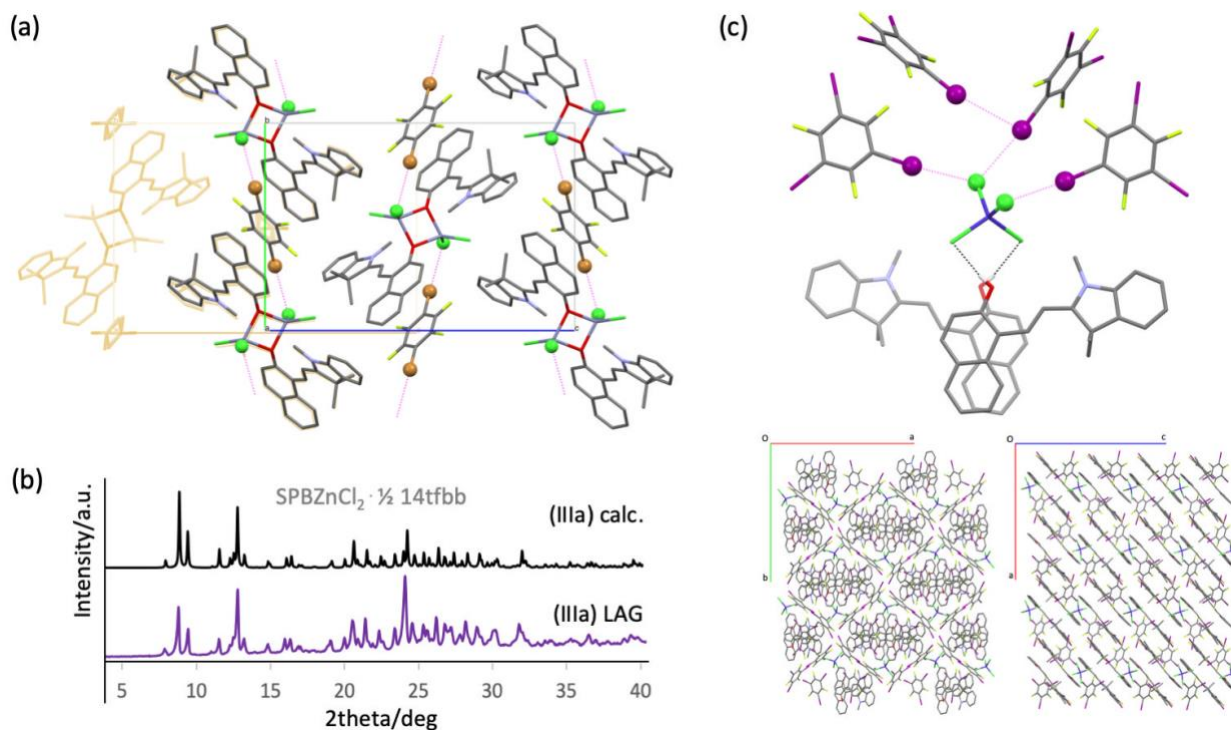
Figure 4. (a) Partial packing diagram of (IIIa) in comparison to the parent complex MCBenzZnCl 2 crystallizing with acetone. (b) Comparison of the XRPD patterns calculated from single crystal data (IIIa) and those obtained of the product by LAG. (c) Asymmetric unit of (IIIb) showing the multi-component solid formation comprised of MCBenz , [CoCl 4 ] 2- and 135tfib. Two different perspectives are highlighted below. HBs are indicated as black dashed lines and XBs in purple.
