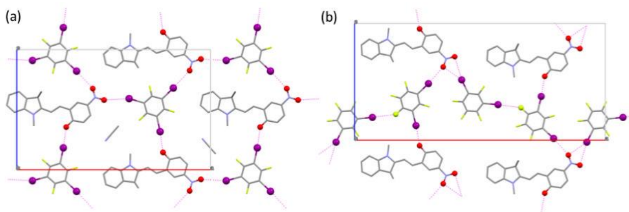
Figure 1. (a) Partial packing diagram of MCNO2 with the XB donor 135tfib (Ia) showing the cavity occupied by solvent molecules of MeCN and (b) the crystal structure of MCNO2 with 13tfib (Ib) not displaying the disordered XB donor. XBs are indicated as dashed lines.
