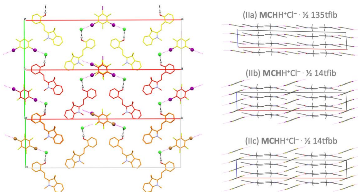
Figure 2. Left: Partial packing diagram of (IIa) yellow C-atoms, (IIb) red C-atoms and (IIc) orange C-atoms in an overlay showing each MCHH +Cl - with one XB donor connected to the Cl - ion. Right: Partial packing diagram displayed along the b -axis of (IIa)-(IIc). HBs are indicated as black dashed lines and XBs in violet.
