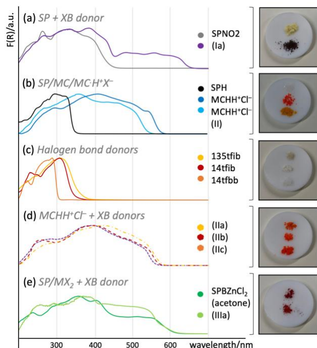
Figure 5. Diffuse reflectance spectroscopy measurements of (a) the co-crystal (Ia) of MCNO 2 with 135tfib compared to SPNO 2 (top; purple and grey curve). (b) SPH in its closed spiropyran form in comparison with the two polymorphs of the salt formed with hydrochloric acid (black and blue curves). (c) The absorption of the XB donor co-formers alone (yellow to red curves). (d) The absorption spectra of (Ia), (Ib) and (Ic) (dotted yellow to red curves) with the absorption spectra. (e) The differences between the MCBenzZnCl 2 acetone solvate and the respective crystal (IIIa) with 14tfbb replacing the acetone in the crystal unit. Photos of the bulk materials are depicted on the left of each spectral data.
