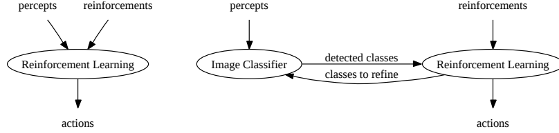
Figure 1: Comparison of information flows between “classical” Reinforcement Learning (left) and Reinforcement Learning of Visual Classes (right).
