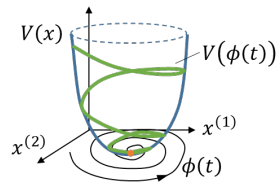
Figure 1.8: Lyapunov function V for a dynamical system \text{Sys} . The value of V (in green) along the trajectory \phi (in black) decreases as time evolves.
