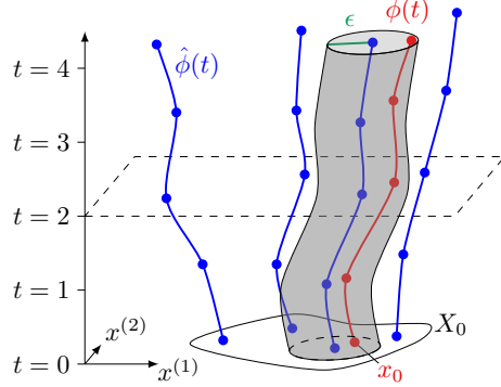
Figure 1.18: (\epsilon, 4) -spanning set \mathcal{E} (in blue) for a hybrid system HySys. Each trajectory \phi (e.g., in red) of HySys is in the \epsilon -tube around some function \hat{\phi} of \mathcal{E} for all time t \in [0, 4) .
