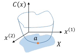
Figure 1.5: Example of a cost function that goes unbounded near the boundary of X \subseteq \mathbb{R}^2 and is zero at a single point a \in X .
