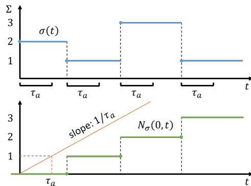
Figure 1.11: Top: Switching signal \sigma with set of modes \Sigma = \{1, 2, 3\} , and with absolute dwell time \tau_a . Bottom: Number of switches of \sigma in the interval [0, t) . The number of switches is always smaller than t/\tau_a since \sigma has absolute (and thus average) dwell time \tau_a .
