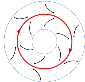
Figure 4: Example of hyperbolic system (see Example 2.9 in Subsection 2.3.3). The dynamics is unstable in the direction of the “circular flow” (red line), and is stable in the transversal direction. Consequently, the trajectories converge to the red set, but the behavior of the system on the red set is unstable.
