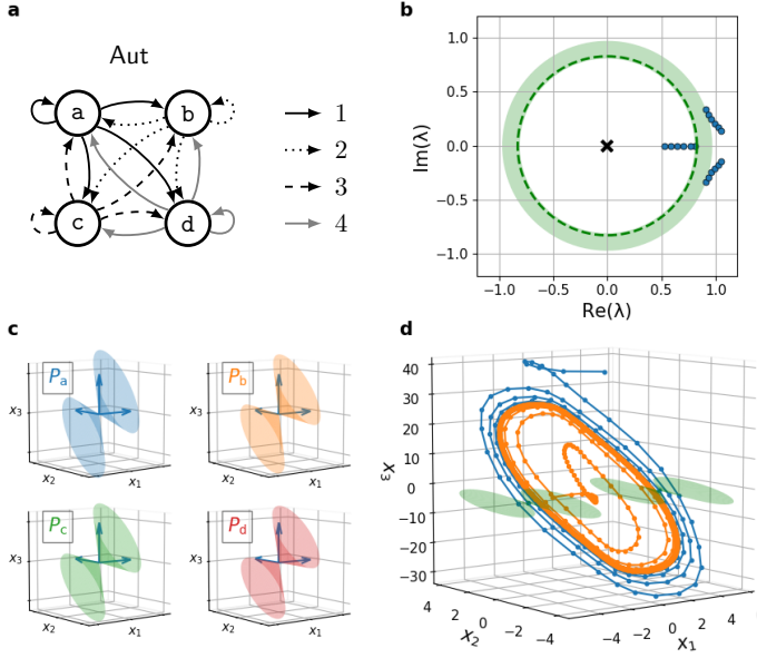
Figure 2.11: a: Automaton used to analyze the 2-dominance of Sys (the transitions are labeled according to the legend on the right). b: The blue dots represent the eigenvalues of \frac{\partial f}{\partial x}(x) for 6 randomly selected points x \in \mathbb{R}^3 . By Proposition 2.26, the value of \tilde{\gamma} must lie in the green strip. The dashed circle corresponds to the value \tilde{\gamma} = 0.83 . c: Quadratic 2-cones associated to the matrices \{P_q\}_{q \in Q} . d: Two trajectories of Sys (in blue and orange). The quadratic 2-cone associated to P_c (in green) centered at 2 different points of the \omega -limit set of the trajectory in blue does not intersect this \omega -limit set, as predicted by Proposition 2.22.
