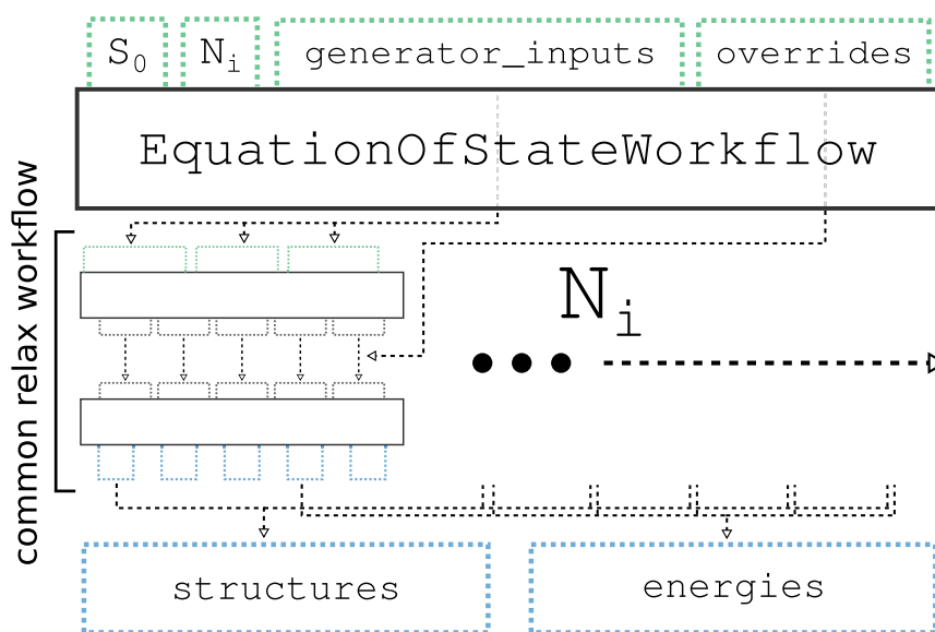
Fig. 6 Schematic diagram of the code-agnostic EOS workflow. Schematic diagram of the implementation of the code-agnostic EquationOfStateWorkflow . The EquationOfStateWorkflow takes a number of arguments: S_0 is the structure of the system at equilibrium volume and N_i are the number of volumes for which to compute the total energy. The generator_inputs will be passed directly to the inputs generator of the chosen common relax workflow implementation, which is called N_i times, once for each system volume. Note that the inset marked as “common relax workflow” corresponds directly to the schematic of the common relax workflow in Fig. 3. This highlights that the EquationOfStateWorkflow directly reuses the common relax workflow as its main building block. Which implementation of the common relax workflow is to be used is communicated to the EquationOfStateWorkflow by a single input, which is not shown for clarity. The overrides port allows an expert user to override certain inputs that are automatically determined by the generator, thus making the EquationOfStateWorkflow optionally transparent.
