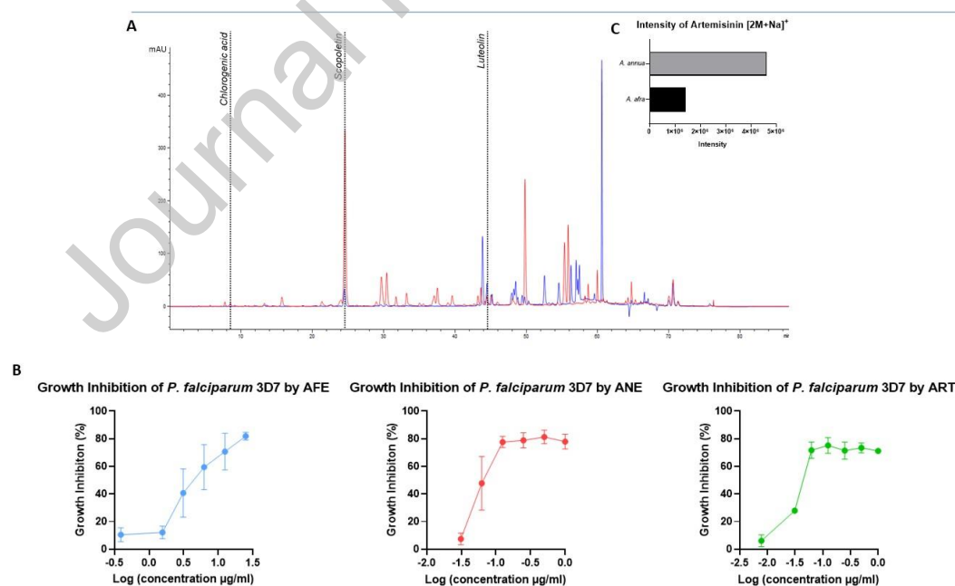
Figure 1 – A – HPLC-UV chromatograms of A. afra extract (AFA) (blue) and A. annua extract (ANE) (red) detected at 330 nm (dotted lines represent retention times of pure standards). B – Growth inhibition curves of AFE, ANE and artemisinin (ART) over 48h (error bars represent standard deviation). Results
