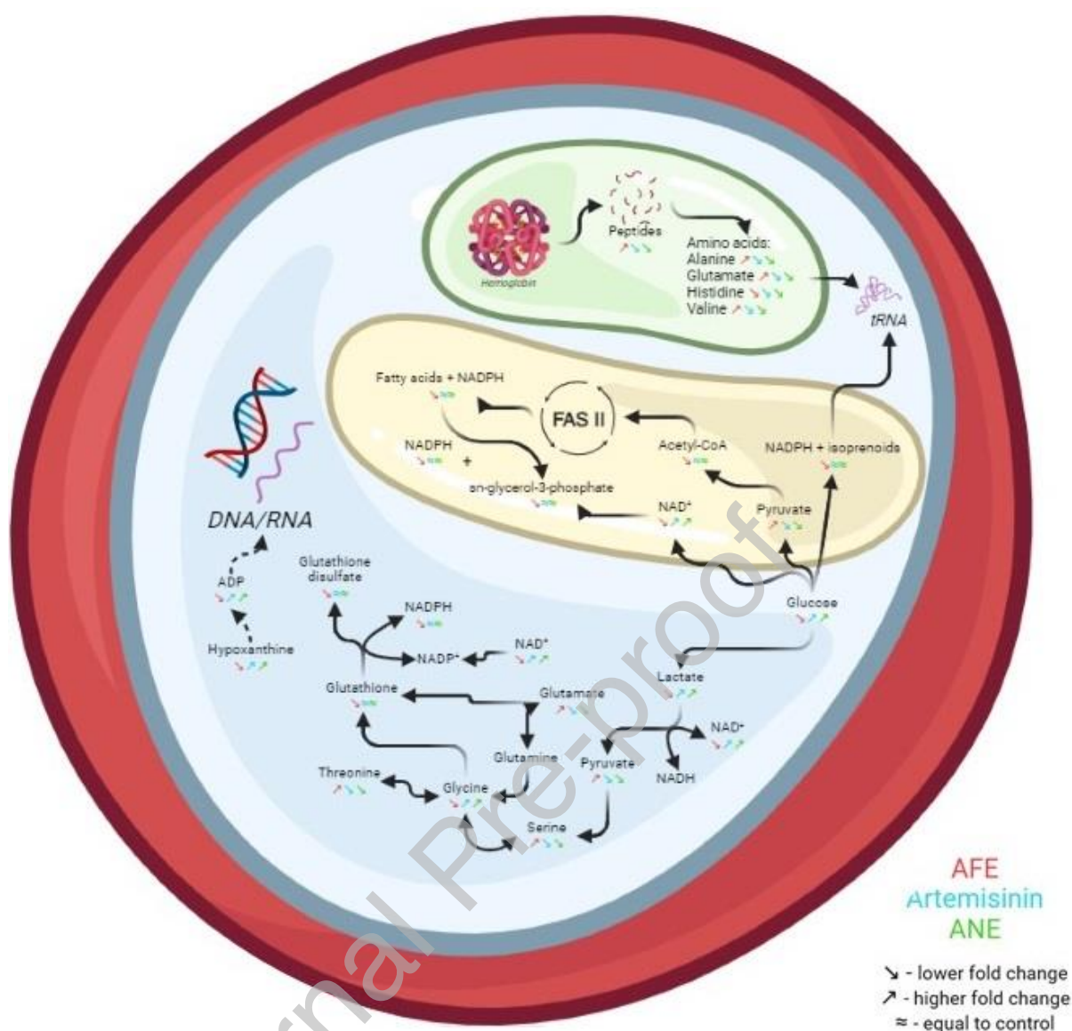
Figure 3 – Schematic view the affected pathways by AFE, ANE and artemisinin. FAS II – Fatty type II Acid Synthesis. (Arrows: red – AFE, blue – artemisinin, green – ANE; > - higher fold change, < - lower fold change, ≈ - equal to control)
