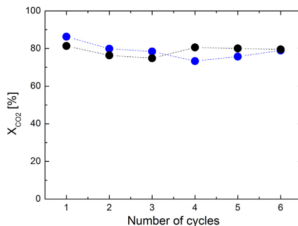
Fig. 5 – CO_2 conversion under conventional CO_2 methanation mode over 5Ni/5A (blue) and 5Ni/13X (black) at 300 °C. (For interpretation of the references to colour in this figure legend, the reader is referred to the web version of this article.)
