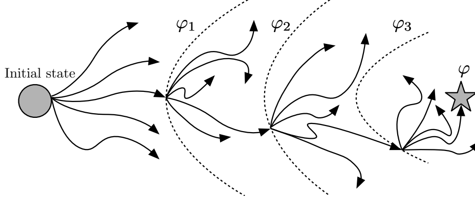
Figure 4.6. Importance splitting using three levels.
