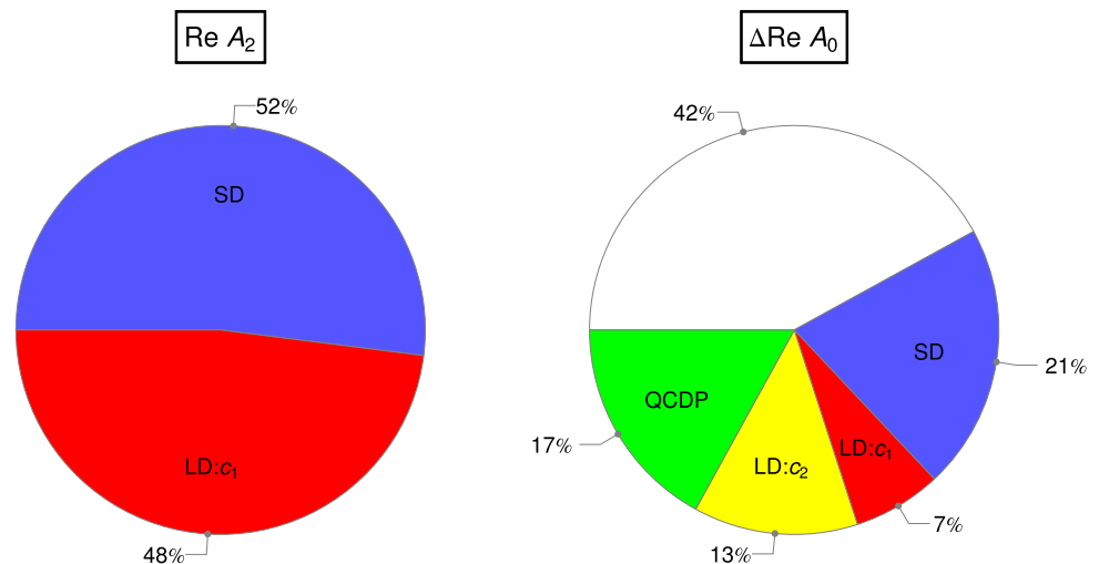
Fig. 3 Budgets for \text{Re} A_2 (left) and \Delta \text{Re} A_0 (right) summarizing the size of different suppression mechanisms of \text{Re} A_2 and enhancement mechanisms of \text{Re} A_0 , denoted here by \Delta \text{Re} A_0 , for the matching scale \mu = M = 0.8 GeV. SD stands for quark–gluon evolution and LD for meson evolution. In the case of \Delta \text{Re} A_0 we decompose LD into contributions coming from c_1 and c_2 . QC DP stands for Q_6 contribution. See text for detailed explanations
