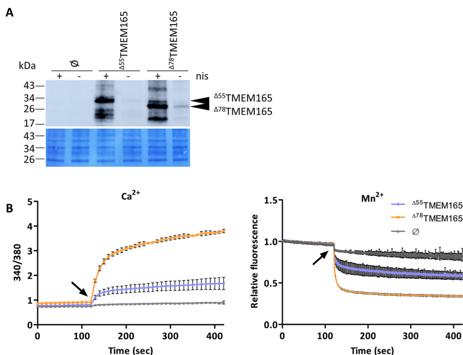
Figure 3. \text{Ca}^{2+} and \text{Mn}^{2+} transport mediated by truncated TMEM165 expressed in L. lactis . A, production of the truncated TMEM165 in L. lactis . The cells were grown to an A_{600} of 0.5 and incubated in the presence (+nis) or not (-nis) of nisin (2.5 \mu\text{g}/\text{l} ) for 2 h to induce the expression of \Delta^{55} TMEM165 or \Delta^{78} TMEM165. The tagged proteins (N terminus) were detected in membrane protein extracts by Western blotting with anti-HA antibodies. \emptyset , cells with the empty pNZ8048 vector. Coomassie Blue-stained polyvinylidene fluoride membrane was used as loading control. B, time-course measurement of the fluorescence emitted by Fura-2 in L. lactis DML1 expressing the truncated versions of TMEM165 or containing the empty pNZ8048 vector ( \emptyset ) in the presence of 75 \mu\text{M} \text{CaCl}_2 (left panel) or 75 \mu\text{M} \text{MnCl}_2 (right panel). The cells were grown to an A_{600} of 0.5, at which the truncated TMEM165 expression was initiated by addition of 2.5 \mu\text{g}/\text{l} nisin. After a 2-h postinduction time, the cells were washed and incubated for 2 h in the presence of Fura-2/AM. Left panel, time-course measurements of the ratio of the fluorescence emitted at 510 nm after excitations at 340 and 380 nm (340/380). Right panel, time-course measurements of the quenching by \text{Mn}^{2+} of the fluorescence emitted at 510 nm after excitation at 360 nm normalized to the initial fluorescence. \text{CaCl}_2 or \text{MnCl}_2 were added after 120 s of measurement (arrow), and the curves represent the means ( n = 3 \pm \text{S.D.} ).
