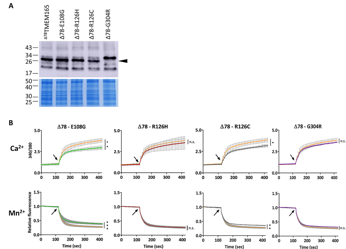
Figure 5. The impact of CDG-related mutations on the transport activity of \Delta^{78} TMEM165 in L. lactis . A , the HA-tagged proteins (N terminus) were detected in membrane protein extracts by Western blotting with anti-HA antibodies. Colloidal blue-stained gel was used as loading control. B , comparison of the fluorescence emitted during time by Fura-2 in L. lactis DML1 expressing the nonmutated \Delta^{78} TMEM165 truncated versions (orange curves) or \Delta^{78} TMEM165 containing the CDG-related mutations (indicated on the top of the graphs). The cells were treated as described in Fig. 3 B . Upper panels , time-course measurements of the ratio of the fluorescence emitted at 510 nm after excitations at 340 and 380 nm (340/380). Lower panels , time-course measurements of the quenching by Mn 2+ of the fluorescence emitted at 510 nm after excitation at 360 nm normalized to the initial fluorescence. CaCl 2 (25 \mu M) or MnCl 2 (25 \mu M) were added after 120 s of measurement (arrow), and the curves are represented as means ( n = 3 \pm S.D.). The values recorded 5 min after CaCl 2 or MnCl 2 addition were analyzed by unpaired t test. *, p < 0.05 ; **, p < 0.01 ; ***, p < 0.001 ; n.s., not significant.
