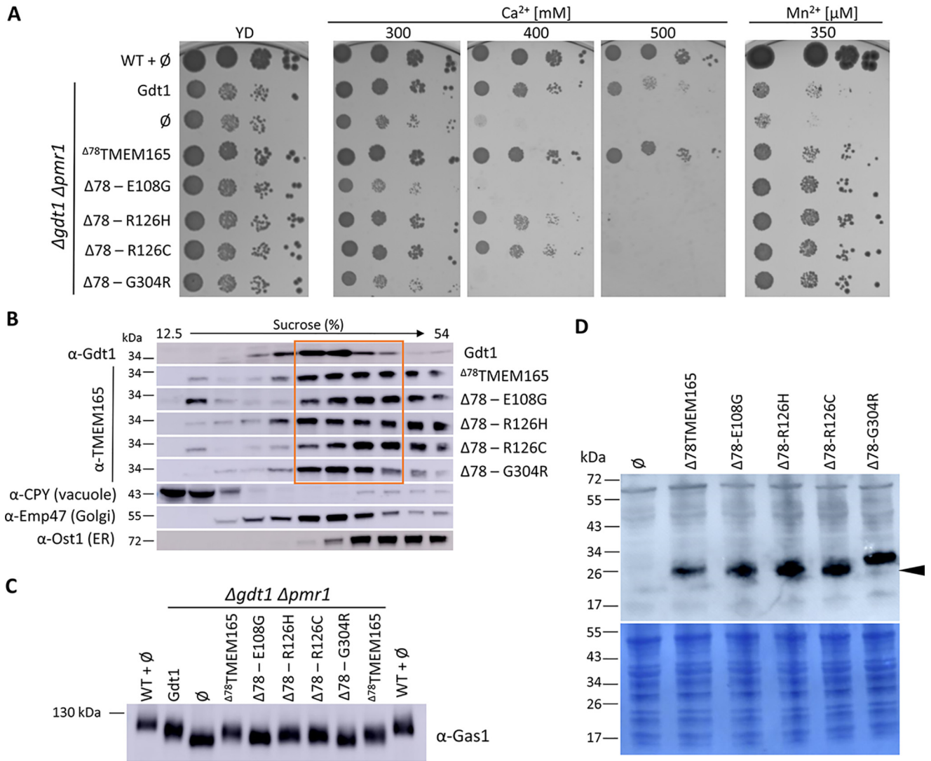
Figure 6. A, phenotypic effects of \Delta^{78} TMEM165-CDG-related mutations within gdt1\Delta pmr1\Delta strain. The gdt1\Delta pmr1\Delta strain expressed GDT1 , \Delta^{78} TMEM165 truncated version, or \Delta^{78} TMEM165 containing CDG-causing mutations. \emptyset , gdt1\Delta pmr1\Delta with the empty pRS416 vector. The cells were treated as described in the legend to Fig. 1B. B, subcellular fractionation of gdt1\Delta pmr1\Delta strain expressing GDT1 , \Delta^{78} TMEM165, or mutated \Delta^{78} TMEM165. Each strain was lysed and fractionated on a sucrose gradient. The collected fractions were analyzed by Western blotting using antibodies against Gdt1 or TMEM165 and against markers of the different subcellular compartments (CPY, Emp47, and Ost1). The distributions of the organellar markers shown here are representatives of those observed in all the strains. C, glycosylation of Gas1p. Total membrane proteins were extracted from the WT strain or gdt1\Delta pmr1\Delta strains expressing GDT1 , \Delta^{78} TMEM165 truncated version, or \Delta^{78} TMEM165 containing CDG-causing mutations. The cells were grown in MD-U supplemented with 200 mM CaCl_2 to an A_{600} of 3. The levels of Gas1p were analyzed by Western blotting with anti-Gas1 antibodies. D, production of the different TMEM165 versions in gdt1\Delta pmr1\Delta strain. Total protein extracts of cells grown in MD-U medium to an A_{600} of 3 were analyzed by Western blotting with antibodies directed against TMEM165.
