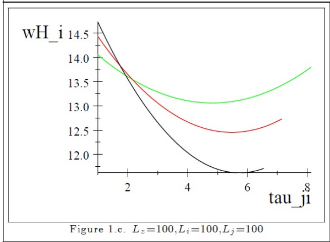
Figure A1: Simulation of impact of tariff reductions on skilled workers' wages in i .
