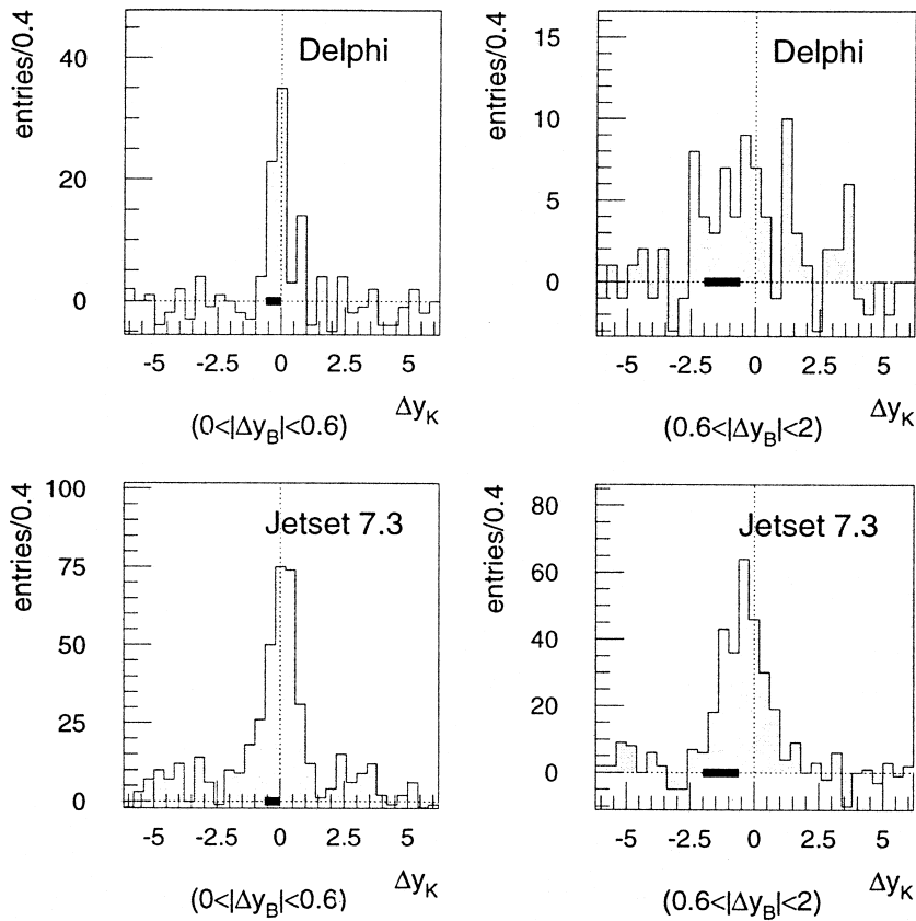
Fig. 4. Rapidity difference y_k - y_\Lambda between the kaon and the \Lambda for two ranges of the rapidity difference of the \Delta p pair. The two upper plots are obtained from the data and the two lower ones from the Delsim simulation, which contains 3.5 times more events than the data. The sign of y is chosen such that \Delta y_B = y_p - y_\Lambda would be negative. The position range of \Delta y_B is indicated as a black bar on the abscissa.
