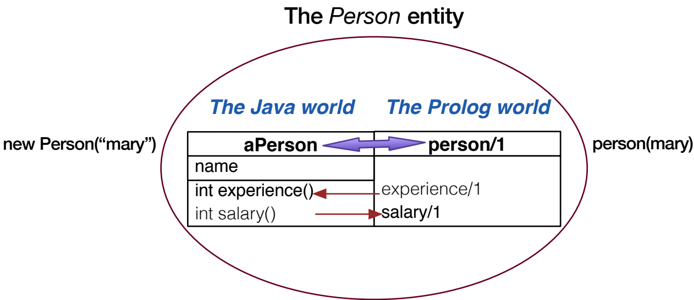
Fig 1. - A dual representation of the Person entity.
