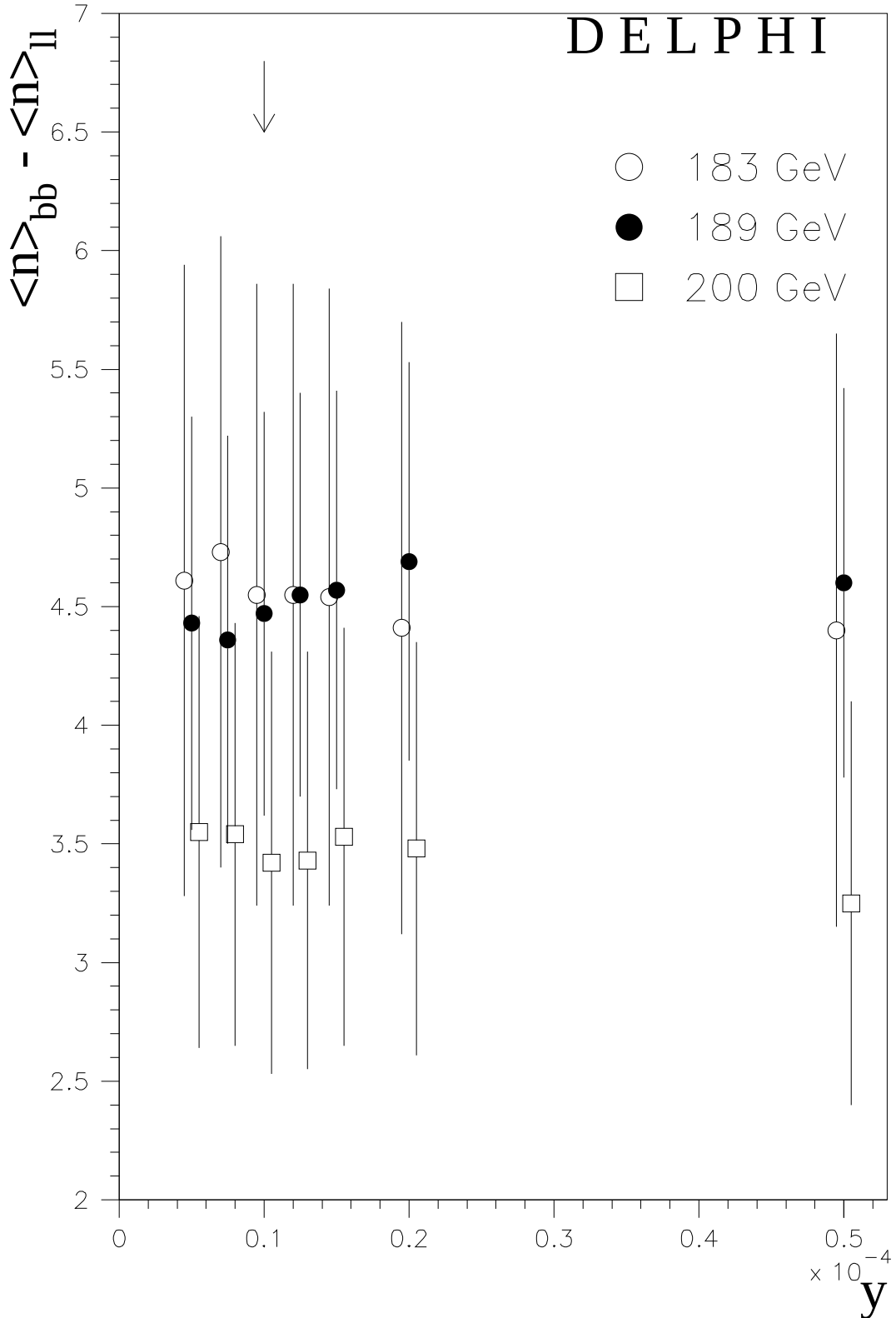
Figure 1: Stability of \delta_{bl} = \langle n \rangle_{bb} - \langle n \rangle_{ll} with respect to variations of the cut on the b-tagging variable, y . Notice that the errors in the plot are correlated (see text). The arrow indicates the value used in the analyses.
