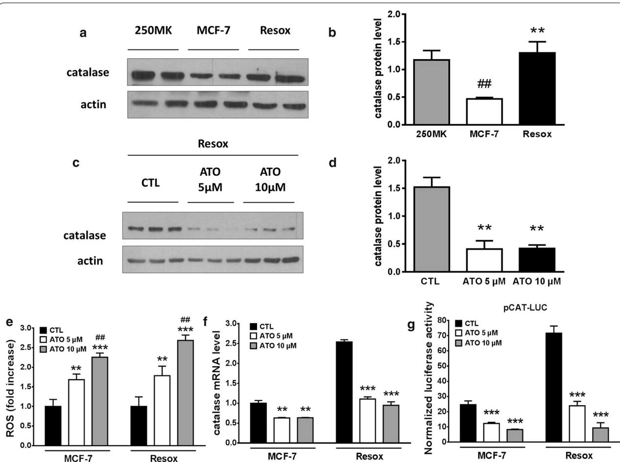
Fig. 3 Arsenic trioxide decreases catalase protein level in Resox cells by diminishing catalase gene transcription. a, b Catalase protein levels were compared and quantified in human mammary 250 MK cells, MCF-7 and Resox cells. ##p value < 0.01 versus 250MK cells. **p value < 0.01 versus MCF-7 cells. c, d Catalase protein levels were evaluated and quantified by immunoblotting in Resox cells after ATO treatment (24 h). **p value < 0.01 versus cells not incubated with ATO (CTL). ***p value < 0.001 versus cells not incubated with ATO (CTL). e ROS levels were quantified by flow cytometry with CM-H2DCFDA probe. ROS levels were compared to their respective control (CTL). **p value < 0.01; ***p value < 0.001 versus cells not incubated with ATO (CTL). f Catalase mRNA were measured by qRT-PCR and compared to untreated MCF-7 cells. **p value < 0.01; ***p value < 0.001 versus cells not incubated with ATO (CTL). g Normalized luciferase activity was measured in MCF-7 and Resox cells stably transfected with the plasmid pCAT-1518/+16 after ATO incubation for 24 h (n = 3). ***p value < 0.001 versus cells not incubated with ATO (CTL). Data are mean \pm s.e.m. Groups were compared using one-way ANOVA followed by Tukey post hoc test for ( b, d–g )
