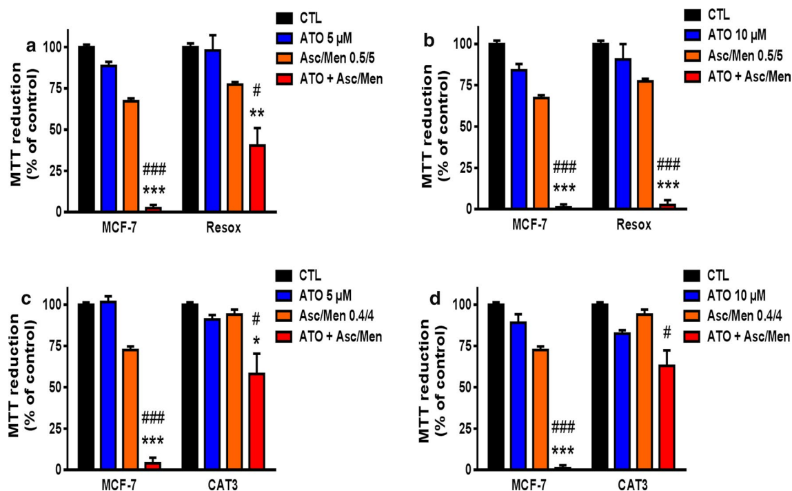
Fig. 1 Arsenic trioxide, in combination with ascorbate/menadione, enhances breast cancer cell cytotoxicity. a, b MCF-7 (from ATCC) and Resox were incubated 24 h with 5 or 10 μM arsenic trioxide (ATO) with and without Ascorbate 0.5 mM/Menadione 5 μM (Asc/Men). Cytotoxicity was evaluated by using MTT assay (n = 3). c, d MCF-7 (from ECACC) and CAT3 cells were incubated 24 h with 5 or 10 μM arsenic trioxide (ATO) with and without Asc/Men (0.4 mM/4 μM), cytotoxicity was evaluated by using MTT assay (n = 3). Data are mean ± s.e.m. Groups were compared using one-way ANOVA followed by Tukey post hoc test for ( a–d ). *p value < 0.05; **p value < 0.01; ***p value < 0.001 versus ATO. #p value < 0.05; ###p value < 0.001 versus Asc/Men
