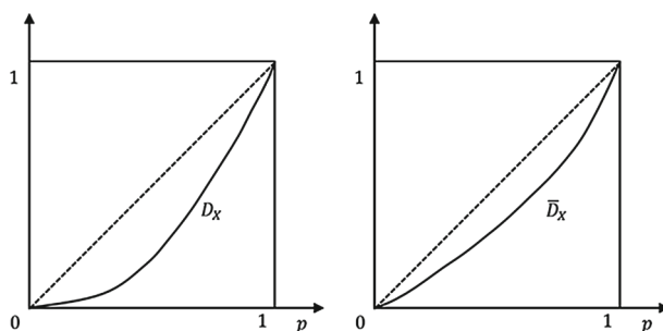
Fig. 2 The downward diagonal dependence curve D_X (left) and upward diagonal dependence curve \bar{D}_X (right) of random vector X
