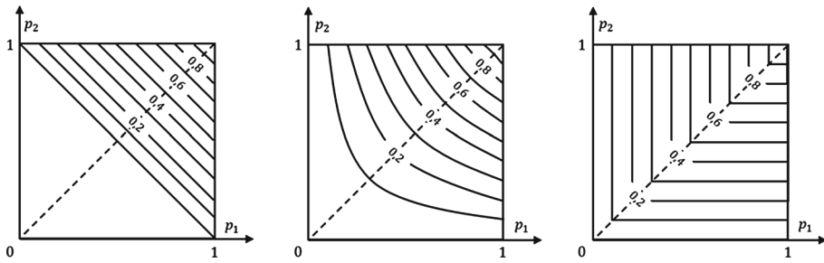
Fig. 1 Contour diagrams of C_- , C_\perp , and C_+
