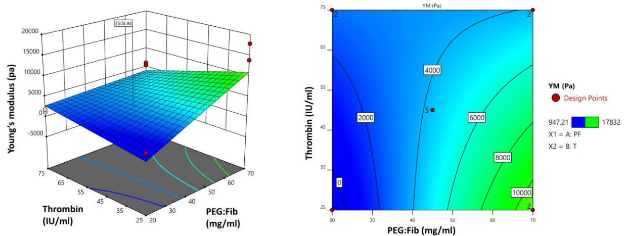
Figure 1. PEGylated fibrin Young's modulus. Response surface methodology of PEGylated fibrin hydrogel Young's modulus based on different concentrations of PEGylated fibrinogen and thrombin. Pa, Pascal; YM, Young's modulus; RSM, response surface methodology; PEG, polyethylene glycol; PF, PEGylated fibrinogen; T, thrombin.
