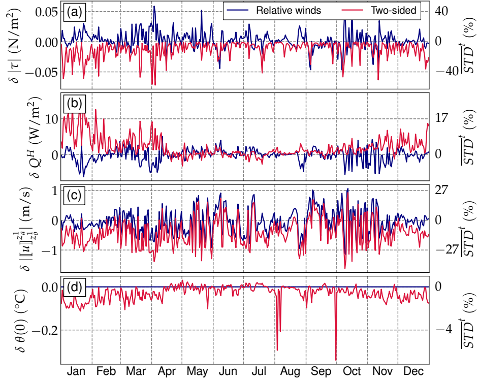
Figure 12: 2006 time series daily biases from classical relative-winds bulk closures and two-sided ones, with respect to classical absolute-winds bulk closures, at (149.25^\circ\text{E}, 36.75^\circ\text{S}) (in the Kuroshio current). (a) \delta |\tau| , (b) \delta Q^H , (c) \delta \llbracket u \rrbracket_{z_0}^{z_a^1} and (d) \delta \theta(z=0) from both closures, with the absolute-winds classical bulk closure as reference. Timewise standard deviations of absolute-winds classical bulk outputs are also given on the right scale.
