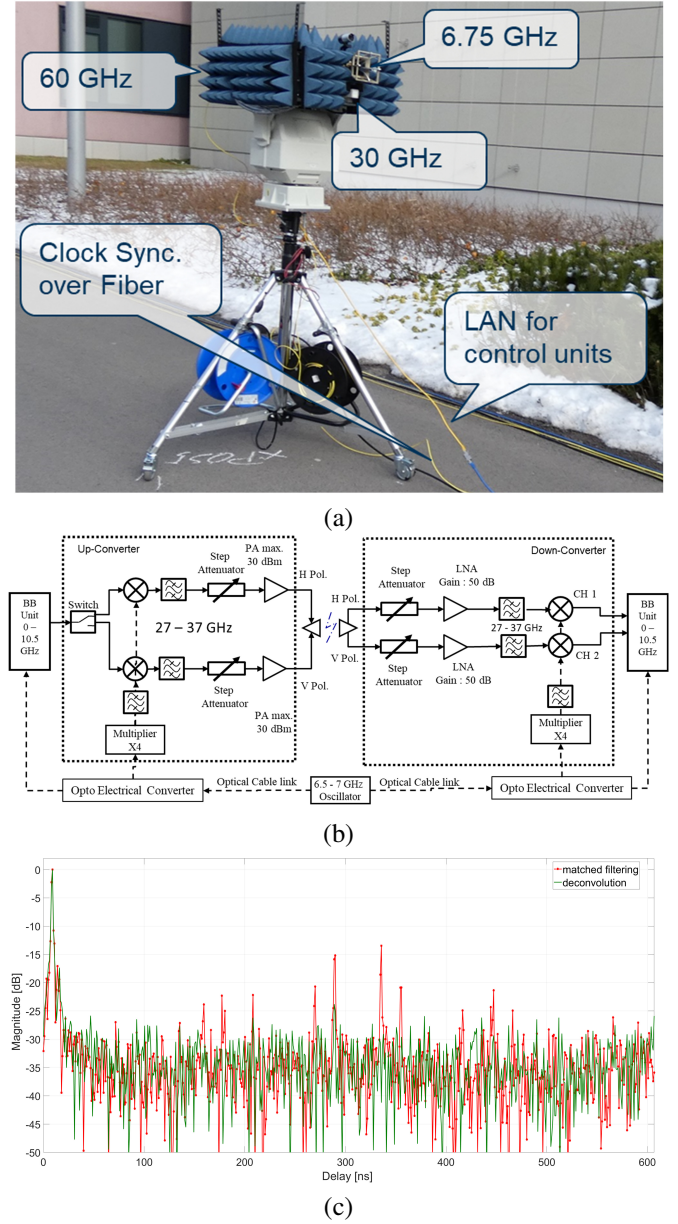
Fig. 6: TUI channel sounder. (a) Photograph. (b) Block diagram. (c) Calibration of impulse response.
