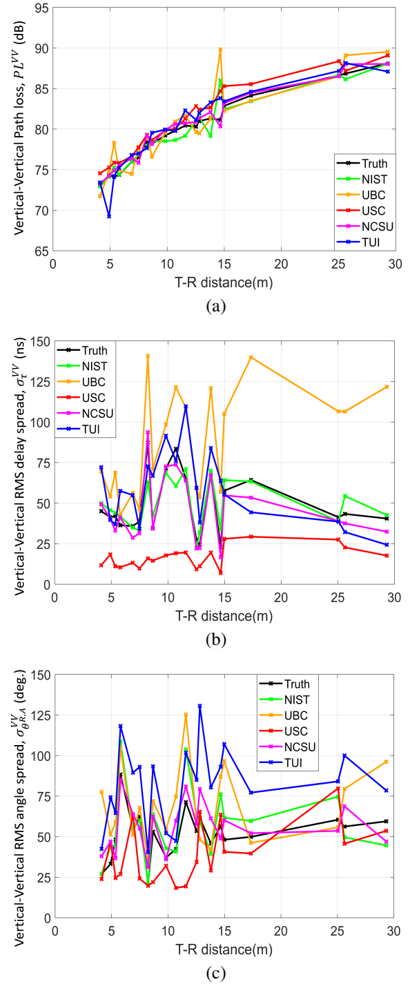
Fig. 10: Comparison of large-scale statistics estimated from five channel sounders to ground-truth statistics. (a) Vertical-Vertical Path loss (b) Vertical-Vertical RMS delay spread (c) Vertical-Vertical RMS angle spread.
