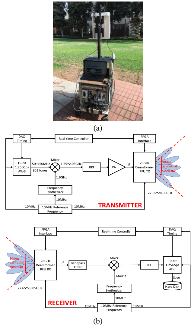
Fig. 4: USC channel sounder. (a) Photograph of RFU. (b) Block diagram.
