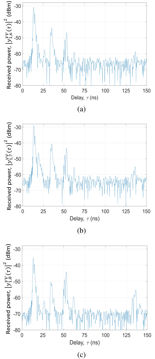
Fig. 9: Received signal y_{1j}^{VV}(\tau, \theta_1^T, \theta_j^R) at three adjacent R elements j = 6, 7, 8 generated from a ground-truth channel response applied to the system model for NIST's channel sounder.
