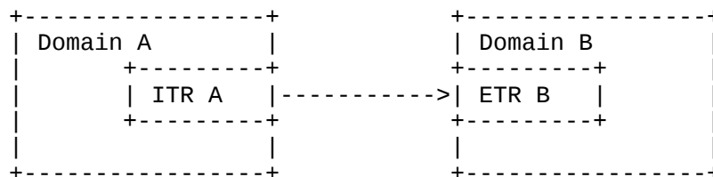
Figure 1: Unidirectional Traffic between LISP Domains
