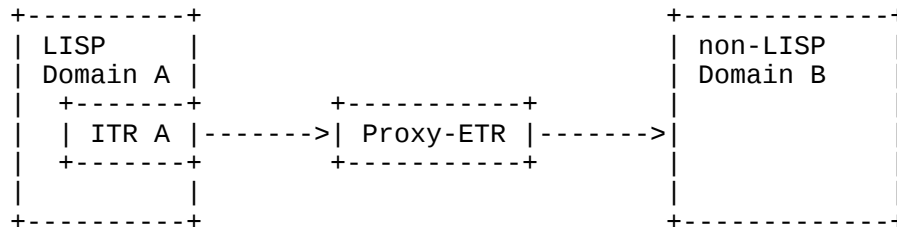
Figure 3: Unidirectional Traffic from LISP Domain to Non-LISP Domain
