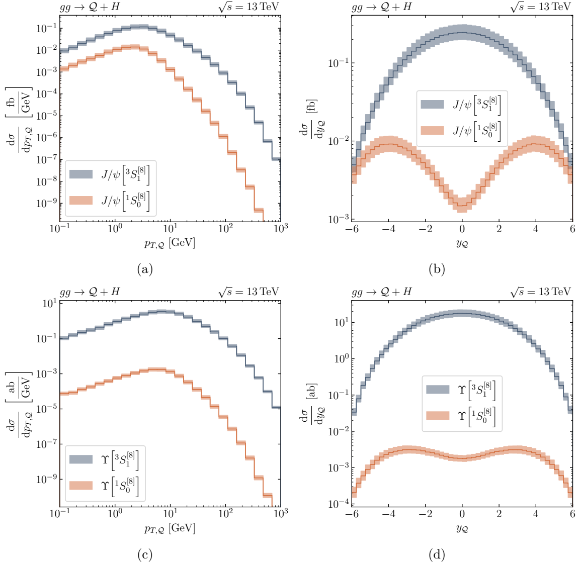
Figure 4. Transverse momentum ( p_{T,Q} ) and rapidity ( y_Q ) differential cross-section distributions for J/\psi (top) and \Upsilon (bottom) production in association with a Higgs boson H in pp collisions at \sqrt{s} = 13 TeV. The contributions from the 1S_0^{[8]} and 3S_1^{[8]} Fock states are shown in orange and blue, respectively, with the error bands representing the standard 7-point scale variation.
