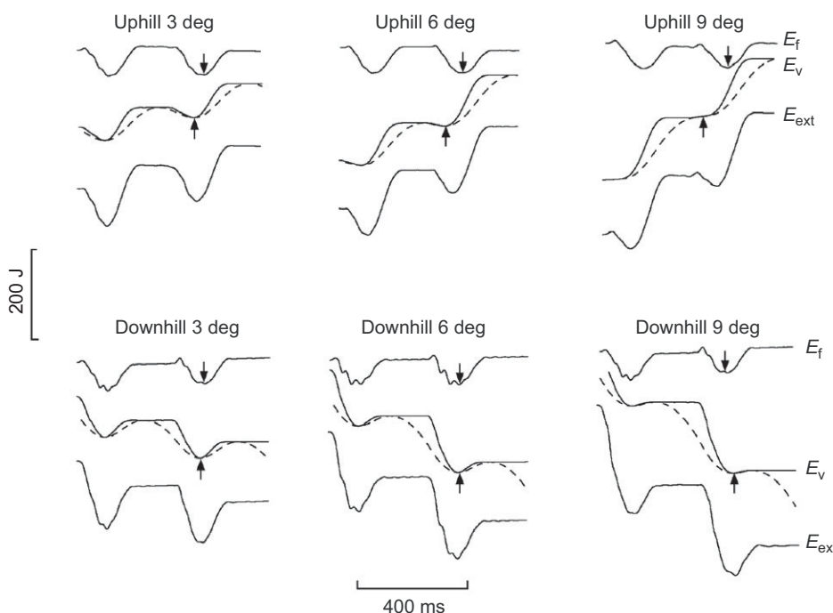
Fig. 2. Energy changes of the COM during a running stride. Mechanical energy–time curves of the COM during a stride on different slopes, while running at \sim 4.2 m s ^{-1} . In each panel, the upper curve ( E_f ) refers to the kinetic energy that is due to the forward motion of the COM, the middle curve ( E_v ) to the sum of the gravitational potential energy (interrupted line) and the kinetic energy that are due to the vertical motion of the COM, and the bottom curve ( E_{ext} = E_f + E_v ) to the total energy of the COM. The arrows pointing downwards indicate the minimum of E_f and the arrows pointing upwards the minimum of E_v during the contact phase of the second step. The horizontal segments of the energy curves correspond to the aerial phase. Tracings are from the same subject as in Fig. 1.
