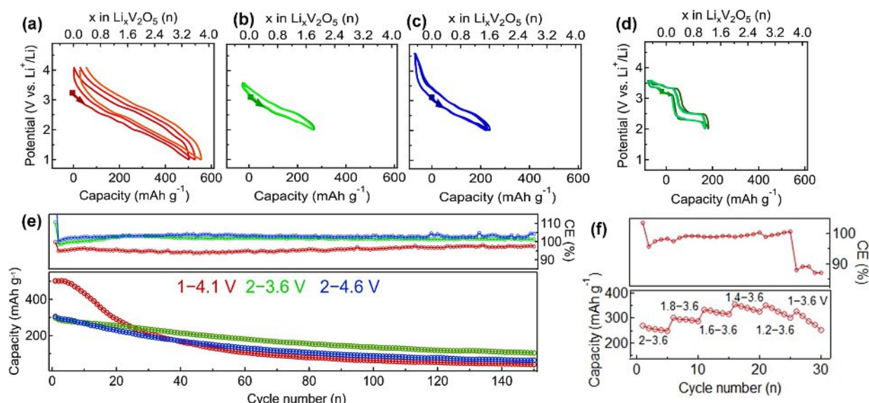
Figure 2. Galvanostatic potential versus gravimetric capacity (bottom axis) and Li-content (top axis) profiles for \text{V}_2\text{O}_5@r\text{GO} electrodes cycled in potential window of (a) 1.0–4.1 V, (b) 2.0–3.6 V; (c) 2.0–4.6 V; and (d) comparison with for \text{V}_2\text{O}_5(\text{CM}) electrode in the 2.0–3.6 V window. (e) Charge capacity and coulombic efficiency (CE) retention with cycling, at constant charge–discharge current density of 100 \text{ mA g}^{-1}_{(\text{V}_2\text{O}_5)} . (f) Coulombic efficiency and stored charge amount chart in various potential windows at charge–discharge current density of 30 \text{ mA g}^{-1}_{(\text{V}_2\text{O}_5)} .
