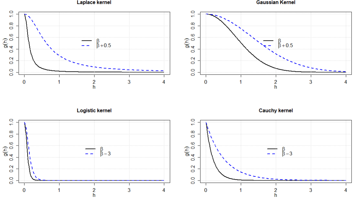
Figure 4.4: Sensitivity of kernel functions to the memory parameter \beta . The initial value of \beta for each model is in table 1.
