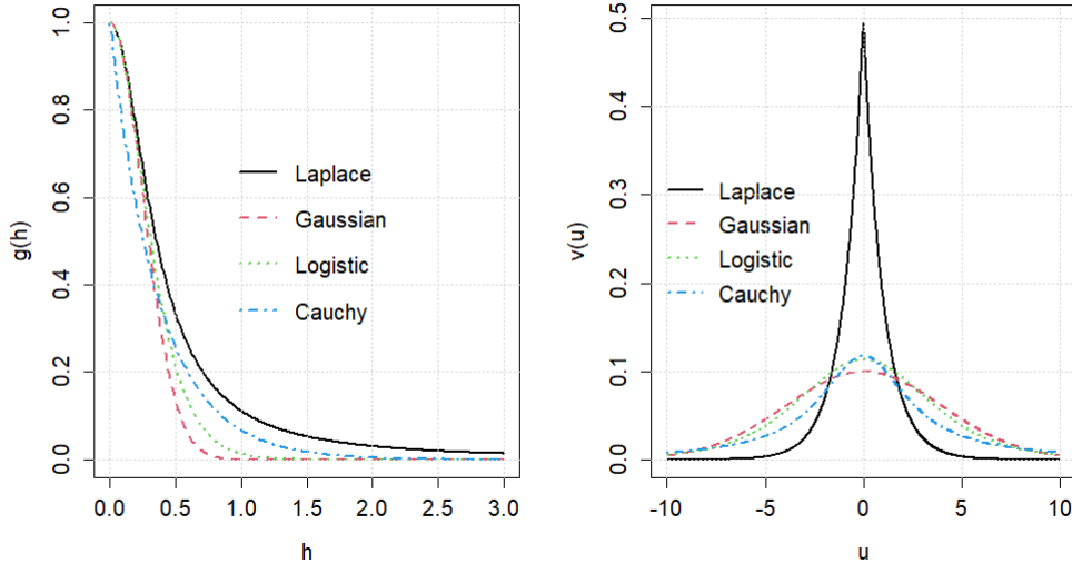
Figure 2.1: Comparison of Laplace, Gaussian and Logistic kernels for \sigma_L^2 = \sigma_G^2 = \sigma_{Log}^2 = 16 . The Cauchy kernel is computed with \beta_C = 2.71 .
