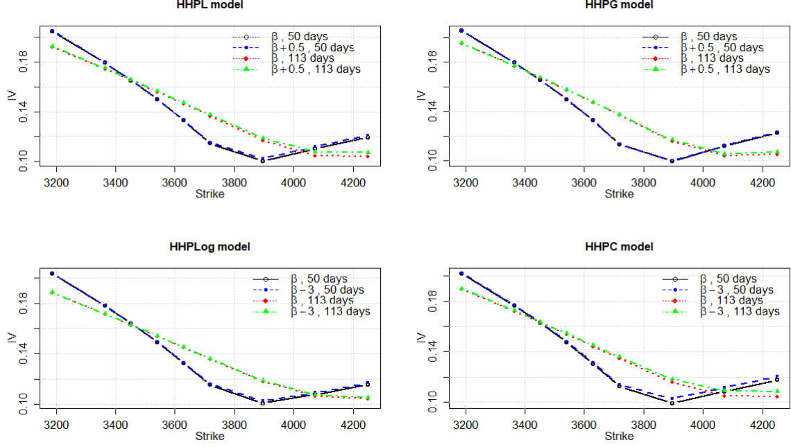
Figure 4.6: Sensitivity to the memory parameter \beta of the HHPL model. Model parameters used are in table 1.
