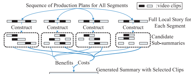
Fig. 6. A resource allocation based framework of sport video summarization.
