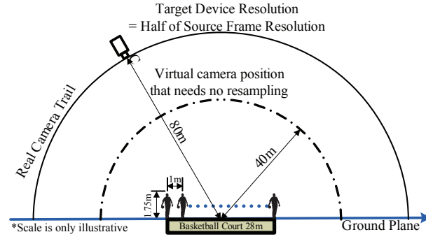
(a) A sandbox case for investigating the criterion
