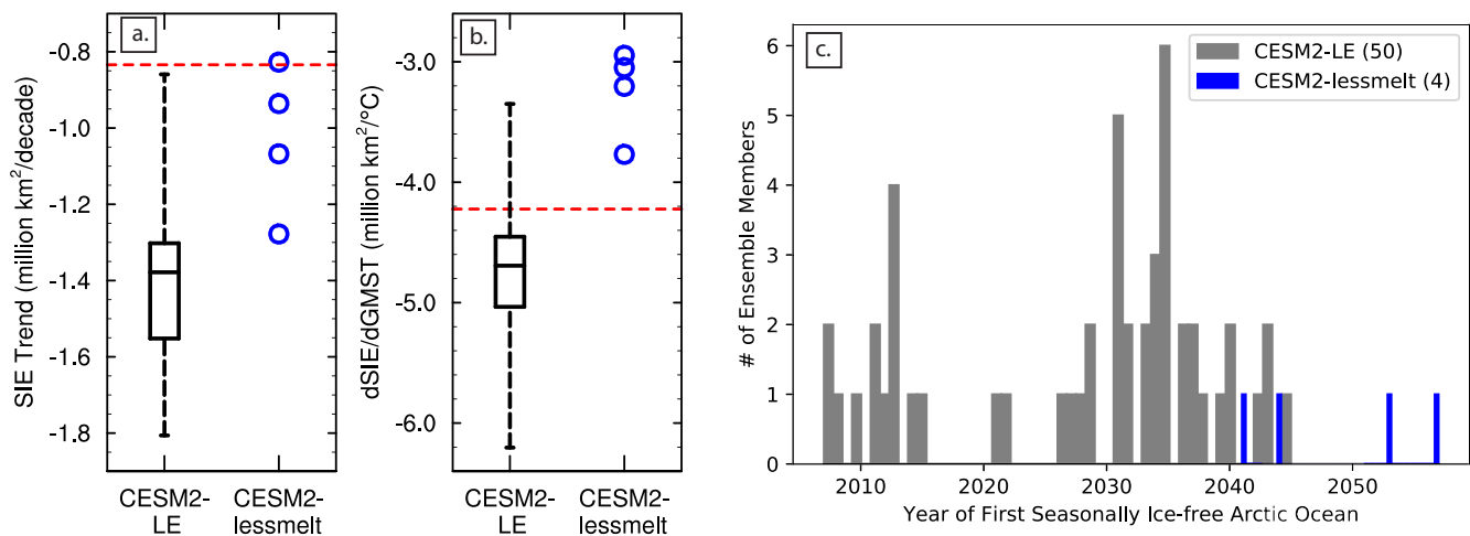
Figure 11. Arctic sea ice comparison metrics: (a) September sea ice trends, (b) sea ice sensitivity defined as the change in September sea ice extent per degree of change in global mean surface temperature ( dSIE/dGMST ), and (c) year of first seasonally ice-free Arctic Ocean. Sea ice extent trend and sensitivity calculations follow protocol and years (1979–2014) used for evaluation of CMIP6 by Notz and SIMIP Community (2020). In (a and b), the observations are shown as a red dashed line and the CESM2 Large Ensemble is shown as a box indicating the interquartile range, a line inside the box indicating the median, and whiskers to show the minimum and maximum across all ensemble members. In (c), a seasonally ice-free Arctic Ocean occurs when the September sea ice extent first falls below 1 million sq. km.
