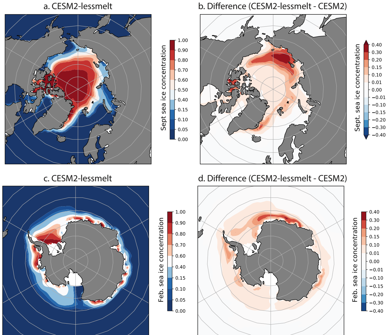
Figure 2. Late summer sea ice concentration in preindustrial control runs: (a) September Arctic CSM2-lessmelt, (b) Difference September Arctic (CSM2-lessmelt—CESM2), (c) February Antarctic CSM2-lessmelt, and (d) Difference February Antarctic (CSM2-lessmelt—CESM2). Values are overlapping 200-year averages as in Figure 1. Note: Nonlinear color scale used to emphasize low ice concentrations.
