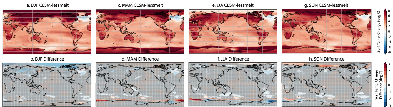
Figure 14. Ensemble mean surface temperature change (2080–2099 minus 1920–1939) by season: (a) DJF CESM2-lessmelt, (b) DJF Difference (CESM2-lessmelt minus CESM2-LE), (c and d) as in (a and b) but for MAM, (e and f) as in (a and b) but for JJA, (g and h) as in (a and b) but for SON. Stippling on difference maps indicates where differences between CESM2-lessmelt and CESM2-LE ensemble means are *not* statistically significant at the 95% confidence level.
