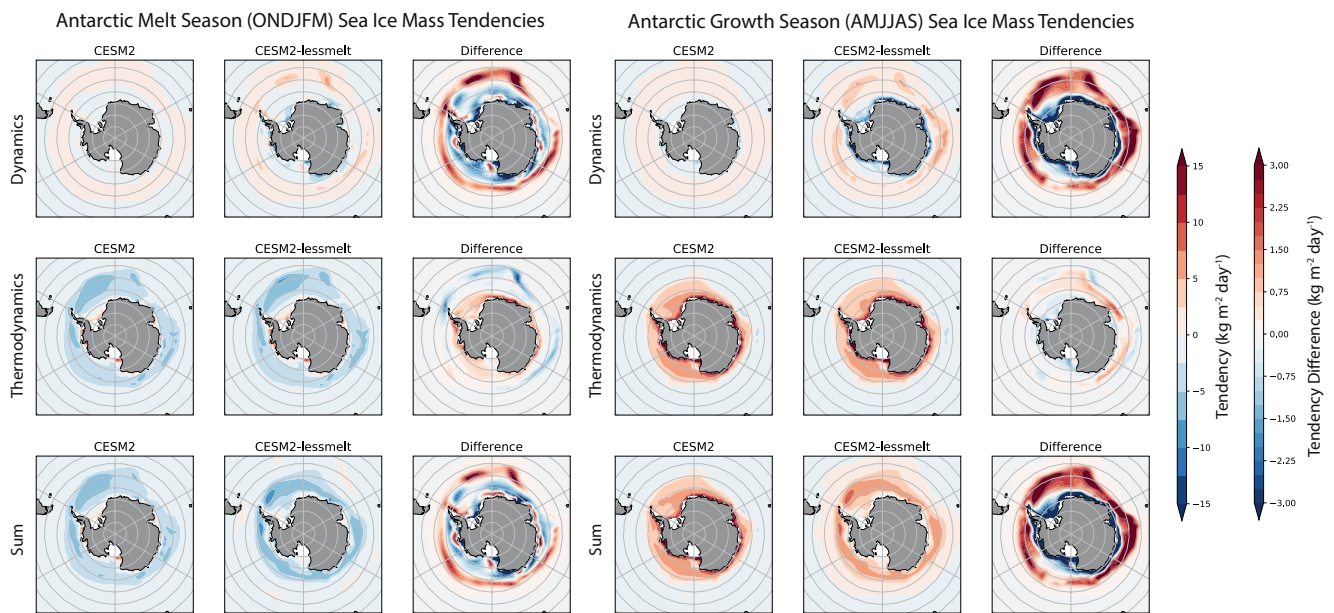
Figure 6. Antarctic sea ice mass tendency terms for the melt season [ONDJFM] (left), and the growth season [AMJJAS] (right). For each season, the top row is tendency due to dynamics (sidmassdyn), the middle row is tendency due to thermodynamics (sidmassst), and the bottom row is their sum. All differences are CESM2-lessmelt minus CESM2. Values are overlapping 200-year averages as in Figure 1.
