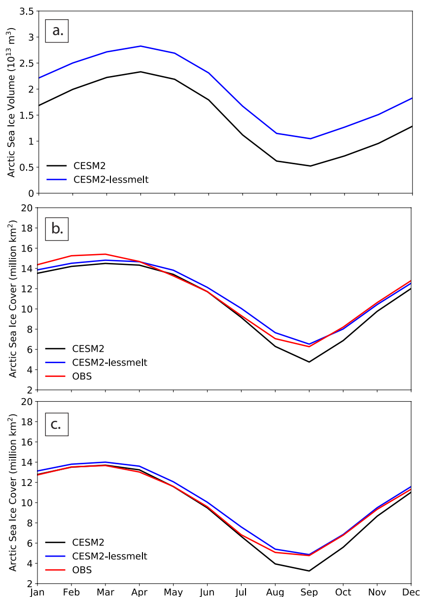
Figure 8. Present-day (1979–2014) ensemble mean seasonal cycle in CESM2-LE and CESM2-lessmelt: (a) Arctic sea ice volume, (b) Arctic sea ice extent, and (c) Arctic sea ice area. Observations are from NSIDC sea ice index with pole filling (Fetterer et al., 2017).
