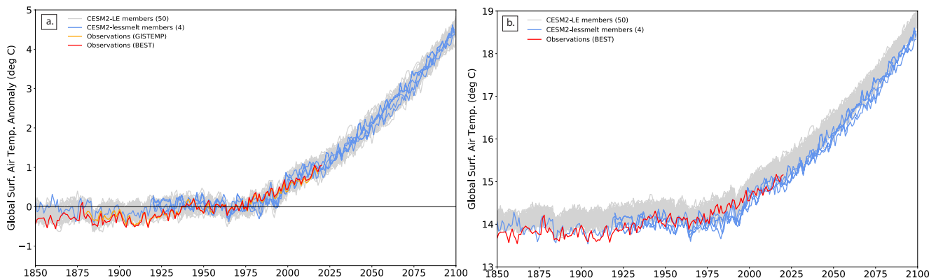
Figure 13. Transient evolution global annual mean surface air temperature in CESM2-LE and CESM2-lessmelt: (a) anomaly from 1951 to 1980 and (b) absolute value. Observations are from GISTEMP (Hansen et al., 2010) and BEST (Rohde & Hausfather, 2020).
