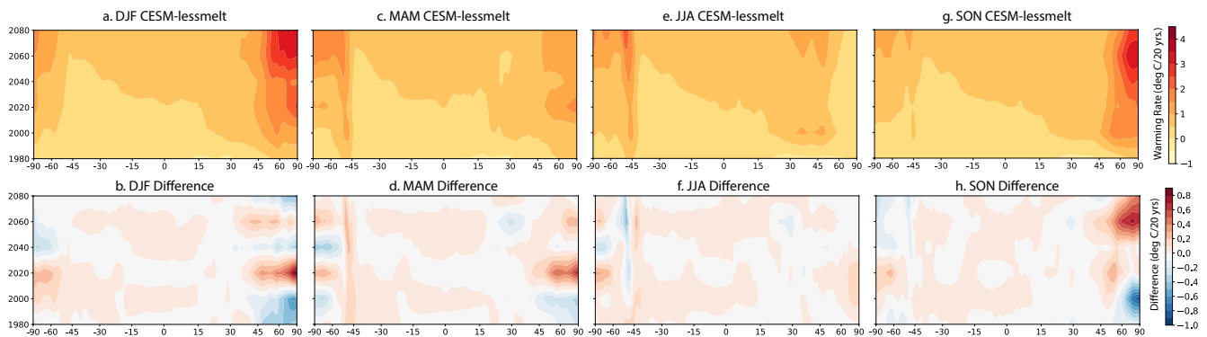
Figure 15. Zonal ensemble mean surface warming rate (deg C/20 years) by season: (a) DJF CESM2-lessmelt, (b) DJF difference (CESM2-lessmelt minus CESM2-LE), (c and d) as in (a and b) but for MAM, (e and f) as in (a and b) but for JJA, (g and h) as in (g and h) but for SON. Warming rates are calculated using 20 years and the start year plotted on the vertical axis.
