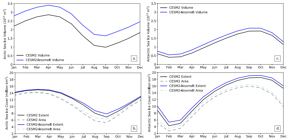
Figure 1. Seasonal cycle in CESM2 and CESM2-lessmelt 1850 preindustrial control runs: (a) Arctic sea ice volume, (b) Arctic sea ice area and extent, (c) Antarctic sea ice volume, and (d) Antarctic sea ice area and extent. Values are overlapping 200-year averages (years 911–1110 of the CESM2 CMIP6 1850 pre-industrial control run).
