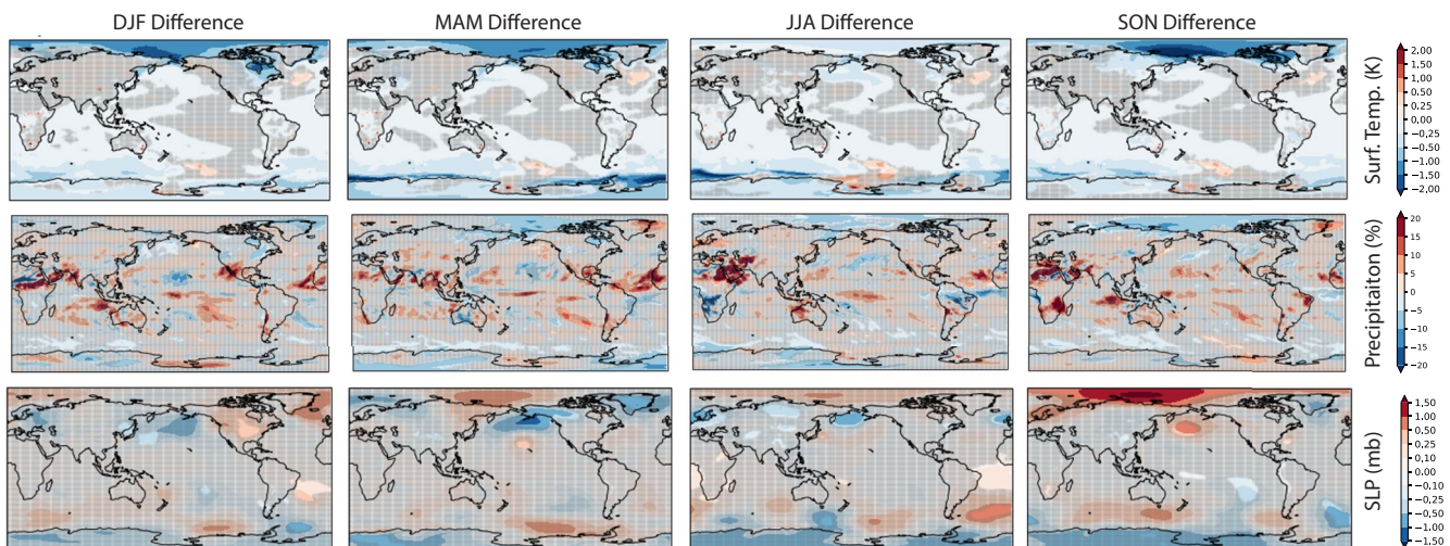
Figure 7. Global maps of pre-industrial control differences (CESM2-lessmelt minus CESM2) by season. Top row shows surface temperature (K). Middle row shows total precipitation (% difference). Bottom row shows sea level pressure (mb). Gray stippling shows regions that are not statistically different at the 95% confidence level using a 2-sided t -test. Values are overlapping 200-year averages as in Figure 1.
