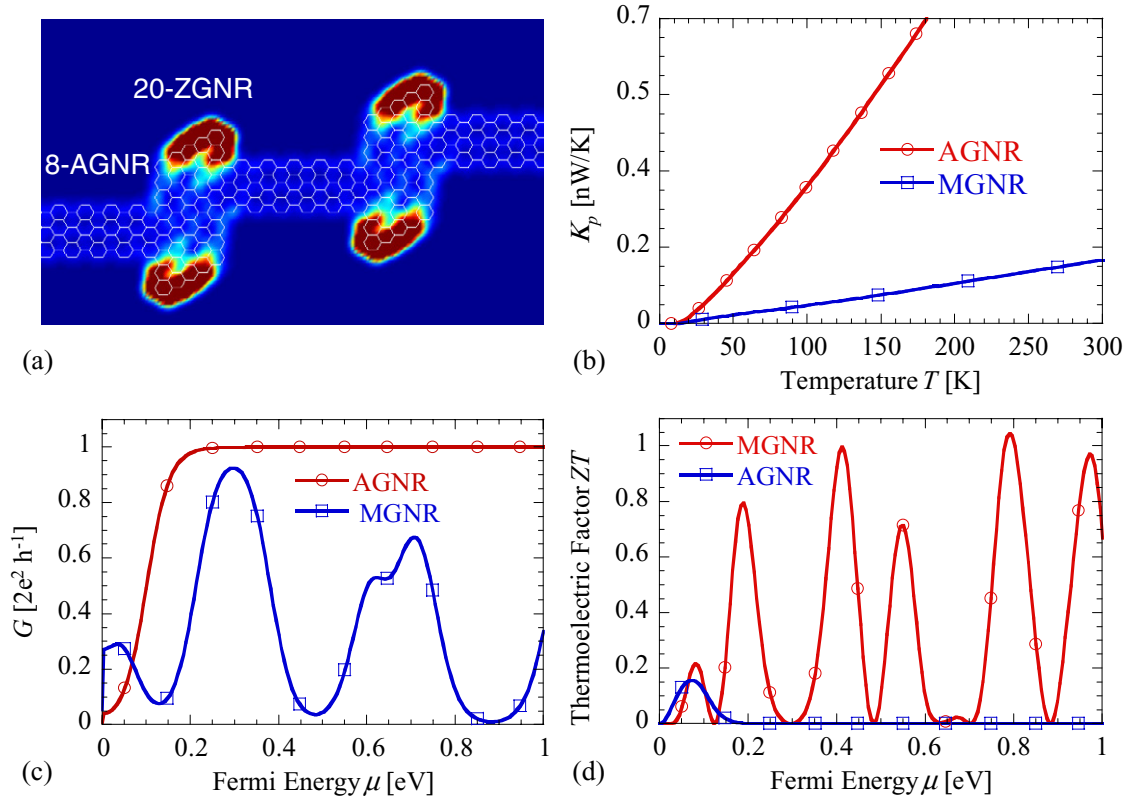
Figure 5. (a) MGNR consisting of alternating 8-AGNR and 20-ZGNR sections, and local DOS at energy E = 0.05 eV. Red and blue areas correspond to high and low DOS, respectively. (b) Phonon contribution to the thermal conductance as a function of temperature in MGNR and 8-AGNR. (c) Electronic conductance and (d) figure of merit ZT as a function of chemical potential in both GNRs at room temperature. Further details in [98].
