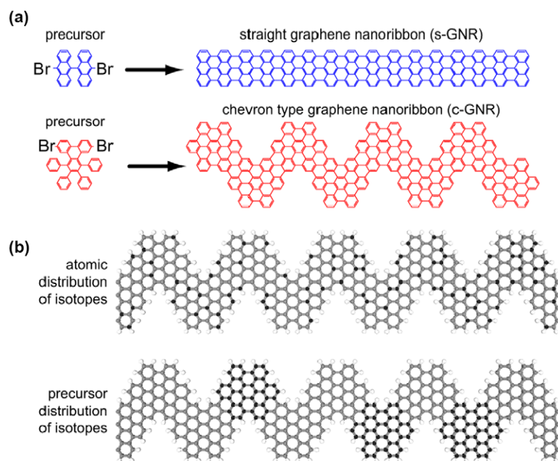
Figure 6. Structural aspects and isotope distribution types of bottom-up fabricated GNRs. (a) Structures of precursors and corresponding straight and chevron type GNRs, s-GNR and c-GNR. (b) Heavy isotopes can be distributed at the atomic or precursor level. Grey, ^{12}\text{C} ; black, ^{14}\text{C} ; white H. Reproduced with permission [134]. Copyright 2013, Nature Publishing Group.
