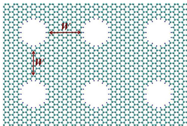
Figure 9. A typical H-passivated GNM system. Here the big cyan (small blue) spheres represent C (H) atoms, and W denotes the neck width along the zigzag and armchair directions. Reproduced with permission [147]. Copyright 2012 by the American Physical Society.
