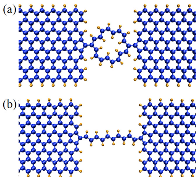
Figure 8. Schematic view of (a) ZGNR|18-annulene|ZGNR and (b) ZGNR|C10|ZGNR single-molecule nanojunctions. The contact between the source and the drain 8-ZGNR (consisting of eight zigzag chains) metallic electrodes and molecules is made via five-membered rings of carbon atoms (dark blue). The hydrogen atoms (light yellow) are included to passivate the edge carbon atoms in the nanoribbon or dangling bonds in the molecules. The distance between ZGNR electrodes is d = 1.29 nm for the device in panel (a) and d = 1.59 nm for the device in panel (b). Reproduced with permission [99]. Copyright 2012, Springer.
