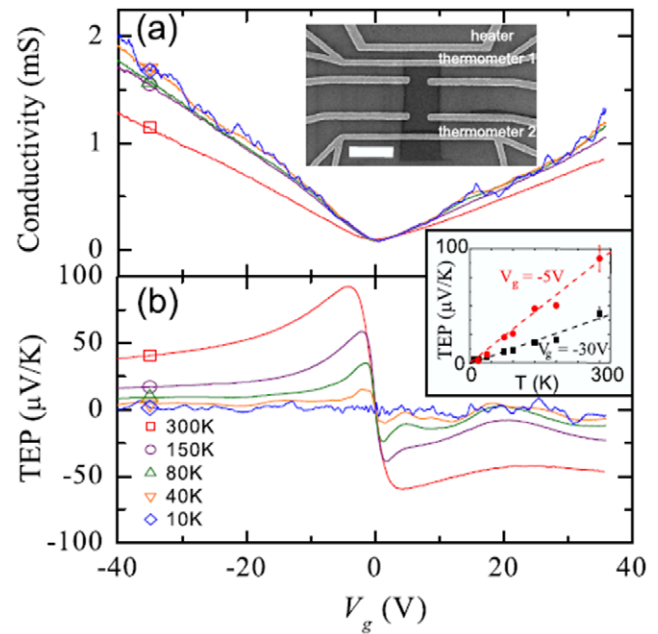
Figure 1. (a) Electrical conductivity and (b) TEP of a graphene sample as a function of V_g for T = 300\text{ K} (square), 150\text{ K} (circle), 80\text{ K} (up triangle), 40\text{ K} (down triangle), and 10\text{ K} (diamond). Upper inset: scanning electron microscopy image of a typical device. The scale bar is 2\text{ }\mu\text{m} . Lower inset: thermopower values taken at V_g = -30\text{ V} (square) and -5\text{ V} (circle). Dashed lines are linear fits to the data. Reproduced with permission [66]. Copyright 2009 by the American Physical Society.
