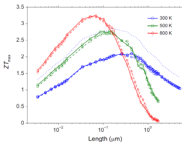
Figure 7. Maximum ZT as a function of length at different temperatures in structures schematized in figure 6. Maximum ZT achievable when Anderson type disorder is introduced in the electronic Hamiltonian. The variation of onsite energies are set equal to the temperature, \sigma = k_B T . Solid lines represent hole-like transport while the dashed lines are for electron-like particles. The ZT_{\text{max}} values shown are realized inside the band gap, i.e. |\mu| < 0.75 \text{ eV} with respect to the mid-gap, except for the dotted curve ( T = 300 \text{ K} ) when |\mu| > 1 . Reproduced with permission [134]. Copyright 2013, Nature Publishing Group.
