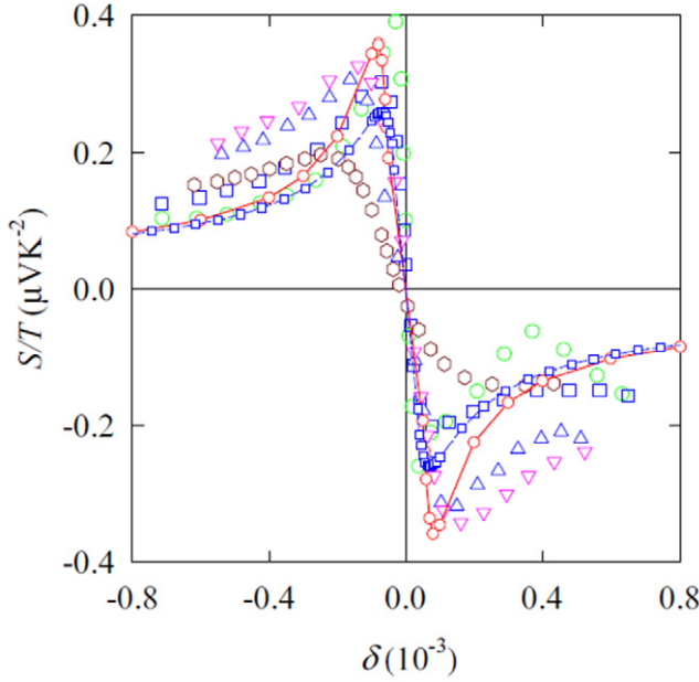
Figure 3. Linear- T dependence coefficient S/T of TEP as a function of the electron doping concentration \delta . The present calculations (red solid line with circles for renormalized \mu and the blue dashed line with squares for \mu = E_F ) are compared with the experimental data in [66] (circles at T = 150 K and squares at T = 300 K), [67] (hexagons at T = 255 K), and [68] (up triangles at T = 160 K and down triangles at T = 280 K). Reproduced with permission [80]. Copyright 2009 by the American Physical Society.
