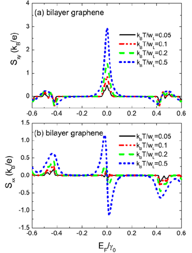
Figure 4. Thermopower S_{xx} and Nernst signal S_{xy} as functions of the Fermi energy in bilayer graphene and at different temperatures. The system size is taken to be N = 96 \times 48 \times 2 , with magnetic flux \varphi = 2\pi/48 , and disorder strength r_s = 0.3 (uniformly distributed positively and negatively charged impurities are considered within this strength) with W_L/\gamma_0 = 0.0376 . Reproduced with permission [89]. Copyright 2011 by the American Physical Society.
