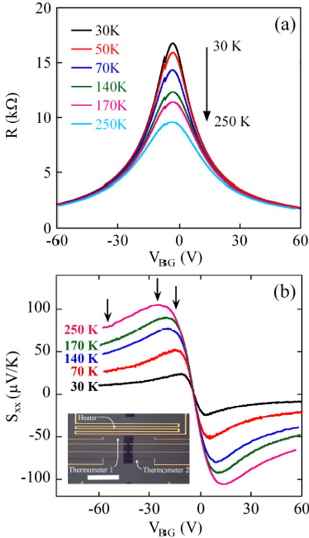
Figure 2. Thermoelectric measurements in bilayer graphene. (a) Two-terminal resistance R and (b) thermopower as a function of the backgate voltage V_{BG} in zero magnetic field and at various temperatures: T = 30, 50, 70, 140, 170 , and 250 K. Inset: optical image of a typical device. Size of the scalebar is 30 nm. Reproduced with permission [70]. Copyright 2010 by the American Physical Society.
