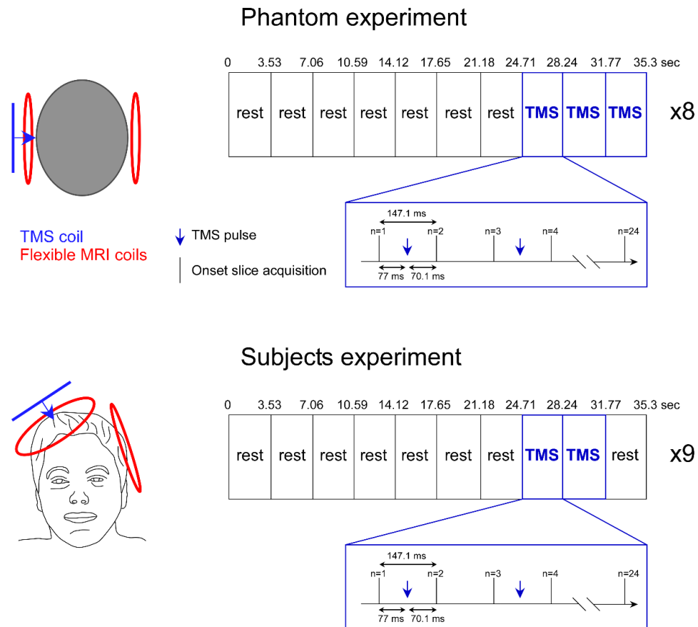
Figure 6.1. Experimental design. The experiments were carried out on a cylindrical phantom, the MRI-compatible figure-of-eight coil was placed at the center of a flexible MRI coil. A second identical MRI coil was positioned on the other side of the phantom. Biphasic TMS pulses at 80% of the maximum stimulator output (MSO) were delivered every two slices with a waiting period of 70 ms before the onset of the acquisition of the next slice. TMS pulses were delivered after a period of 77 ms corresponding to the time required for data readout. The inter-slices interval was kept constant across volumes and set at 147.1 ms. Each volume (TR = 3530 ms) included 24 slices
