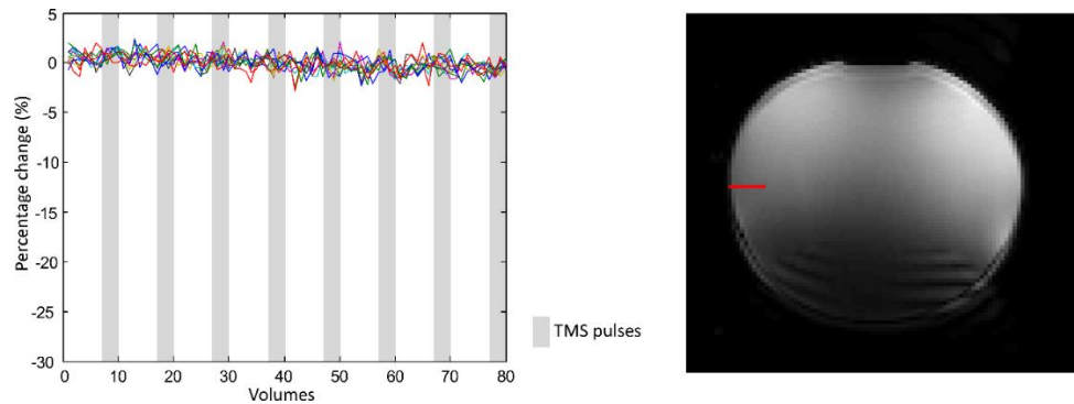
Figure 6.6. Percentage of signal change in a line of voxels in front of the TMS coil (slice 12), from the closest to the surface, to 10 voxels deeper (red line). Gray rectangles indicate when the TMS pulses were delivered. This graph shows that no systematic signal change was induced by TMS confirming that dynamic imaging artifacts were absent.
