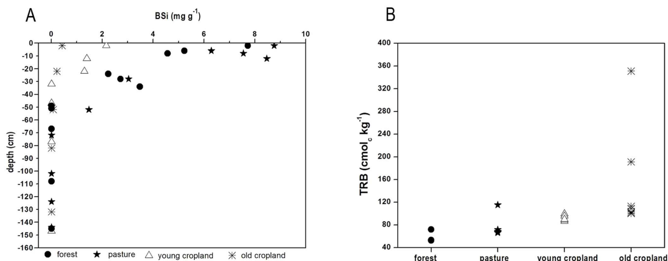
Figure 2 | (a) Scatterplot of biogenic silica (BSi) in mg g -1 dry soil in the soil profile, (b) Total Reserve in Bases (TRB = [Na] + [Mg] + [Ca] + [K]) weathering index calculated on dry soil, in cmol charge kg -1 . Sites are represented by symbols: Ronquières (circles), Blégny (stars), Ganspoel (triangle) and Velm (crosses). Multiple symbols within a site in (b) represent different TRB values calculated from positions and depths along the slope in every site for which soil water DSi \delta^{30}\text{Si} are available, i.e. 3 in forests, 6 in pasture, 5 in young cropland and 7 in old cropland (See supplementary information for details).
