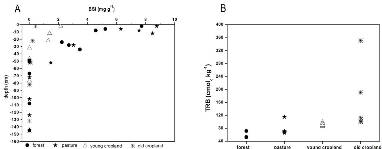
Figure 1 | (a) Scatterplot of biogenic silica (BSi) in \text{mg g}^{-1} dry soil in the soil profile, (b) Total Reserve in Bases ( \text{TRB} = [\text{Na}] + [\text{Mg}] + [\text{Ca}] + [\text{K}] ) weathering index calculated on dry soil, in \text{cmol charge kg}^{-1} . Sites are represented by symbols: Ronquières (circles), Blégny (stars), Ganspoel (triangle) and Velm (crosses). Multiple symbols within a site in (b) represent different TRB values calculated from positions and depths along the slope in every site for which soil water \text{DSi } \delta^{30}\text{Si} are available, i.e. 3 in forests, 6 in pasture, 5 in young cropland and 7 in old cropland (See supplementary information for details).
