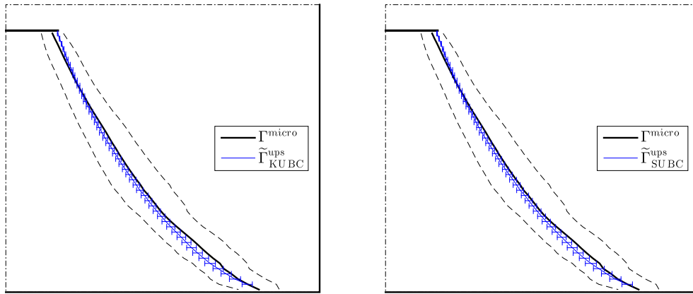
FIGURE 15 Comparison of crack paths obtained with the microscopic description (black dashed/solid lines) and the mesoscopic formulation. Left panel: case of KUBC. Right panel: case of SUBC. KUBC, kinematic uniform boundary condition; SUBC, static uniform boundary condition
