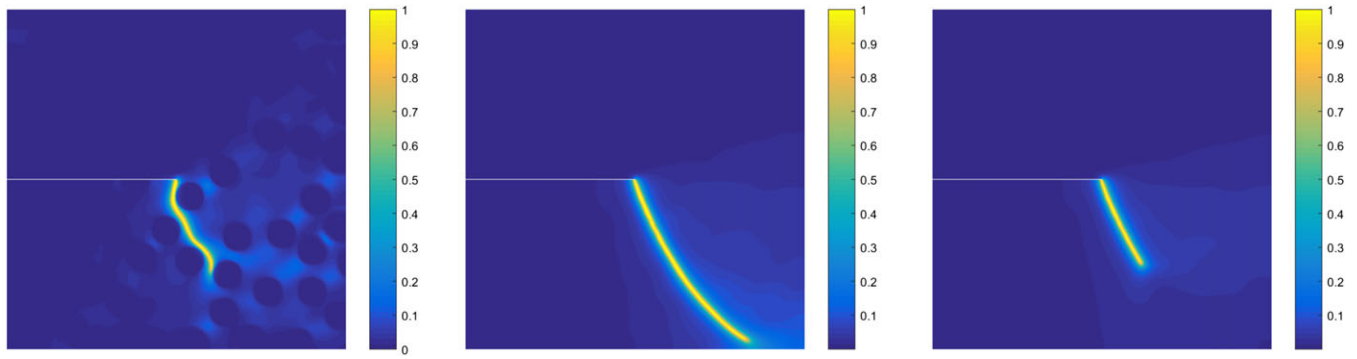
FIGURE 14 Crack path for the same microstructure: microscale description (left), KUBC-based description (middle), SUBC-based description (right). KUBC, kinematic uniform boundary condition; SUBC, static uniform boundary condition
