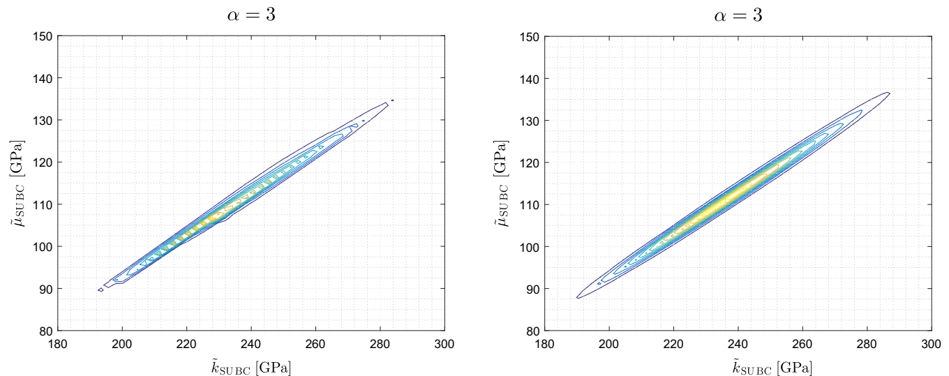
FIGURE 18 Kernel density estimates for the joint probability density function of the bulk and shear moduli, for homogenization-based (left) and model-based (right) samples (for SUBC). SUBC, static uniform boundary condition [Colour figure can be viewed at wileyonlinelibrary.com ]
