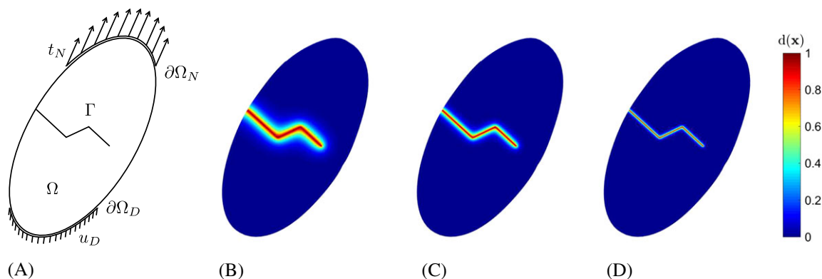
FIGURE 1 Panel (A): sharp description of a cracked solid. Panels (B), (C), and (D): smeared description within the phase field framework, showing damage profile \mathbf{x} \mapsto d(\mathbf{x}) for different values of the regularization length \ell (in this figure, L denotes the characteristic length of the domain, here of the minor axis of the ellipsoidal shape). A, no phase-field regularization; B, \ell = (1/10)L ; C, \ell = (1/20)L ; D, \ell = (1/50)L
