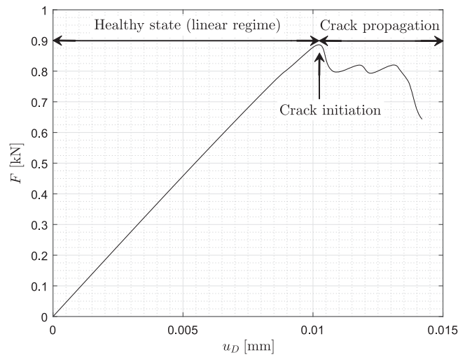
FIGURE 5 Simulated displacement-force response for the microstructure shown in the left panel in Figure 3
