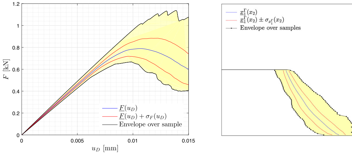
FIGURE 6 Envelope, mean, and standard deviation for the displacement-force curve (left) and the crack path (right)
