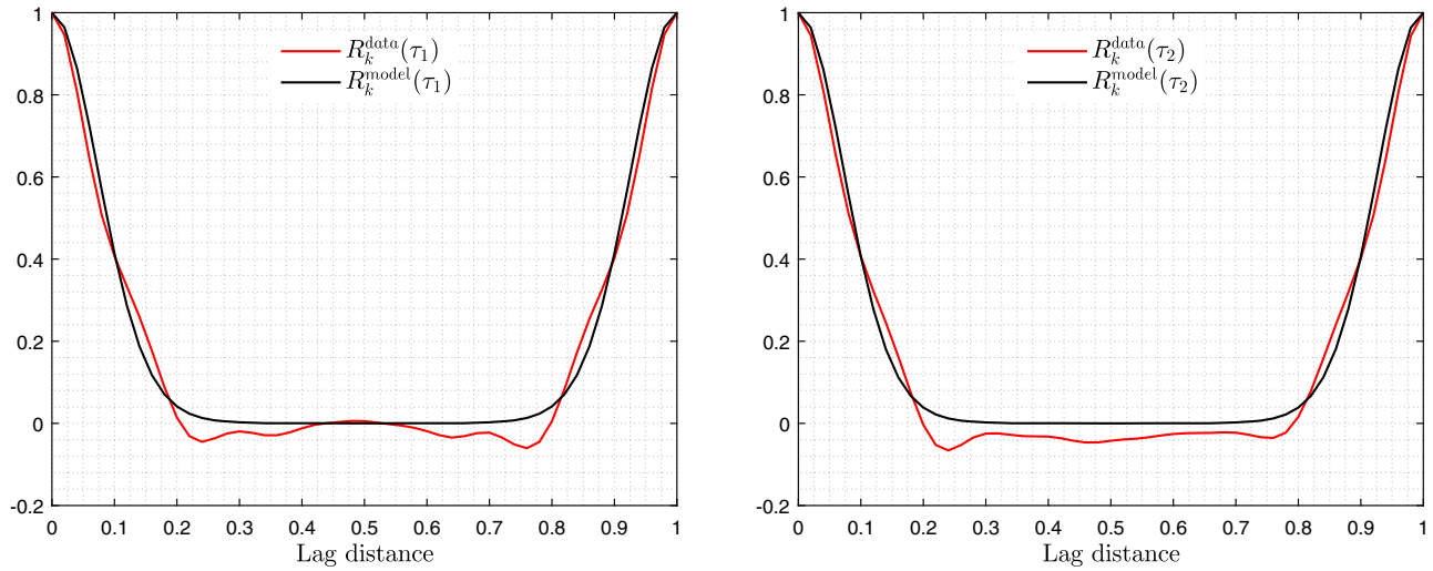
FIGURE 19 Normalized correlation function of the bulk modulus random field along \mathbf{e}^{(1)} (left) and \mathbf{e}^{(2)} (right), estimated from the multiscale data (red line) and the calibrated stochastic model (black line)
