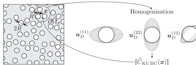
FIGURE 7 Defining mesoscale fields of stiffness through homogenization (case of kinematic uniform boundary condition)
