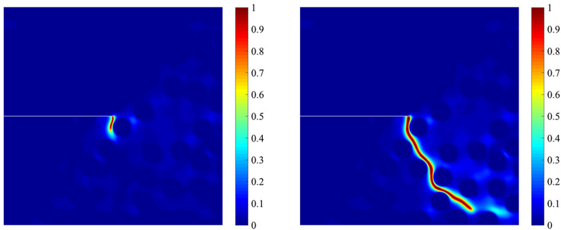
FIGURE 4 Evolution of the damage field \mathbf{x} \mapsto d(\mathbf{x}) for the microstructure shown in Figure 3
