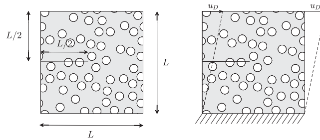
FIGURE 3 Boundary conditions applied to the domain and initial crack
