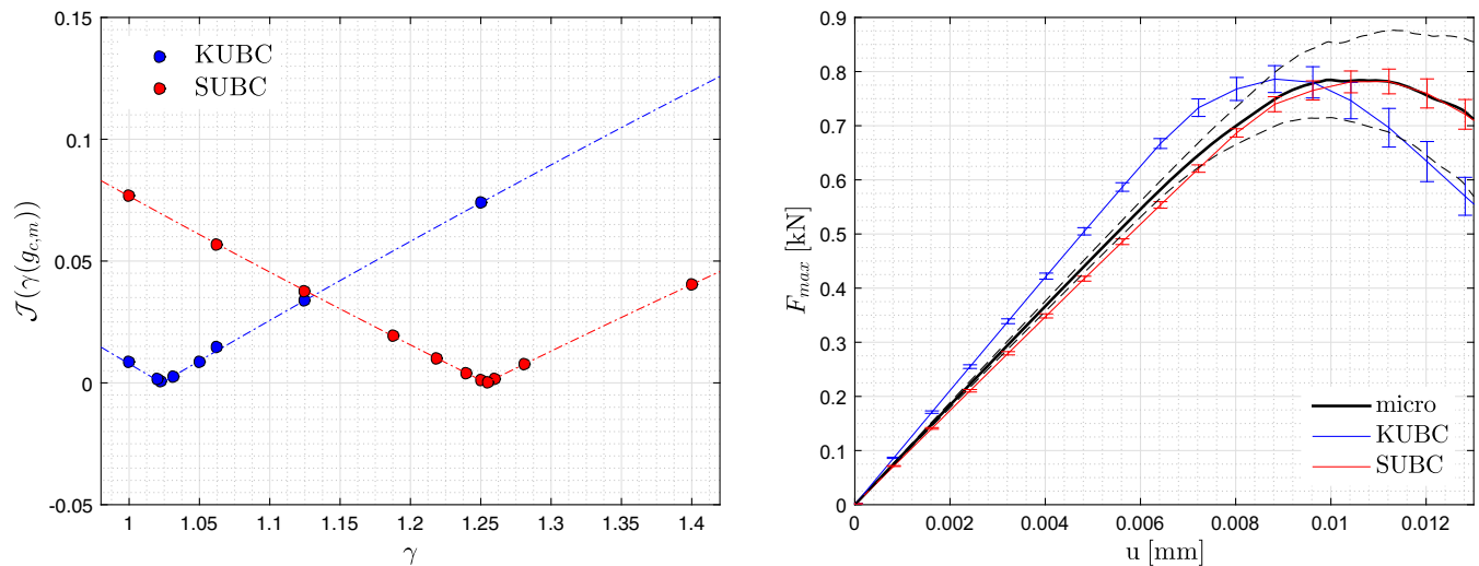
FIGURE 13 Graphs of the cost function for kinematic uniform boundary condition (KUBC) and static uniform boundary condition (SUBC) (left), and envelopes of the macroscopic response for the reference microscale model and the mesoscopic formulations (right)
