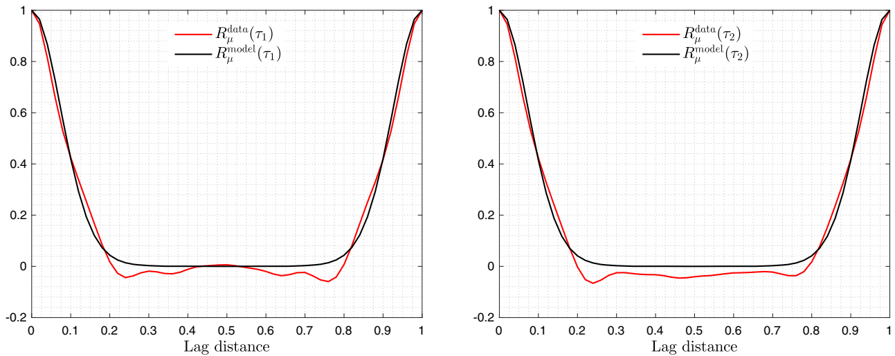
FIGURE 20 Normalized correlation function of the shear modulus random field along \mathbf{e}^{(1)} (left) and \mathbf{e}^{(2)} (right), estimated from the multiscale data (red line) and the calibrated stochastic model (black line)
