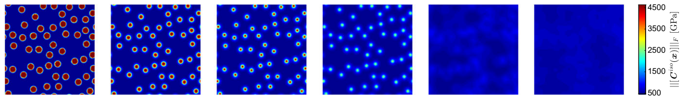
FIGURE 10 One realization of the random field \{|||C^{iso}(x)|||_F, x \in \Omega\} for \tilde{R}/R \in \{0.2, 0.6, 0.8, 1, 2, 4\} (from left to right)
