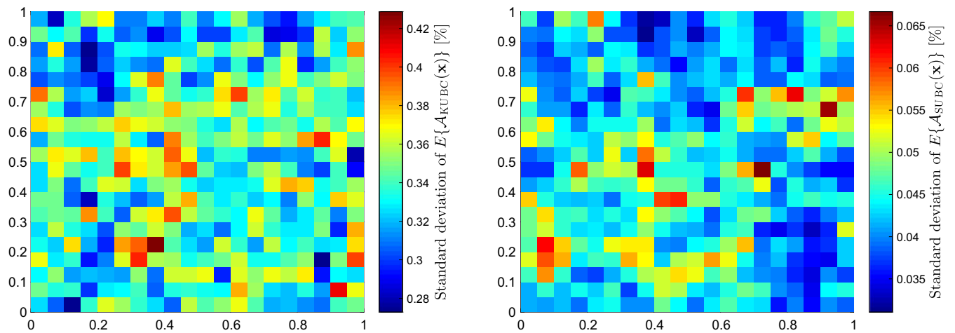
FIGURE 9 Graphs of the fields of standard deviation for the random fields \{A_{KUBC}(x), x \in \Omega\} (left) and \{A_{SUBC}(x), x \in \Omega\} (right). KUBC, kinematic uniform boundary condition; SUBC, static uniform boundary condition
