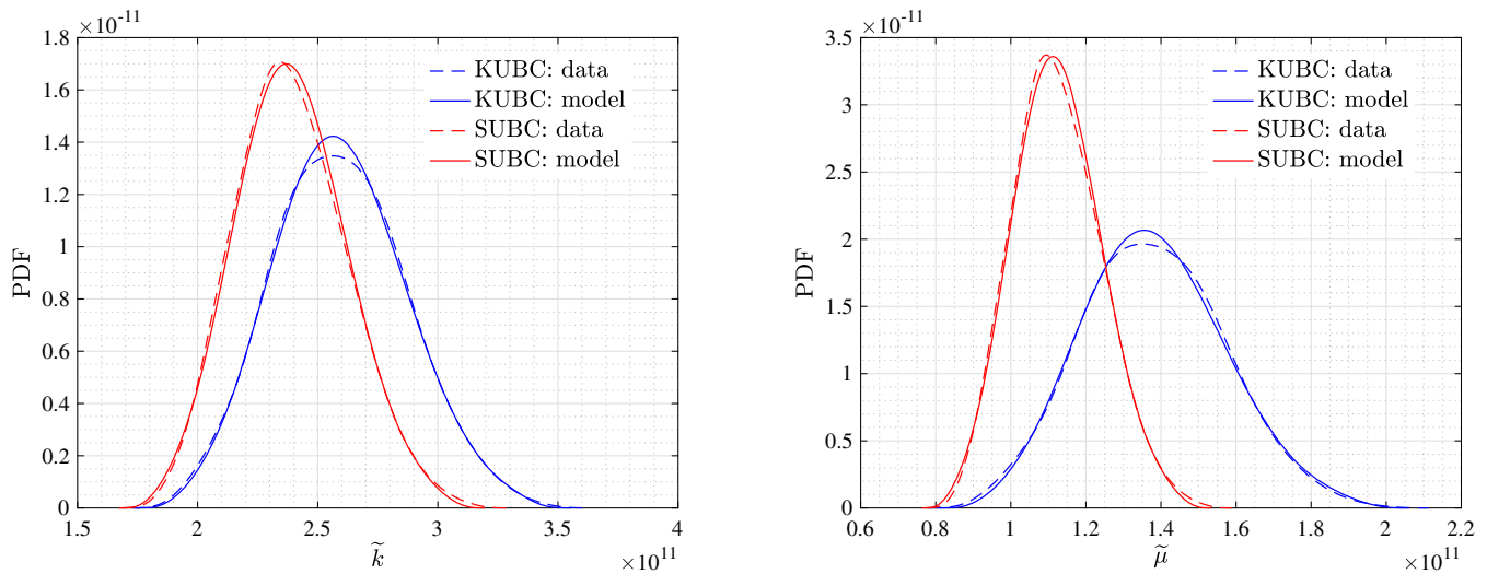
FIGURE 17 Kernel density estimates for the probability density function of the bulk (left) and shear (right) moduli, for the two types of boundary conditions kinematic uniform boundary condition (KUBC) (blue) and static uniform boundary condition (SUBC) (red)
