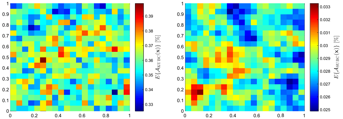
FIGURE 8 Graphs of the mean functions for the random fields \{A_{KUBC}(x), x \in \Omega\} (left) and \{A_{SUBC}(x), x \in \Omega\} (right). KUBC, kinematic uniform boundary condition; SUBC, static uniform boundary condition
