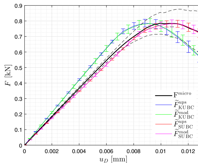
FIGURE 22 Envelopes of the macroscopic response for the reference microscale model ( F ) and the mesoscopic formulations parametrized either by upscaled coefficients ( \tilde{F}_{\text{KUBC}}^{\text{ups}} , \tilde{F}_{\text{SUBC}}^{\text{ups}} ) or model-based coefficients ( \tilde{F}_{\text{KUBC}}^{\text{mod}} , \tilde{F}_{\text{SUBC}}^{\text{mod}} )
