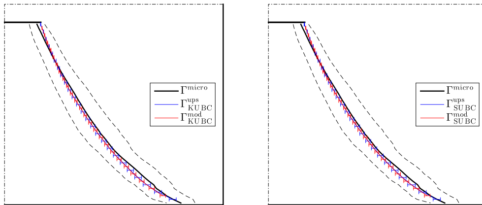
FIGURE 21 Comparison of crack paths obtained with the microscopic description (black dashed/solid lines), the mesoscopic formulation where the elasticity is obtained from microstructural samples (blue lines), and the mesoscopic formulation involving the stochastic model for elasticity tensors (red lines). Left panel: case of KUBC. Right panel: case of SUBC. KUBC, kinematic uniform boundary condition; SUBC, static uniform boundary condition
