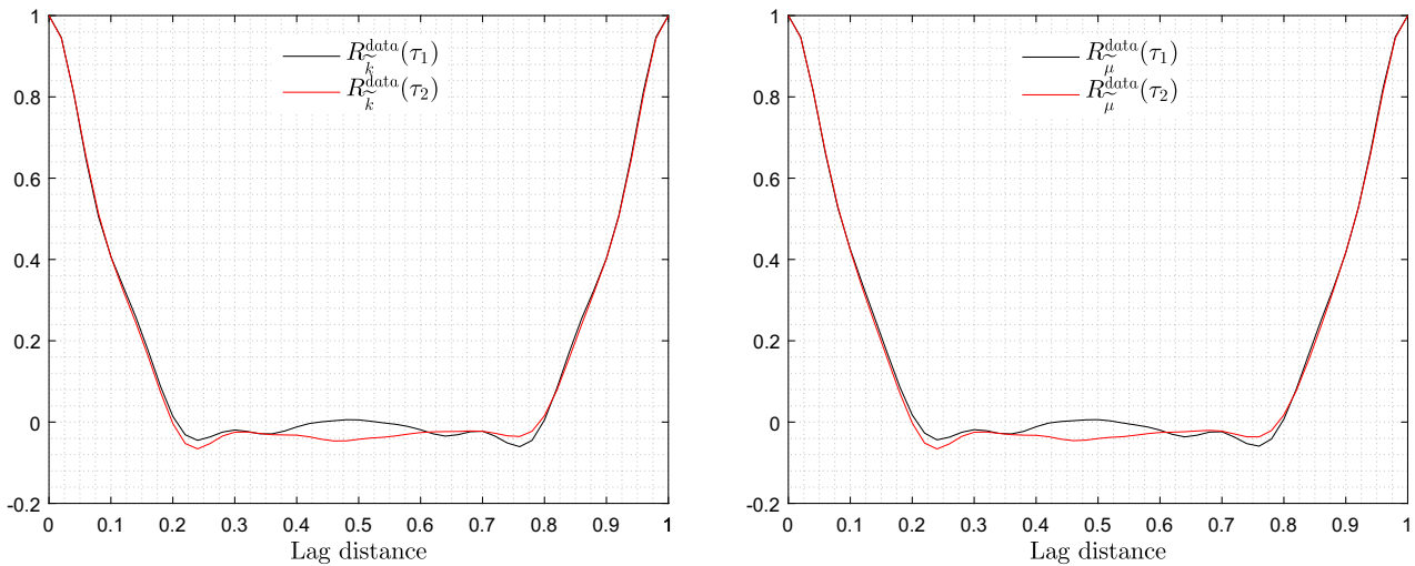
FIGURE 12 Graph of the correlation function along \mathbf{e}^{(1)} and \mathbf{e}^{(2)} , estimated from the simulated data, for the random fields of bulk (left) and shear (right) moduli
